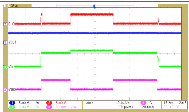
图 14. TS Entering and Leaving Cold Temperature
