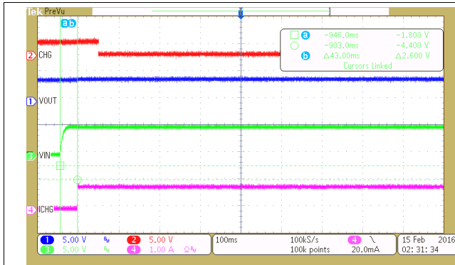
图 11. Power-Up Timing
