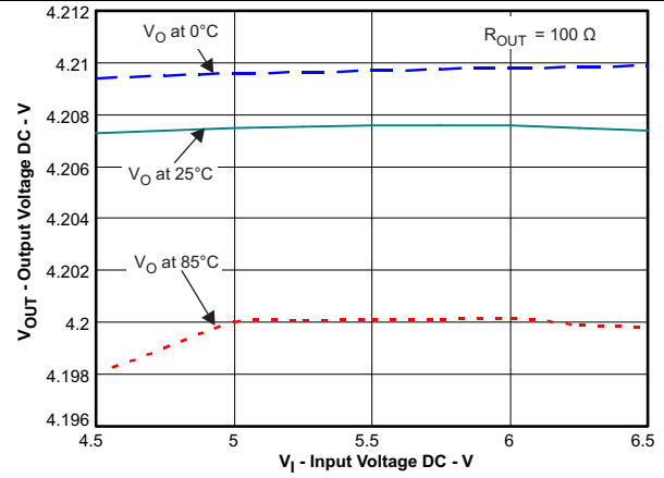
图 2. Line Regulation
