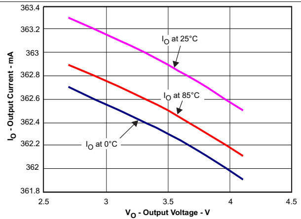
图 4. Current Regulation Over Temperature
