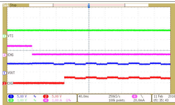
图 19. Battery Removal - GND Removed 1st, 42- \Omega Load
