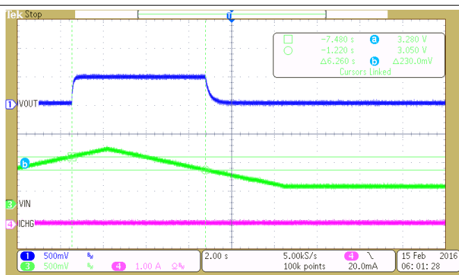
图 26. DPM – USB Current Limits – VIN Regulated to 4.4 V
