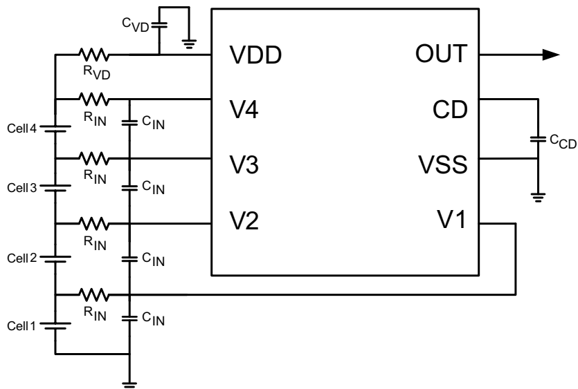
图 9-1. Application Configuration
