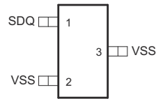
图 5-1. DBZ Package 3-Pin SOT-23 (Top View)
