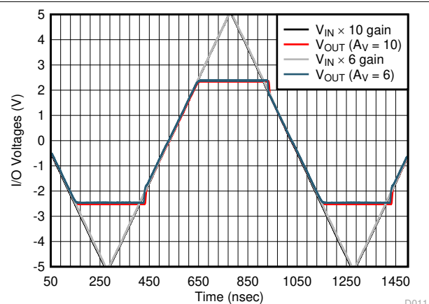
图 7-9. Simulated Noninverting Settling Time
