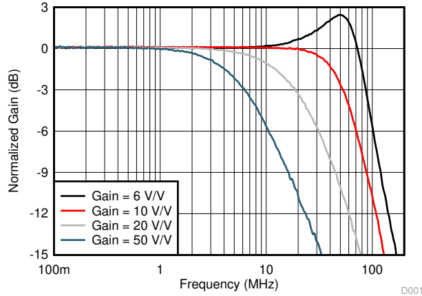
图 7-1. Noninverting Small-Signal Frequency Response vs Gain
