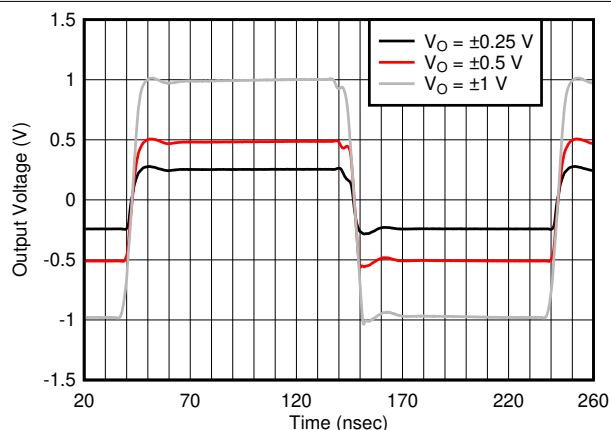
图 7-26. Inverting Step Response vs V_{OPP}
