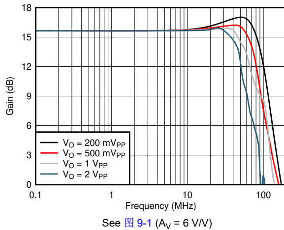
图 7-21. Noninverting Large-Signal Bandwidth vs V_{OPP}
