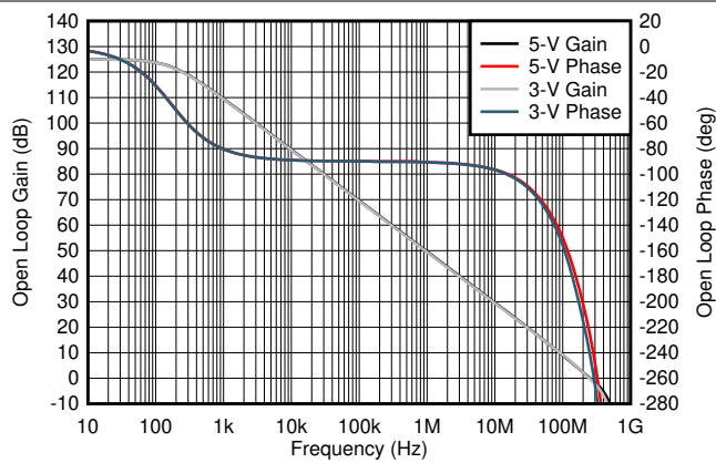
图 7-37. Open-Loop Gain and Phase
