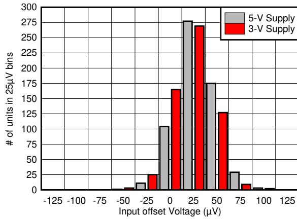
图 7-43. Input Offset Voltage Distribution
