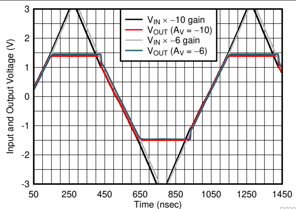
图 7-28. Inverting Settling Time
