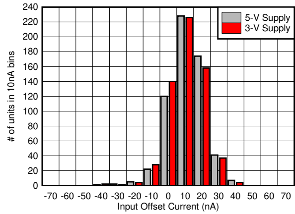
图 7-44. Input Offset Current Distribution
