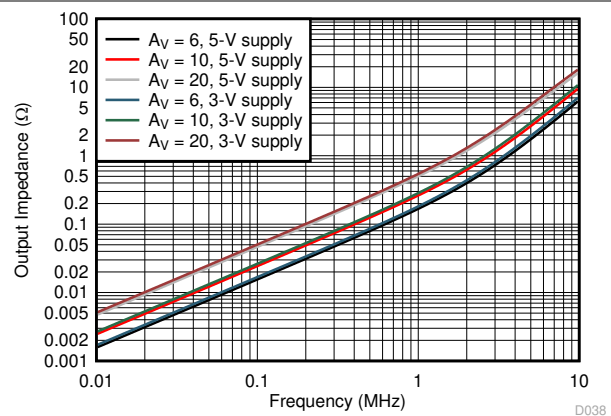
图 7-38. Closed-Loop Output Impedance
