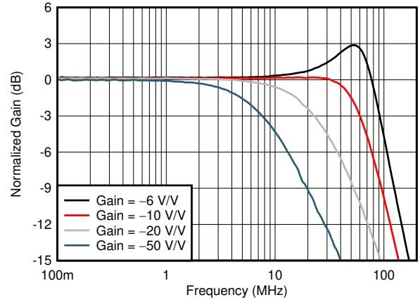
图 7-2. Inverting Small-Signal Frequency Response vs Gain
