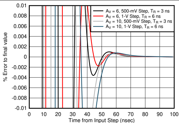
图 7-25. Noninverting Step Response vs V_{OPP}
