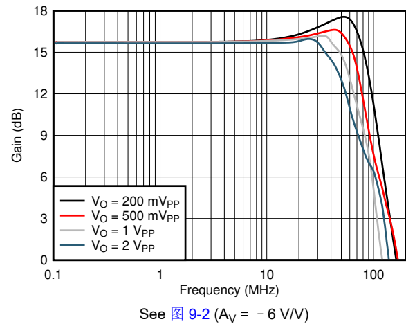
图 7-22. Inverting Large-Signal Bandwidth vs V_{OPP}
