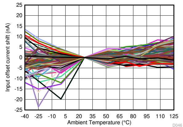
图 7-44. Input Offset Current Distribution
