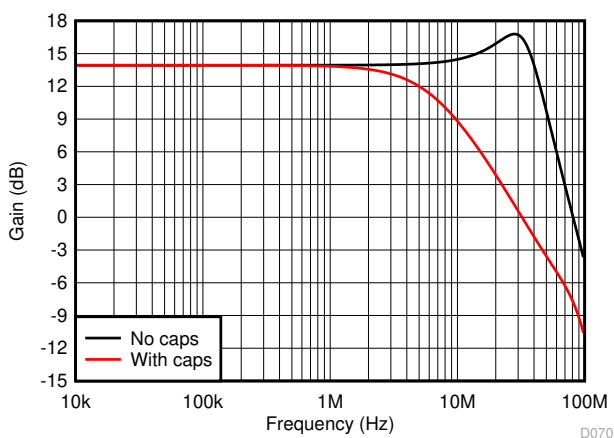
图 8-5. Inverting Response With and Without Compensation
