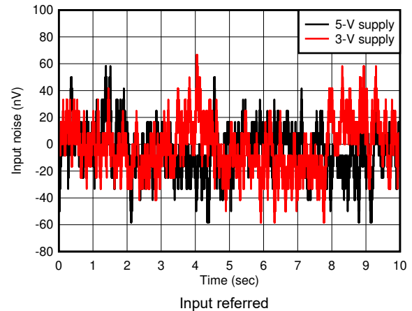
图 7-40. Low-Frequency Voltage Noise
