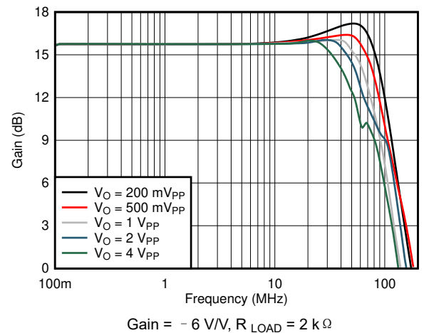
图 7-4. Inverting Large-Signal Bandwidth vs V_{OPP}
