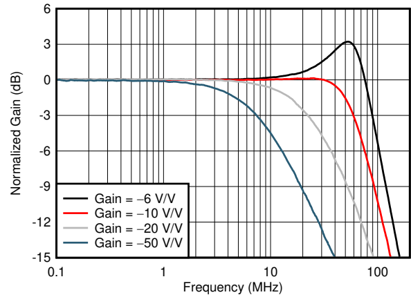
图 7-20. Inverting Small-Signal Response vs Gain
