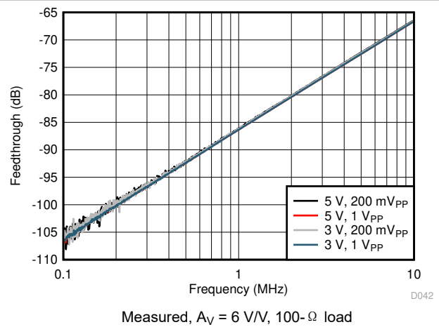
图 7-42. Disabled Isolation Noninverting Input to Output
