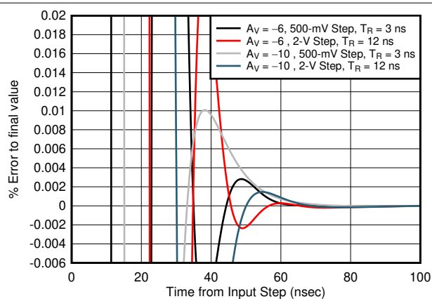
图 7-8. Inverting Step Response vs V_{OPP}
