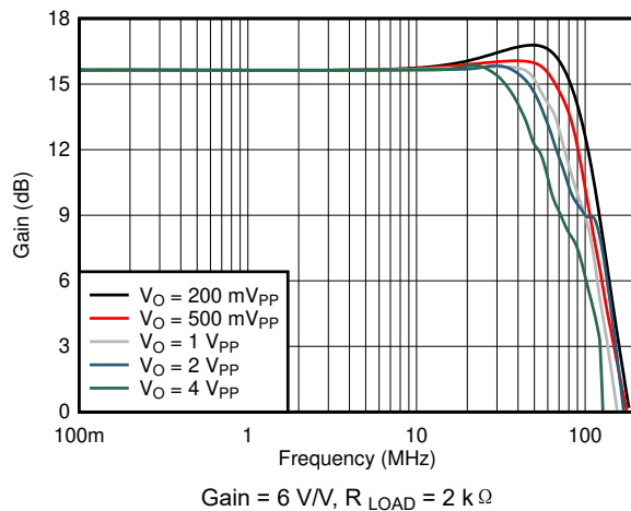
图 7-3. Noninverting Large-Signal Bandwidth vs V_{OPP}
