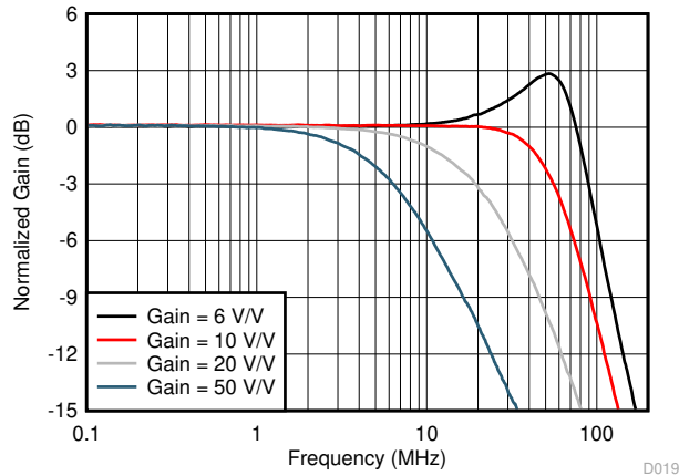
图 7-19. Noninverting Small-Signal Response vs Gain
