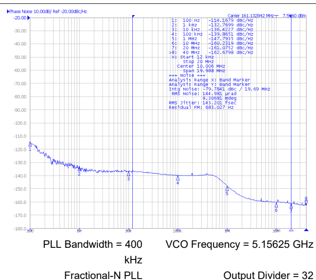
图 6-4. Closed-Loop Phase Noise of LVPECL Differential Output at 161.1328125 MHz
