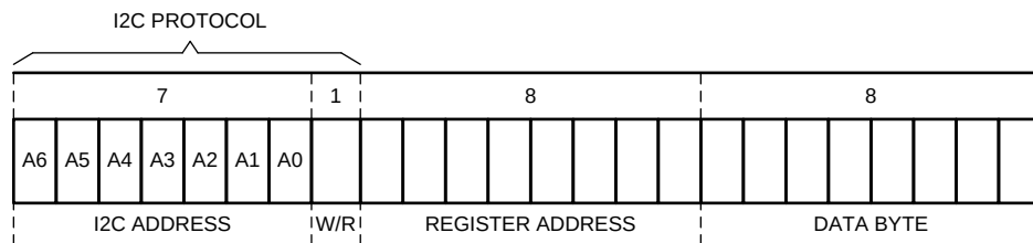
Figure 28. I 2 C Register Structure
