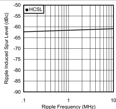
图 6-8. PSRR vs Ripple Frequency at 312.5 MHz
