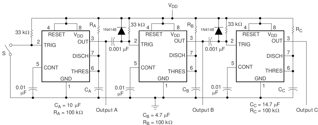
图 7-8. Sequential Timer Circuit
