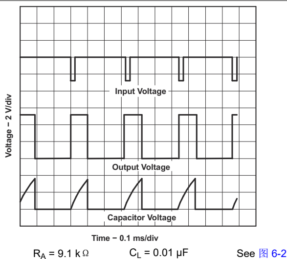
图 6-3. Typical Monostable Waveforms
