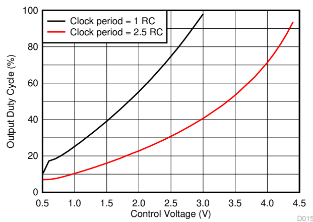
图 7-4. Pulse-Width-Modulation vs Control Voltage Clock Duty Cycle 98%, V_{DD} = 5\text{ V}
