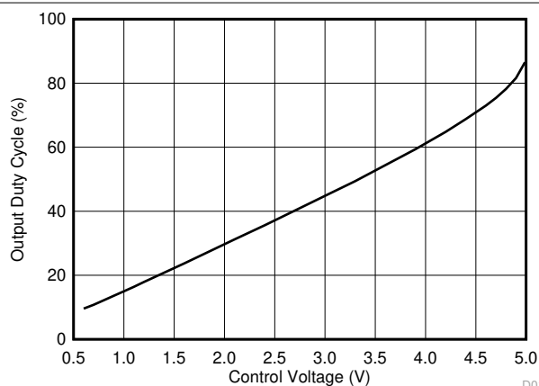
图 7-7. Pulse-Position-Modulation Duty Cycle vs Control Voltage, V_{DD} = 5 \text{ V}
