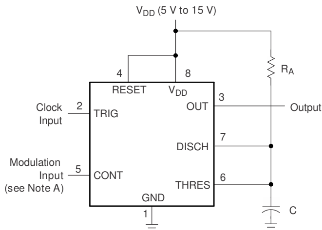
图 7-3. Circuit for Pulse-Width Modulation
