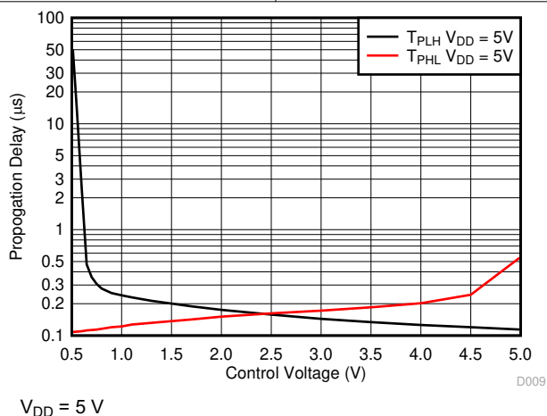
图 5-9. Propagation Delay vs Control Voltage
