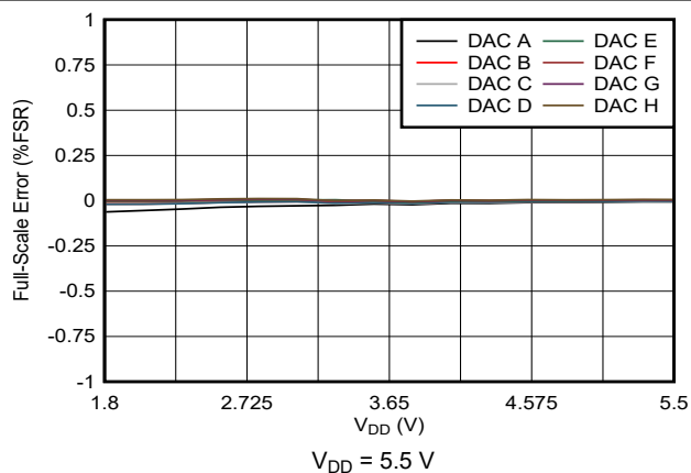
图 5-34. Full-Scale Error vs Supply Voltage
