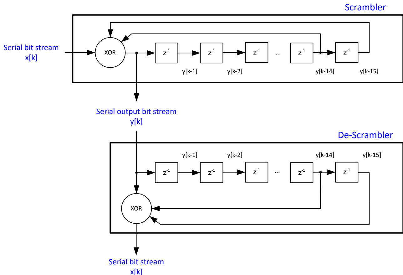
图 7-38. Output scrambler and descrambler operation
