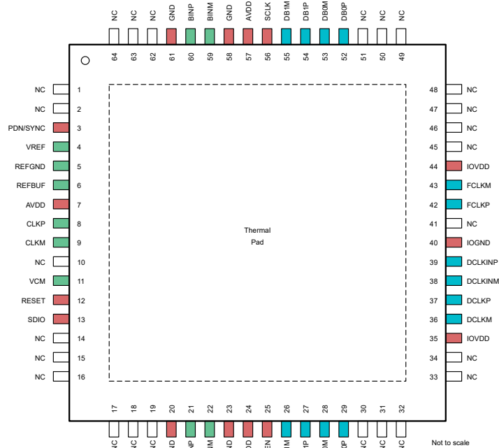
图 4-1. HBP Package, 64-Pin CFP (Top View)
