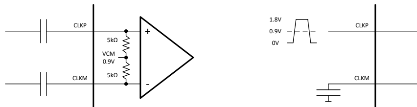
图 7-12. External and internal connection using differential (left) and single ended (right) clock input
