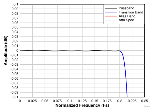
图 7-24. Decimation by 2 Complex Passband Ripple Response
