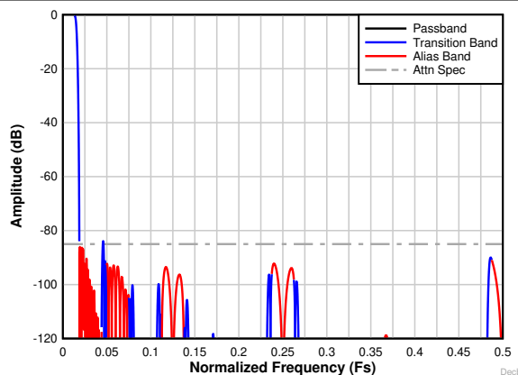
图 7-31. Decimation by 32 Complex Frequency Response
