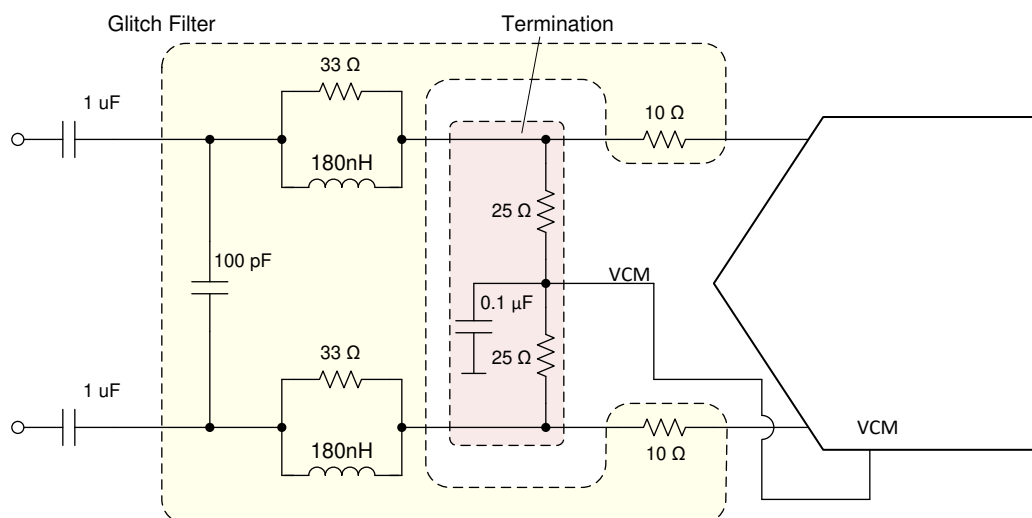
图 7-4. AC-Coupling: Termination Network Provides DC Bias (Glitch Filter Example for DC to 30MHz)
