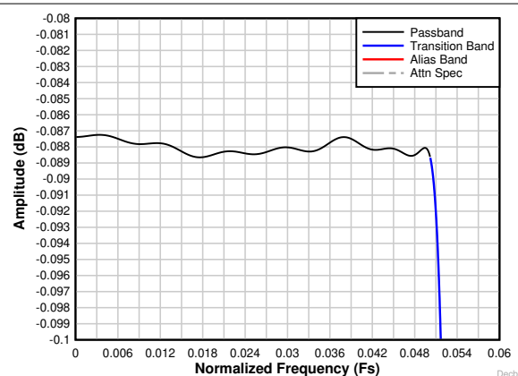
图 7-28. Decimation by 8 Complex Passband Ripple Response
