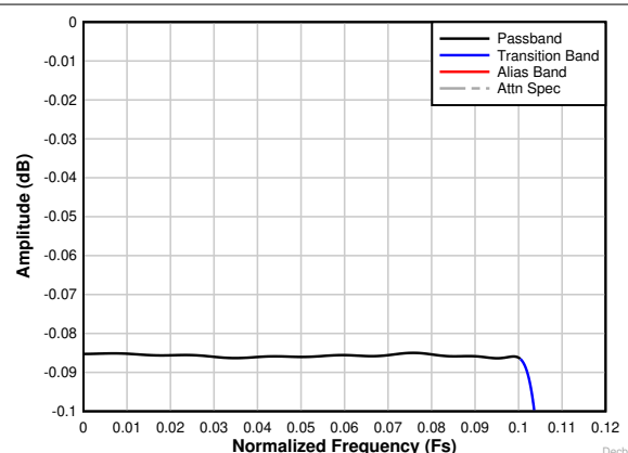
图 7-26. Decimation by 4 Complex Passband Ripple Response
