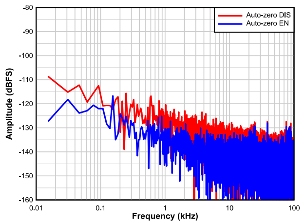
图 7-9. FFT at 65MSPS with Input Frequency of 5MHz (Auto-Zero Feature Enable vs Disable, 4M Point FFT) zoomed in near DC
