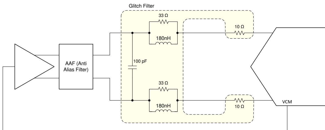
图 7-5. DC-Coupling: DC bias provided by FDA (glitch filter example for DC to 30MHz)
