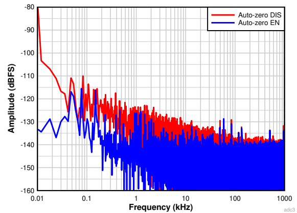
图 7-7. FFT at 2 MSPS with Input Frequency of 3MHz (Auto-Zero Feature Enable vs Disable, 4M Point FFT) zoomed in near DC
