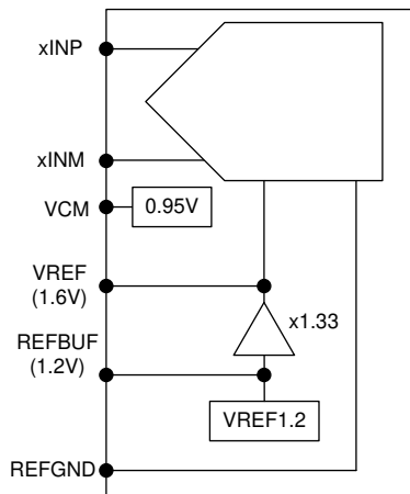
图 7-13. Different Voltage Reference Options for ADC3683-SP
