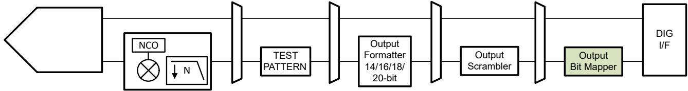
图 7-39. Output Bit Mapper
