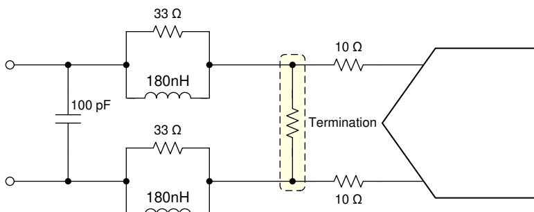
图 7-2. Sampling Glitch Filter Example for Input Frequencies From DC to 30MHz
