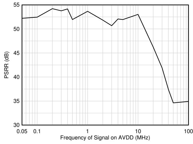
图 8-7. Power Supply Rejection Ratio (PSRR) vs Frequency
