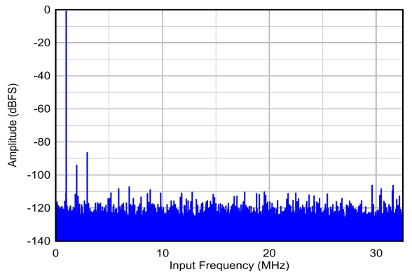
图 5-1. Single Tone FFT at F_{IN} = 1\text{MHz}
