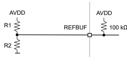
图 7-47. Configuration of external voltage on REFBUF pin
