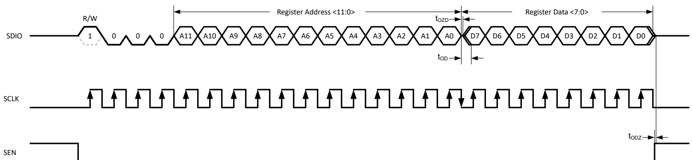
图 7-49. Serial Register Read Timing Diagram
