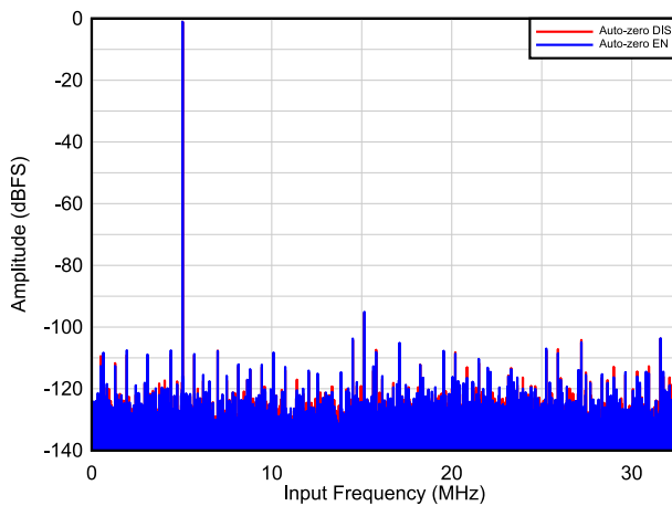
图 7-8. FFT at 65MSPS with Input Frequency of 5MHz (Auto-Zero Feature Enable vs Disable, 4M Point FFT)
