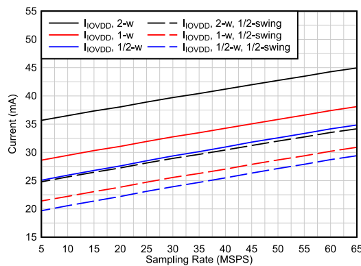
图 5-3. Current vs Sampling Rate
