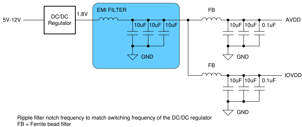
图 8-9. Example Switcher-Only Approach
