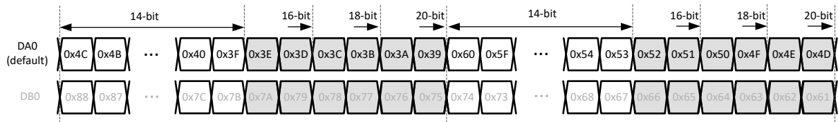
图 7-43. 1/2-wire output bit mapping
