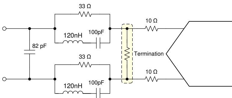
图 7-3. Sampling Glitch Filter Example for Input Frequencies From 30 to 70MHz
