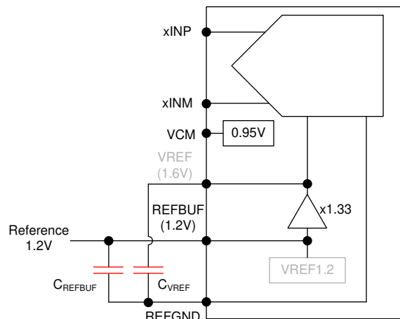
图 7-16. External 1.2V Reference Using Internal Reference Buffer
