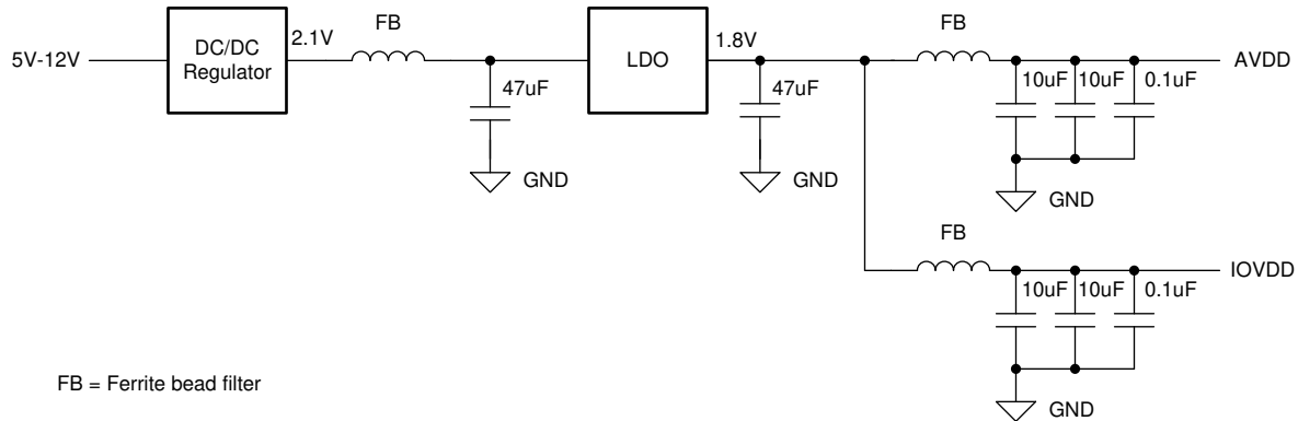
图 8-8. Example: LDO Linear Regulator Approach
