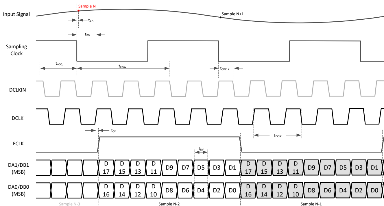
图 6-1. Timing diagram: 2-wire SLVDS
