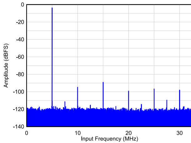
图 8-2. Single Tone FFT at F_{IN} = 5\text{MHz}
