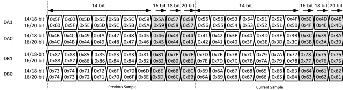
图 7-40. 2-wire output bit mapper
