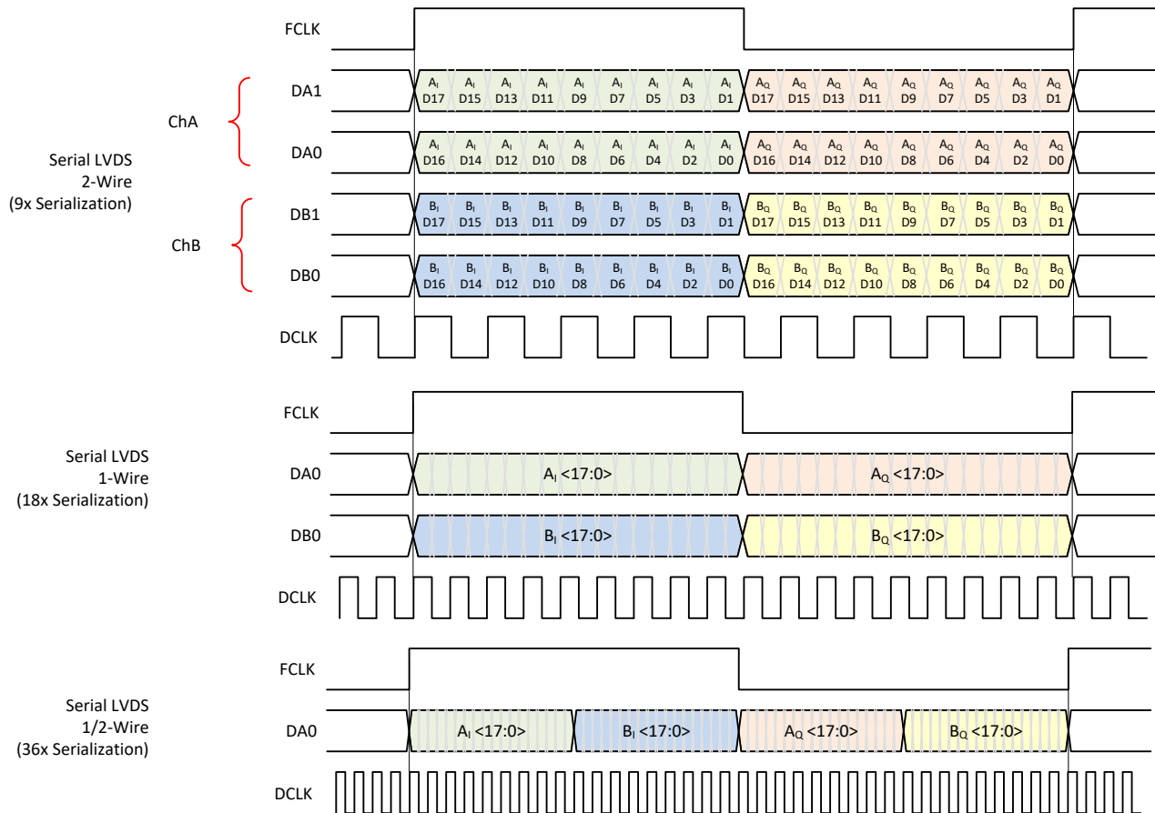
图 7-34. Output Data Format in Complex Decimation (18-bit Output Resolution)
