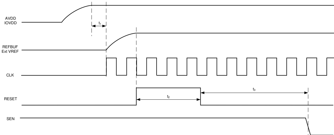
图 8-6. Initialization of serial registers after power up
