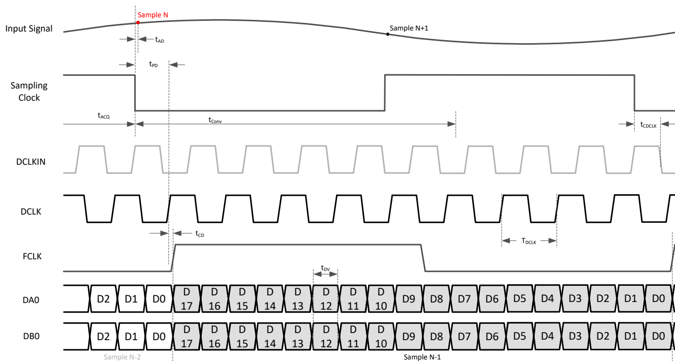
图 6-2. Timing diagram: 1-wire SLVDS
