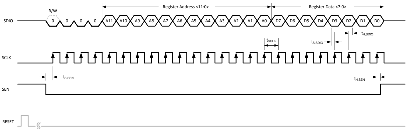
图 7-48. Serial Register Write Timing Diagram
