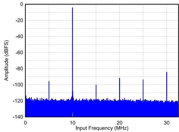
图 8-3. Single Tone FFT at F_{IN} = 10\text{MHz}
