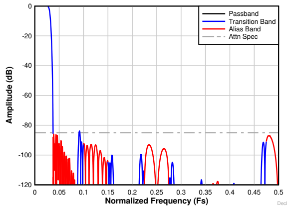
图 7-29. Decimation by 16 Complex Frequency Response
