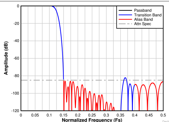
图 7-25. Decimation by 4 Complex Frequency Response
