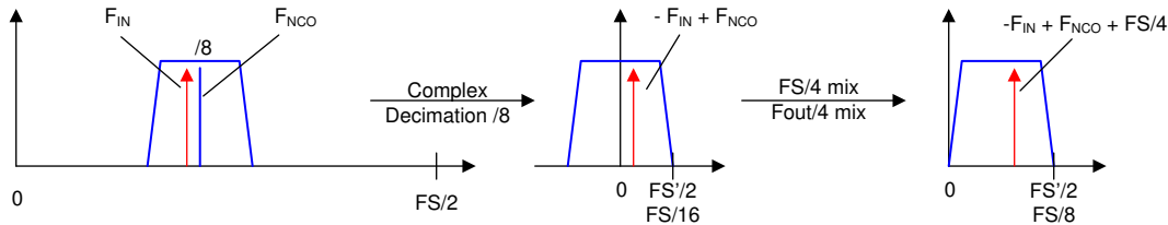
图 7-21. FS/4 Mixing with Real Output
