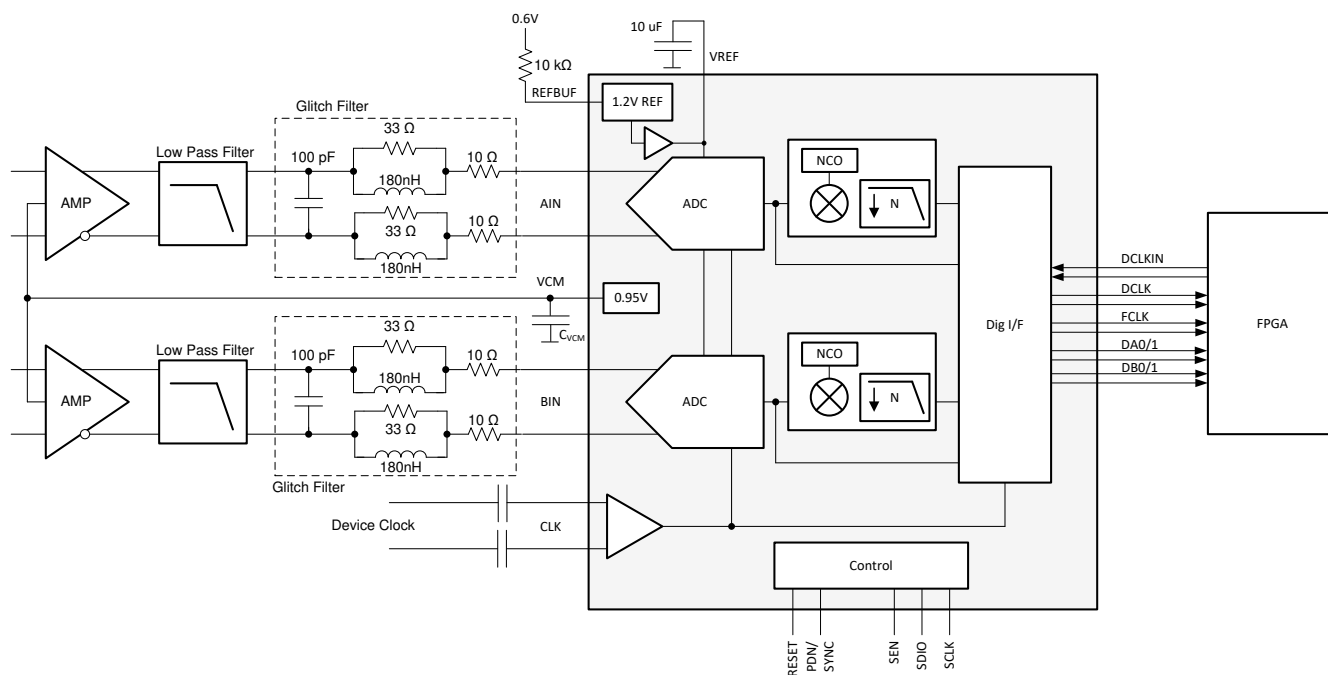
图 8-1. Typical Configuration for a Spectrum Analyzer with DC Support
