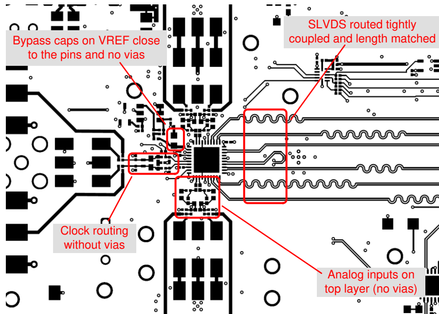
图 8-10. Layout example: top layer of ADC3683EVM
