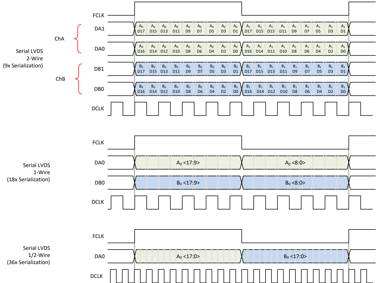
图 7-35. Output Data Format in Real Decimation (18-bit Output Resolution)
