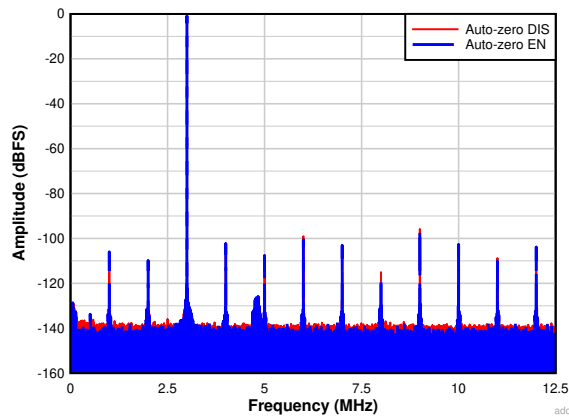
图 7-6. FFT at 25MSPS with Input Frequency of 3MHz (Auto-Zero Feature Enable vs Disable, 4M Point FFT)
