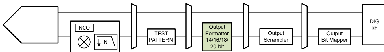
图 7-36. Interface Output Bit Mapper
