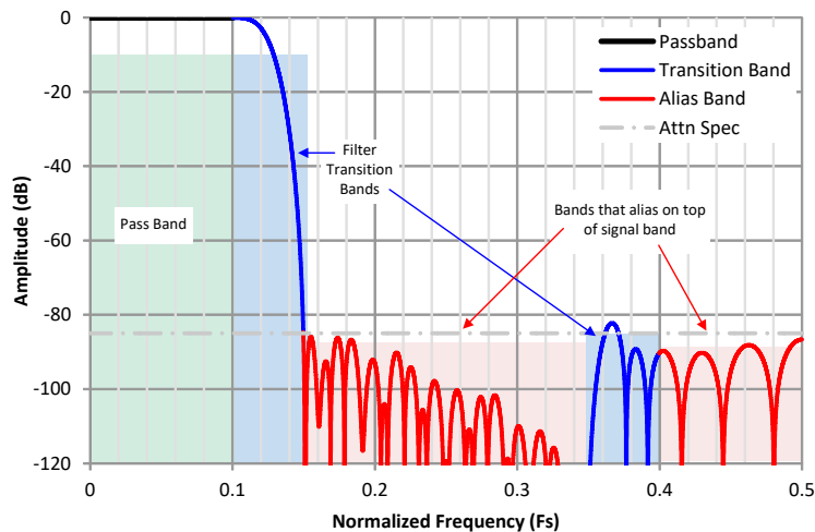
图 7-22. Interpretation of the Decimation Filter Plots
