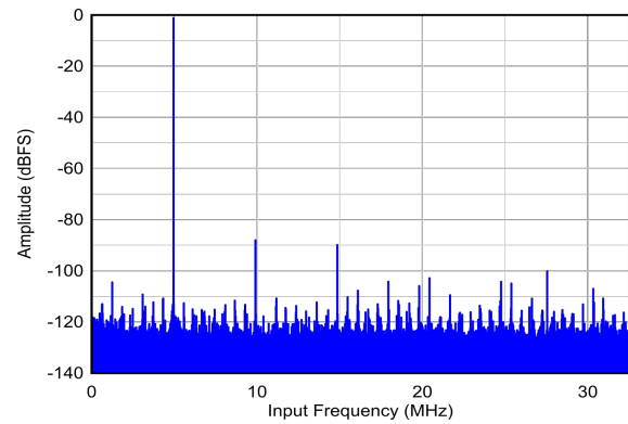
图 5-2. Single Tone FFT at F_{IN} = 5\text{MHz}
