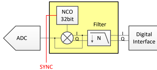
图 7-17. Internal Digital Decimation Filter
