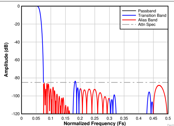
图 7-27. Decimation by 8 Complex Frequency Response
