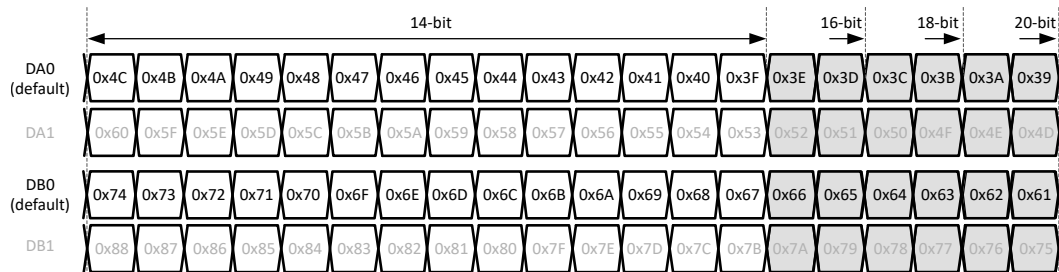
图 7-42. 1-wire output bit mapping
