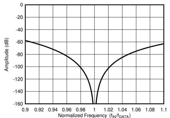
图 7-22. Detail Sinc3 Frequency Response (OSR = 32000)
