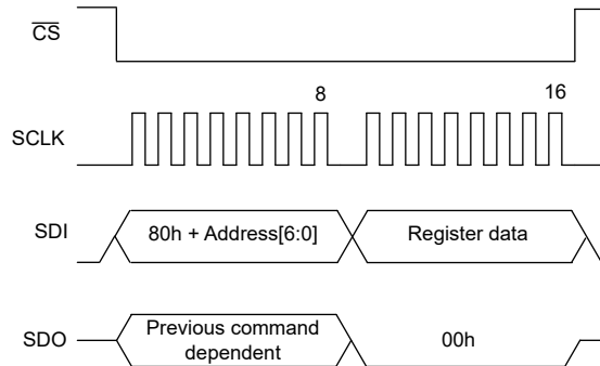
图 7-46. Write Register Data (STATUS and CRC Disabled)
