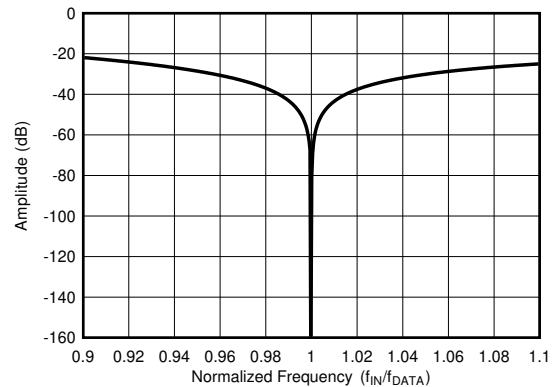
图 7-24. Detail Sinc3 + Sinc1 Frequency Response
