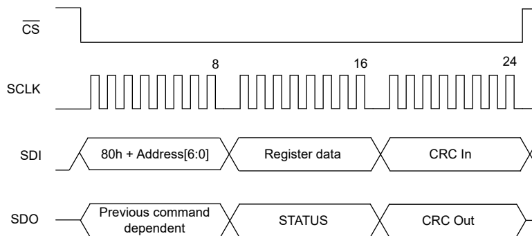
图 7-47. Write Register Data (STATUS and CRC Enabled)
