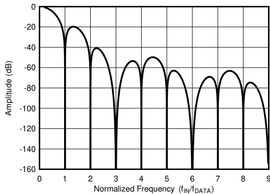
图 7-23. Sinc3 + Sinc1 Frequency Response
