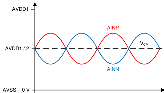
图 7-1. Unipolar Differential Input Signal
