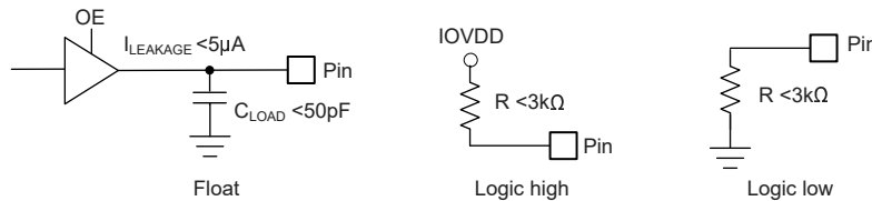
图 7-42. Hardware Programming Pin Conditions
