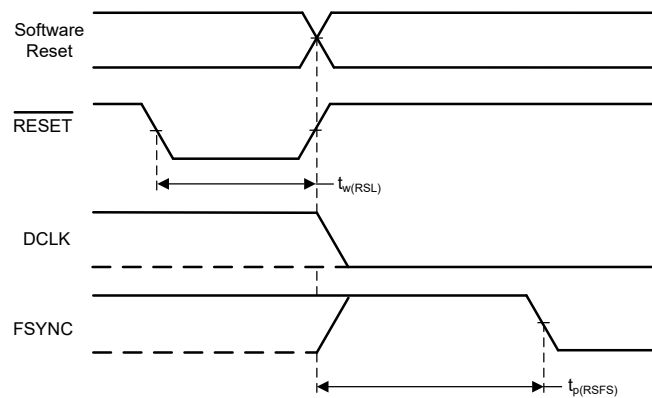
图 5-6. RESET Pin Timing Requirements and Switching Characteristic
