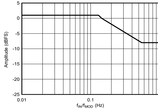
图 7-11. Amplitude Limit to Avoid Modulator Saturation
