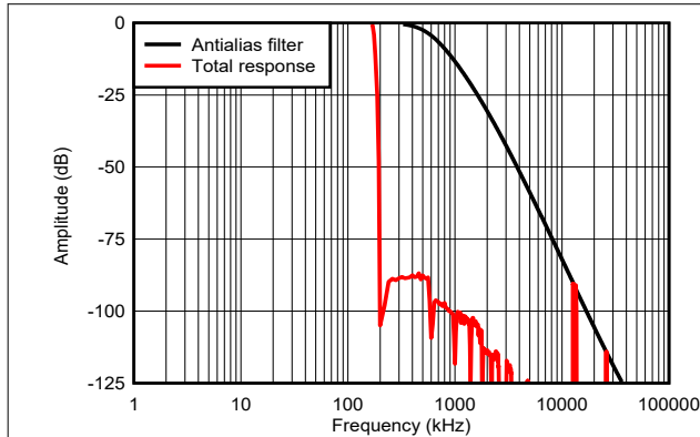
图 9-2. Antialias Filter Frequency Response
