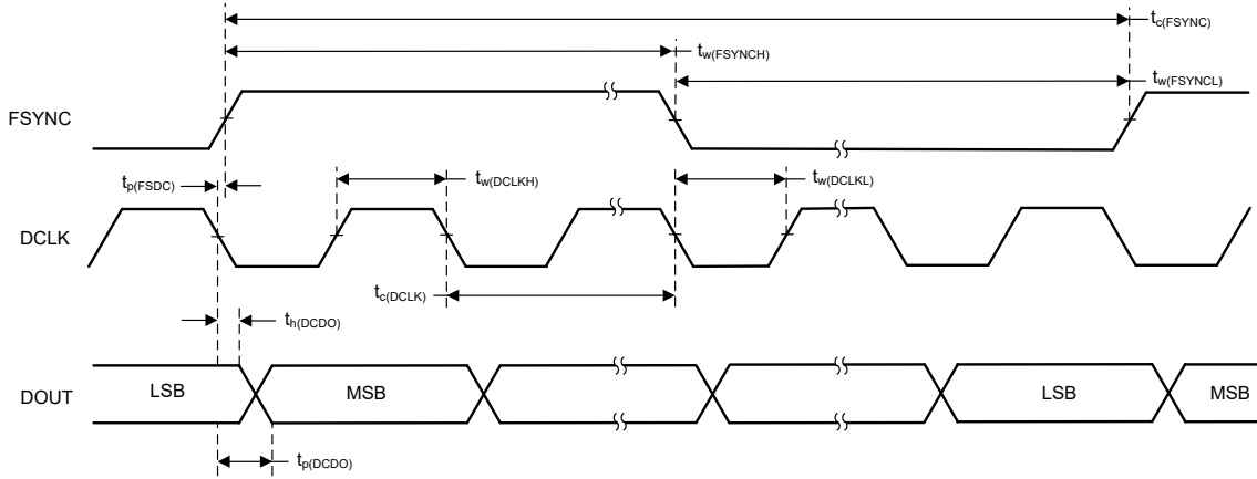
图 5-2. Frame-Sync Data Port Switching Characteristics
