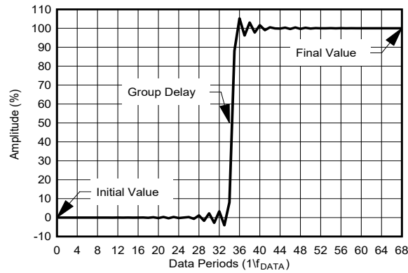
图 7-17. Wideband Filter Step Response
