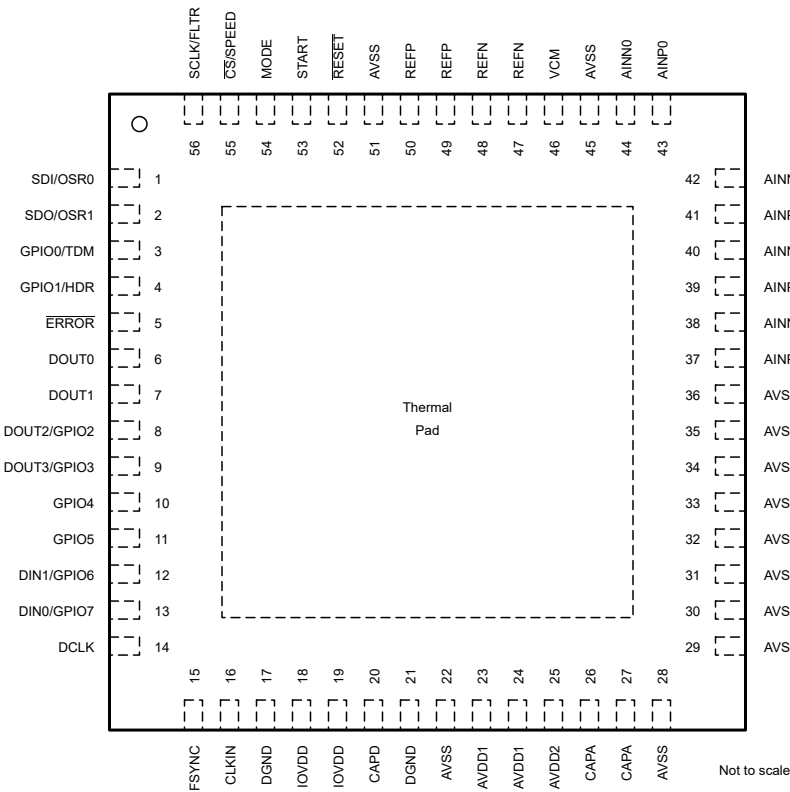
图 4-1. ADS127L14 RSH Package, 56-Pin VQFN (Top View)
