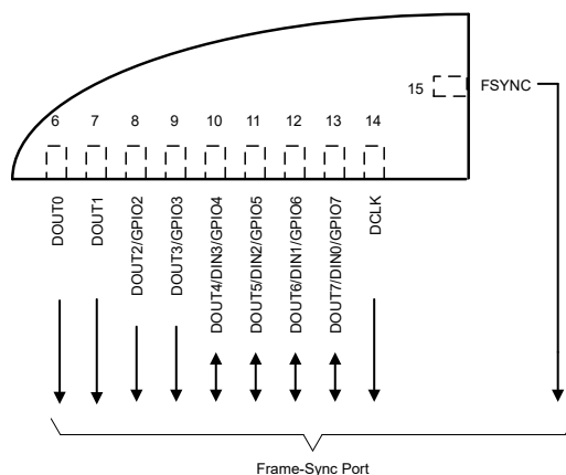
图 7-30. ADS127L18 Frame-Sync Port Pins
