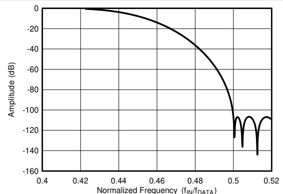
图 7-13. Wideband Filter Transition Band
