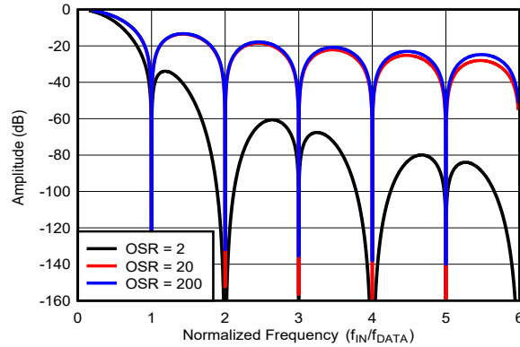
图 7-20. Sinc4 + Sinc1 Frequency Response
