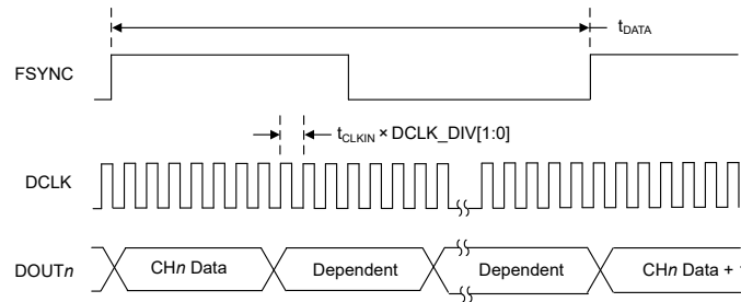
图 7-31. Frame-Sync Port Operation
