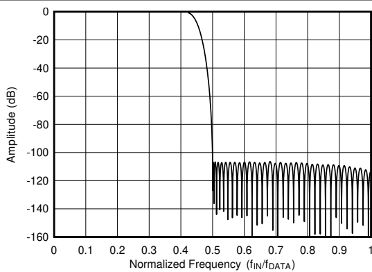
图 7-14. Wideband Filter Frequency Response
