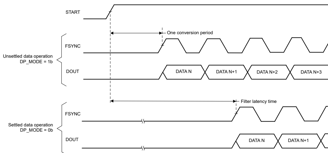
图 7-27. Settled and Unsettled Data Modes
