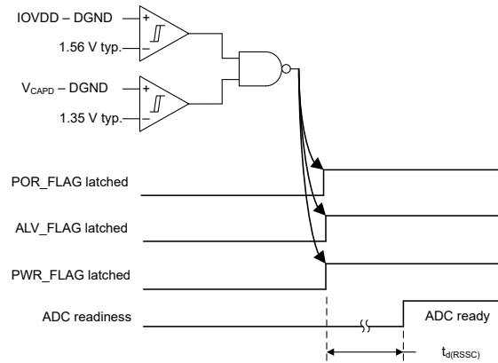
图 7-7. Digital Supply Threshold
