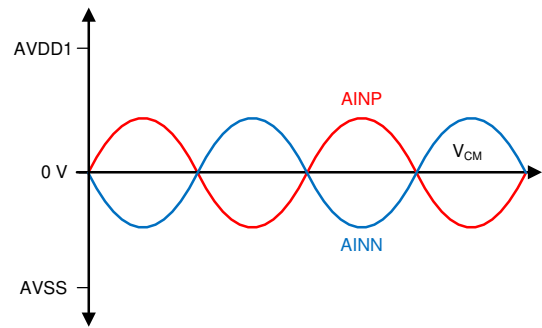
图 7-2. Bipolar Differential Input Signal
