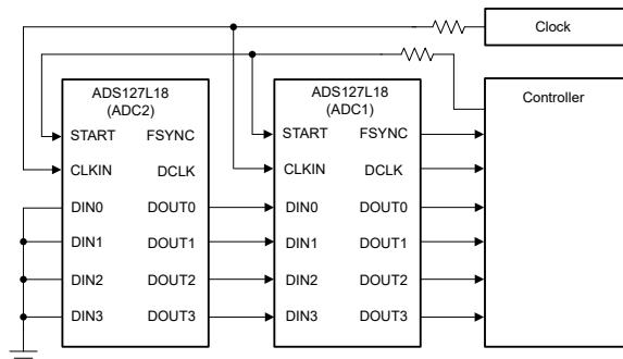
图 7-36. Daisy-Chain Connection in TDM Mode (DP_TDM = 01b)
