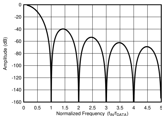
图 7-21. Sinc3 Frequency Response (OSR = 32000)
