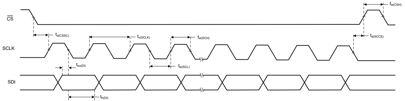
图 5-3. SPI Serial Timing Requirements
