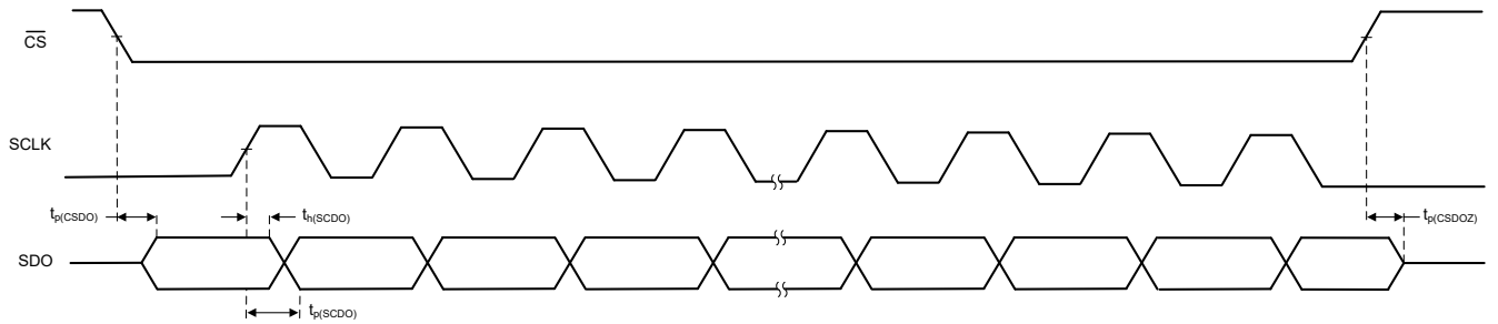
图 5-4. SPI Switching Characteristics
