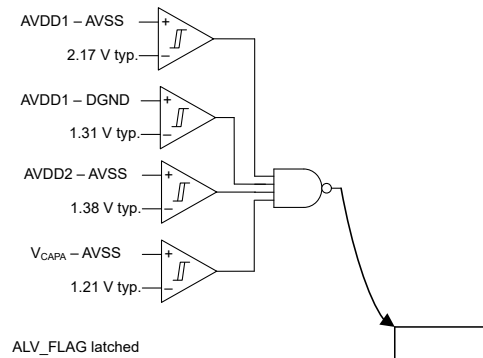
图 7-8. Analog Supply Threshold
