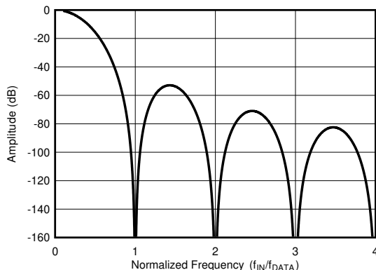
图 7-18. Sinc4 Frequency Response (OSR = 32)
