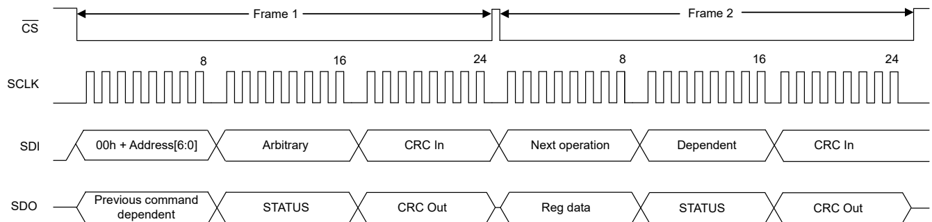
图 7-45. Read Register Data (STATUS and CRC Enabled)
