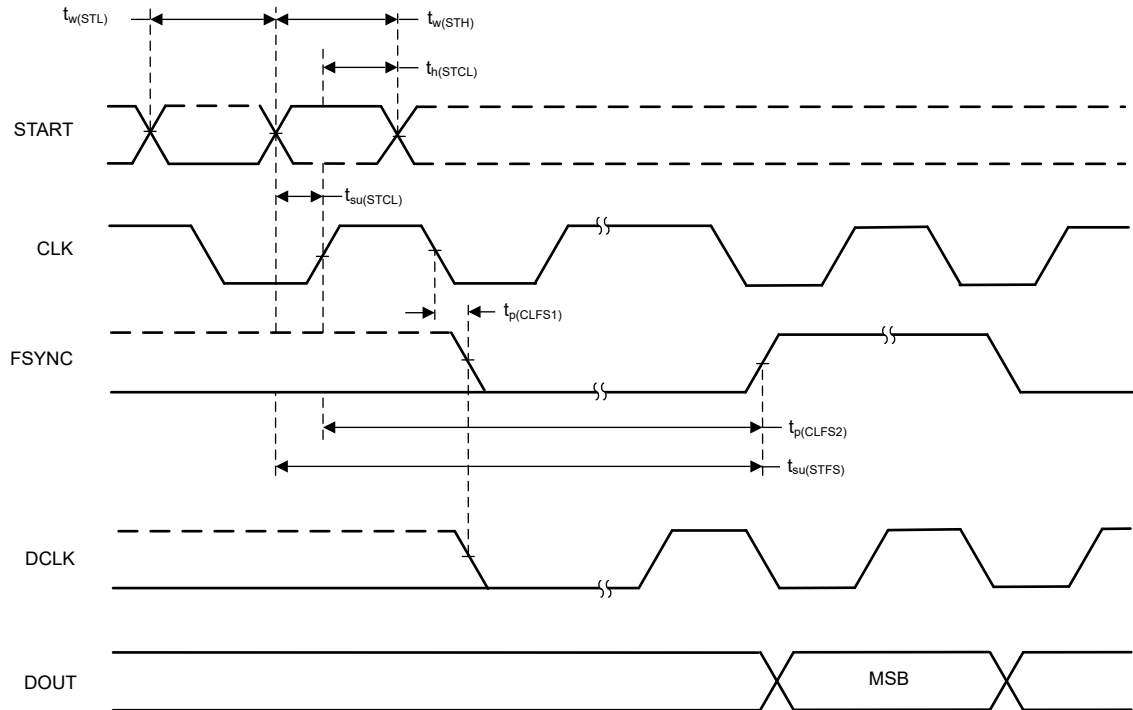
图 5-5. START Pin Timing Requirements and Switching Characteristics
