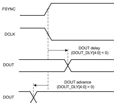
图 7-40. DOUT Offset Timing
