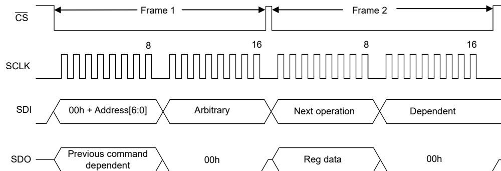
图 7-44. Read Register Data (STATUS and CRC Disabled)
