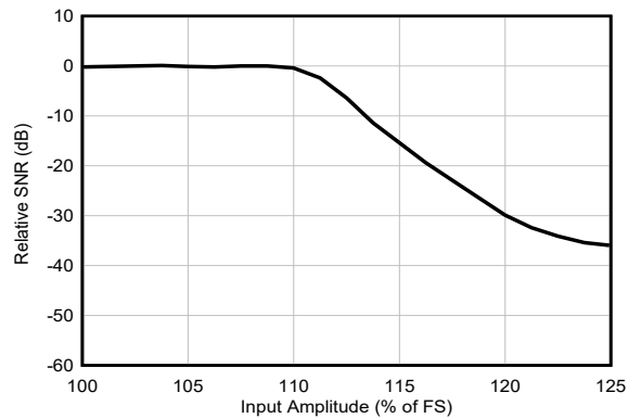
图 7-4. Extended Range SNR Performance
