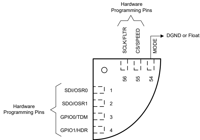
图 7-41. Hardware Programming Mode
