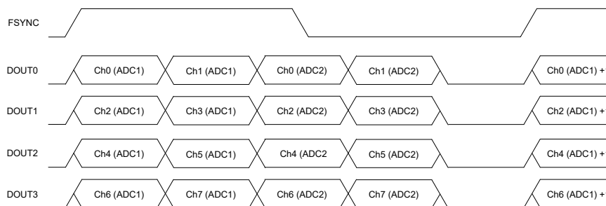
图 7-37. Daisy-Chain Data in TDM Mode (DP_TDM = 01b)
