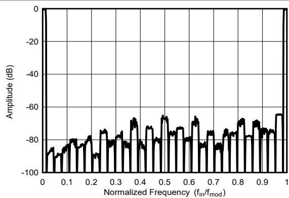
图 7-15. Wideband Filter Stop-Band
