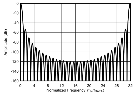
图 7-19. Sinc4 Frequency Response to f_{\text{MOD}} (OSR = 32)
