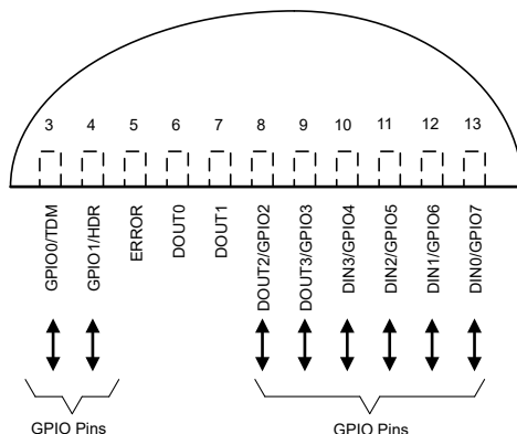
图 7-10. GPIO Pins (ADS127L14 pins shown)
