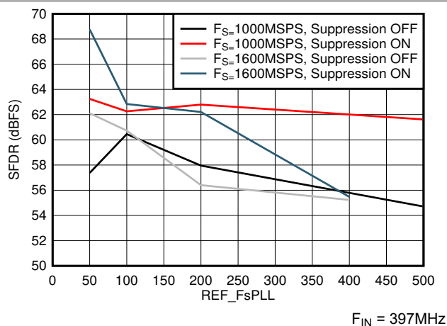
图 5-39. SFDR vs F_{REF} and Suppression
