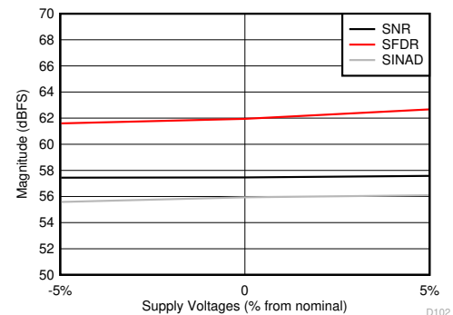
图 5-62. SNR, SFDR and SINAD vs Supply Voltages
