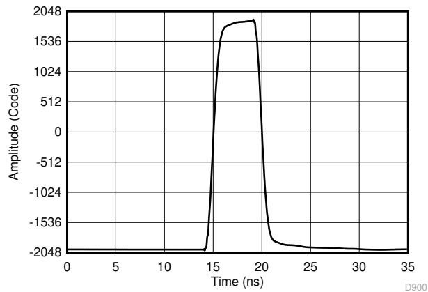
图 7-2. Measured Pulse using Sub-Sampling Technique for Equivalent 32 GSPS Measurement
