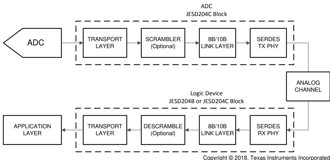
图 6-5. Simplified 8B/10B Encoded JESD204C Interface Diagram
