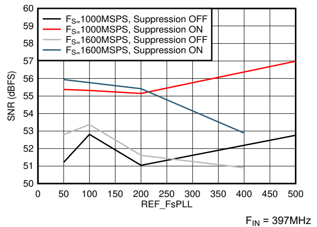
图 5-38. SNR vs F_{REF} and Suppression
