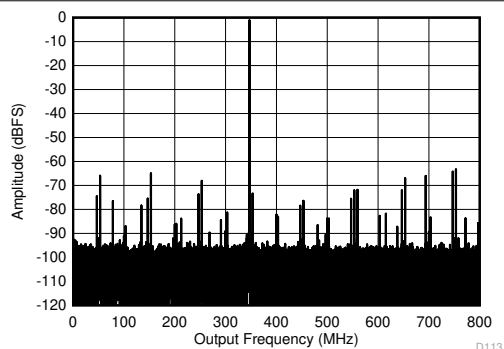
图 5-6. Single Tone FFT at 347 MHz and -1 dBFS
