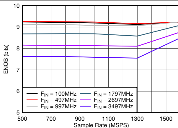
图 5-26. ENOB vs Sample Rate
