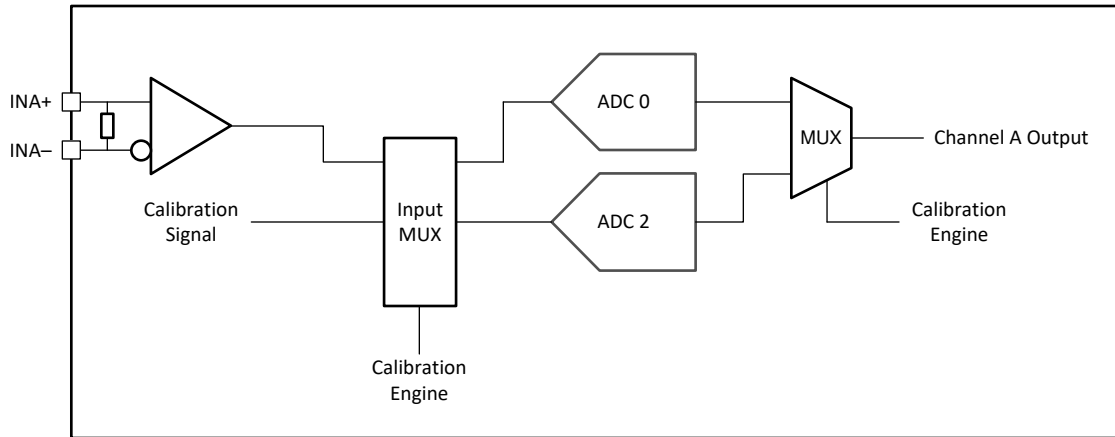
图 6-15. Single Channel Calibration System Block Diagram
