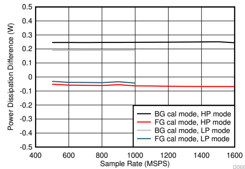
Difference to lower power background calibration, JMODE independent 图 5-110. Dual Channel, Power Dissipation Change with Calibration Mode
