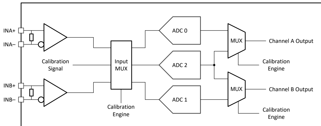
图 6-14. DualChannel Calibration System Block Diagram
