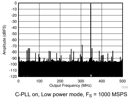
图 5-13. Single Tone FFT at 347 MHz and -1 dBFS
