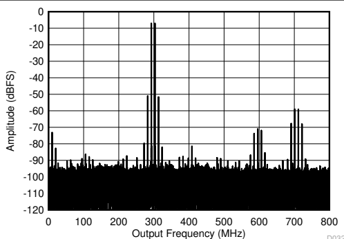
图 5-69. Two Tone FFT at 498MHz
