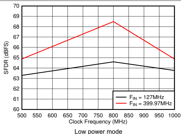
图 5-27. SFDR vs Sample Rate
