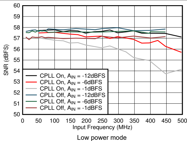
图 5-55. SNR vs A_{IN} and C-PLL
