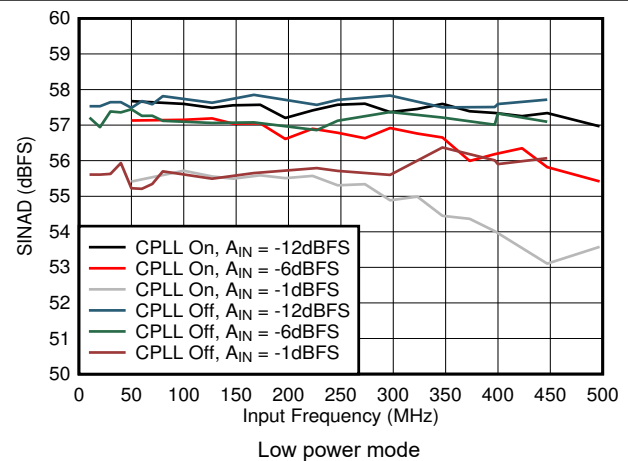
图 5-56. SINAD vs A_{IN} and C-PLL
