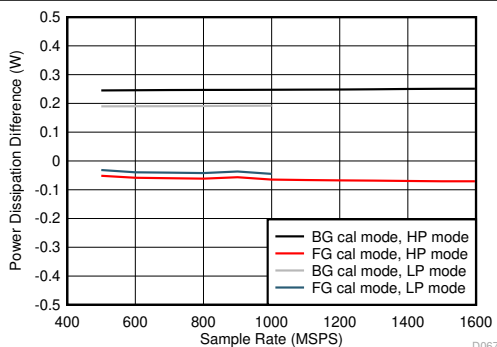
Difference to lower power background calibration, JMODE independent 图 5-111. Single Channel, Power Dissipation Change with Calibration Mode
