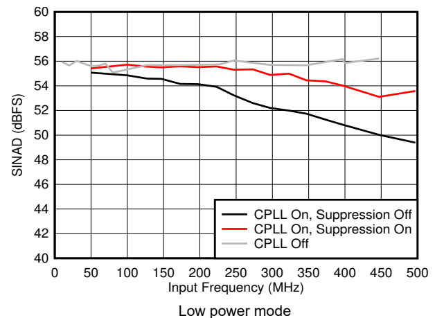
图 5-46. SINAD vs F_{IN} and C-PLL modes
