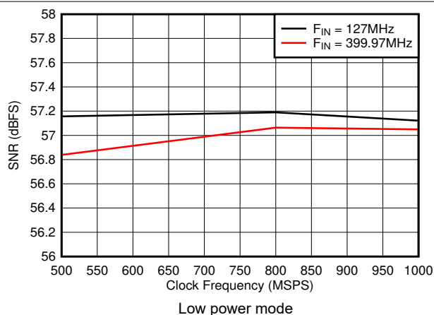
图 5-28. SNR vs Sample Rate
