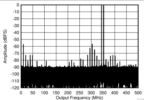
图 5-70. Two Tone FFT at 1798MHz
