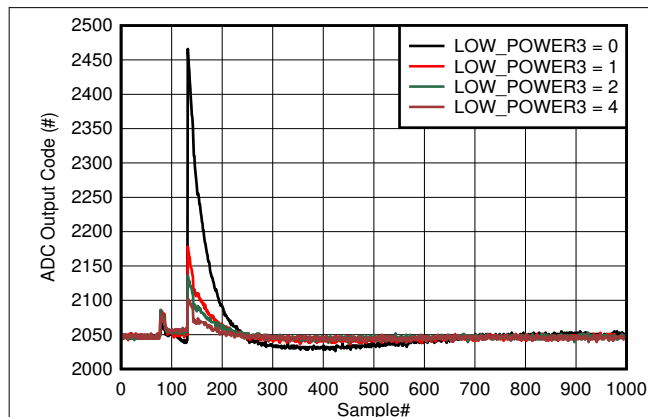
图 6-10. Background Calibration Core Transition In Low Power Mode
