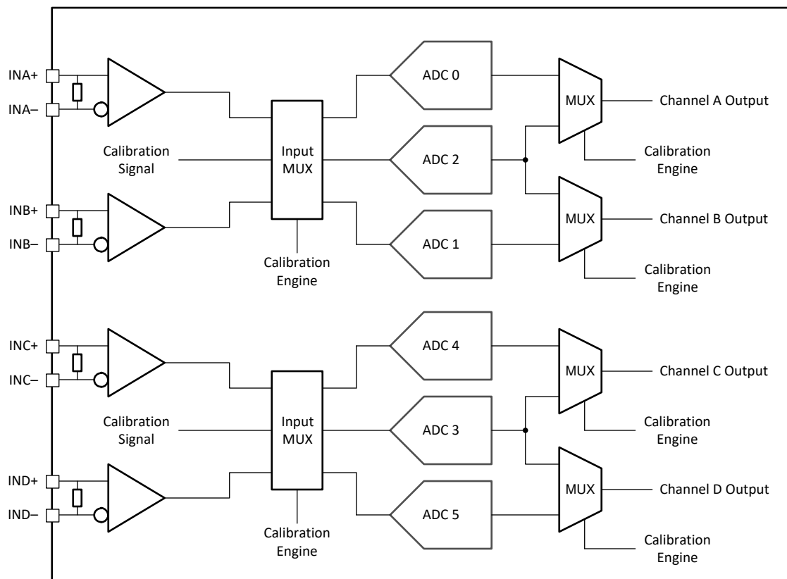
图 6-13. Quad Channel Calibration System Block Diagram
