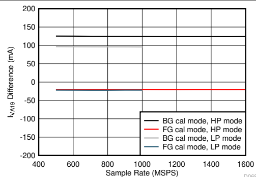
Difference to lower power background calibration, JMODE independent 图 5-112. Quad Channel, I_{VA19} Change with Calibration Mode
