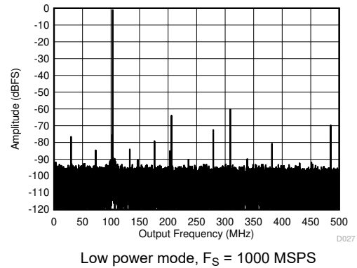
图 5-14. Single Tone FFT at 897 MHz and -1 dBFS
