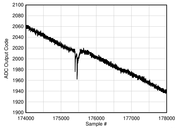
图 5-125. Background Calibration Core Transition (offset voltage)
