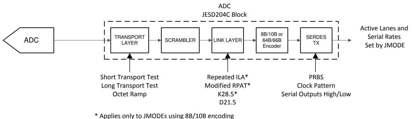
图 6-12. Test Mode Insertion Points
