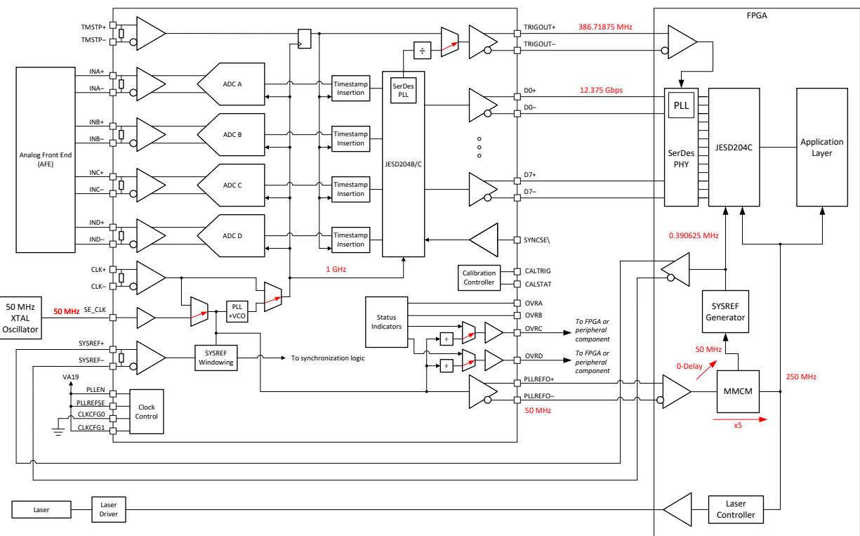
图 7-1. Typical Configuration for a LiDAR Digitizer
