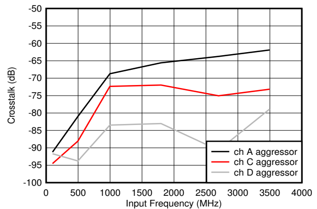
图 5-78. Crosstalk to Channel B vs F_{IN}
