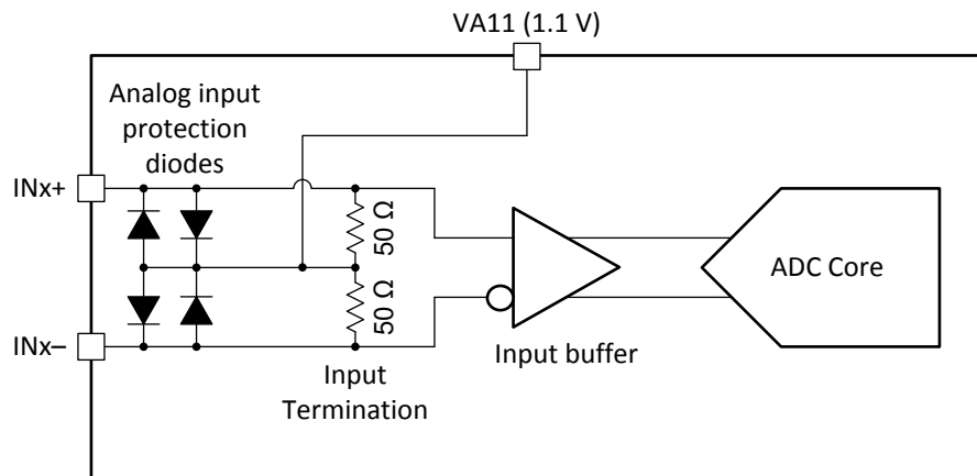
图 6-2. Analog Input Internal Termination and Protection Diagram
