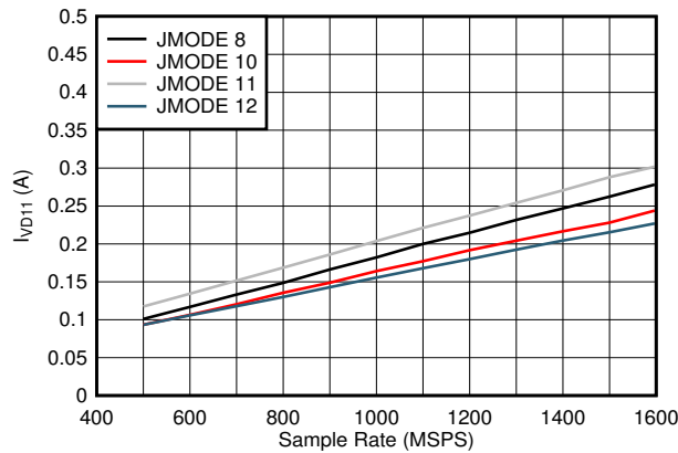
Low power background calibration mode 图 5-107. Single Channel, I_{VD11} vs F_S and JMODE 8 - 12
