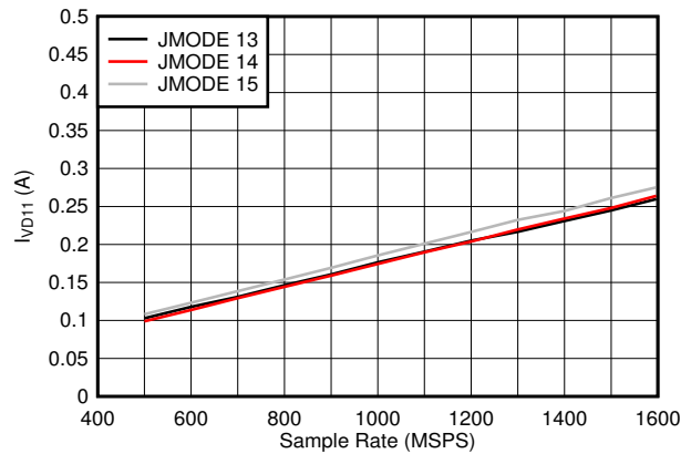
Low power background calibration mode 图 5-108. Single Channel, I_{VD11} vs F_S and JMODE 13 - 15
