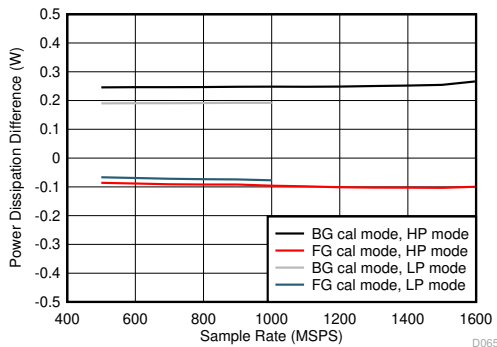
Difference to lower power background calibration, JMODE independent 图 5-109. Quad Channel, Power Dissipation Change with Calibration Mode
