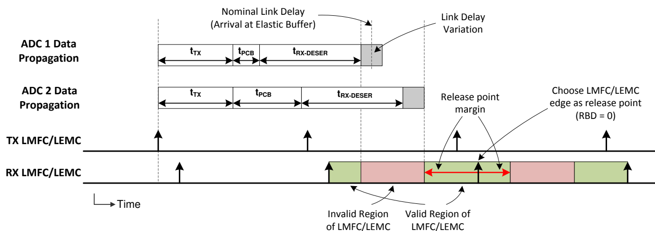
图 6-9. LMFC/LEMC Valid Region Definition for Elastic Buffer Release Point Selection
