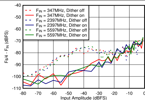
图 5-72. DES Mode: F_s/4 - F_{\text{IN}} vs Input Amplitude and Dither
