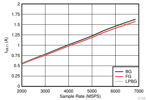
图 5-124. DES Mode: I_{VA11} vs Sample Rate
