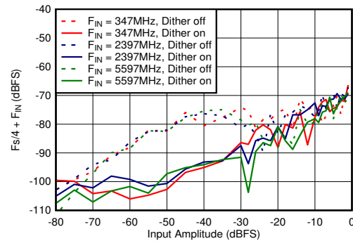
图 5-68. DES Mode: F_s/2 - F_{\text{IN}} vs Input Amplitude and Dither
