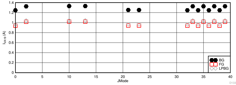
图 5-119. Other Modes with Lower Maximum FS: I_{VA19} vs JMODE
