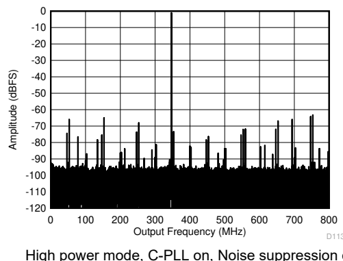
图 7-6. Single Tone FFT at 347 MHz and -1 dBFS
