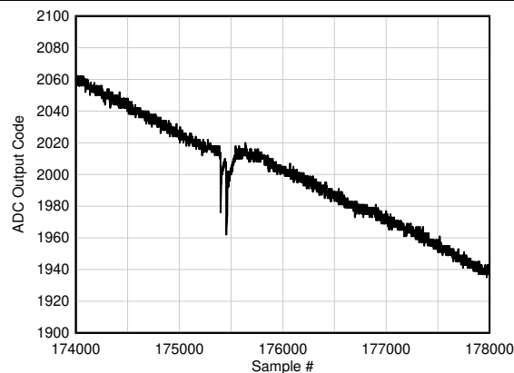
图 7-125. Background Calibration Core Transition (offset voltage)
