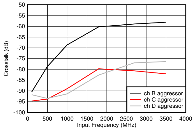
图 7-77. Crosstalk to Channel A vs F_{IN}
