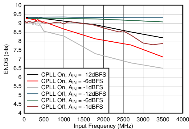
图 7-51. ENOB vs A_{IN} and C-PLL
