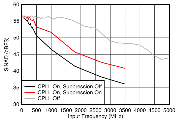
图 7-42. SINAD vs F_{IN} and C-PLL modes
