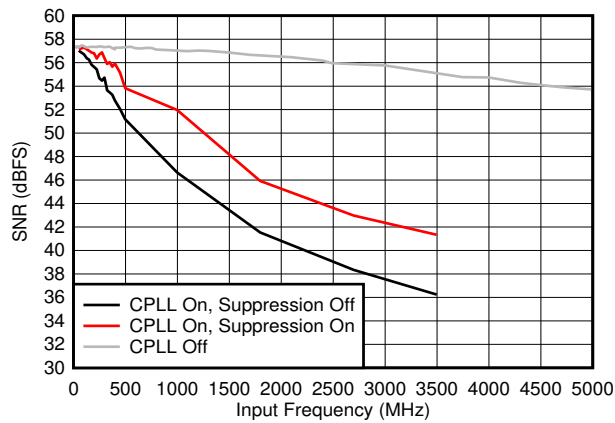
图 7-41. SNR vs F_{IN} and C-PLL modes
