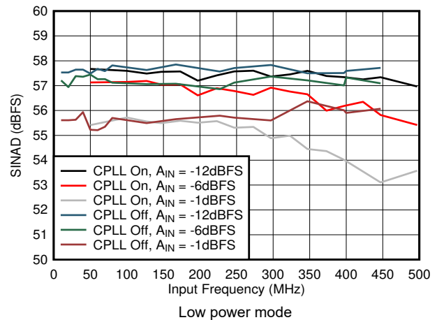
图 7-56. SINAD vs A_{IN} and C-PLL
