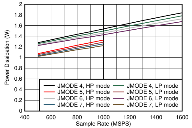
图 7-90. Dual Channel, Power Dissipation vs F_S and JMODE 4 - 7
