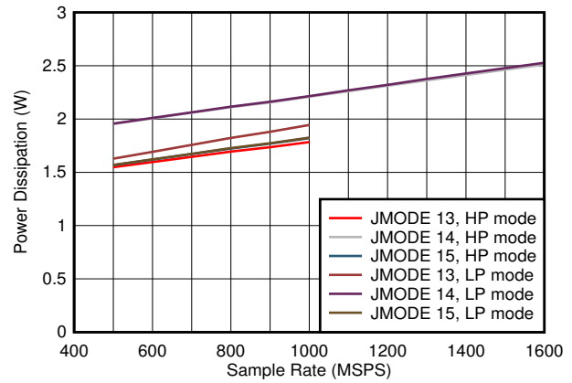
图 7-82. Quad Channel, Power Dissipation vs F_S and JMODE 13 - 15
