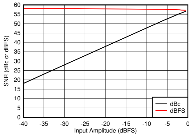
图 7-35. SNR vs A_{IN}
