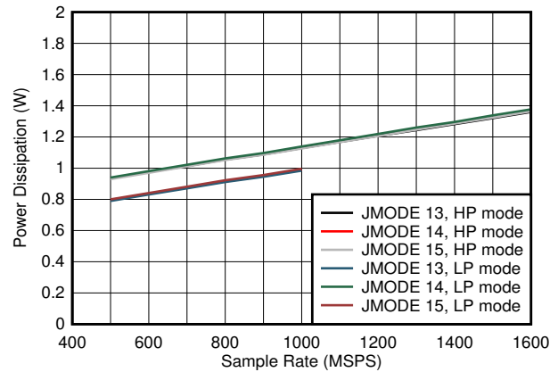
图 7-102. Single Channel, Power Dissipation vs F_S and JMODE 13 - 15
