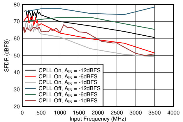
图 7-48. SFDR vs A_{IN} and C-PLL
