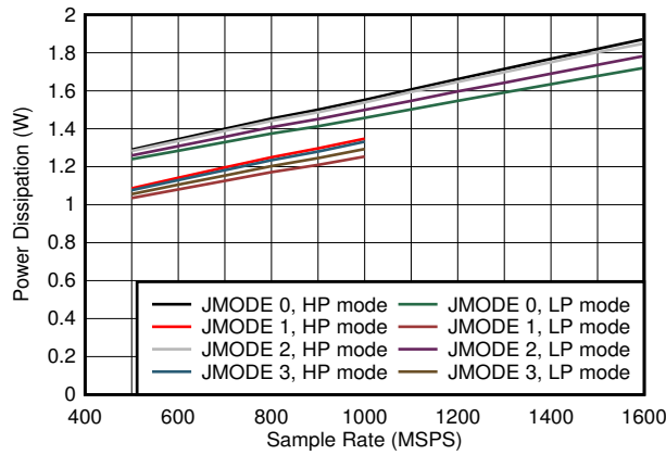
图 7-89. Dual Channel, Power Dissipation vs F_S and JMODE 0 - 3
