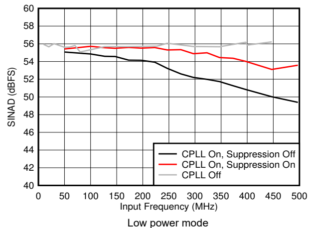
图 7-46. SINAD vs F_{IN} and C-PLL modes
