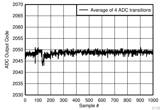
图 7-124. Background Calibration Core Transition (midscale voltage)
