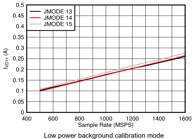
图 7-108. Single Channel, I_{VD11} vs F_S and JMODE 13 - 15
