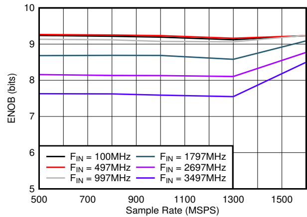
图 7-26. ENOB vs Sample Rate
