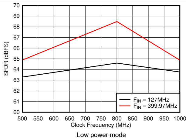
图 7-29. SFDR vs Sample Rate
