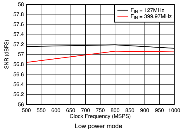
图 7-28. SNR vs Sample Rate
