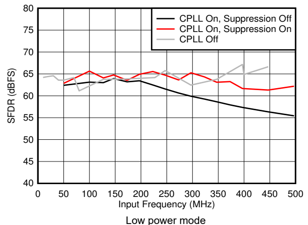
图 7-44. SFDR vs F_{IN} and C-PLL modes
