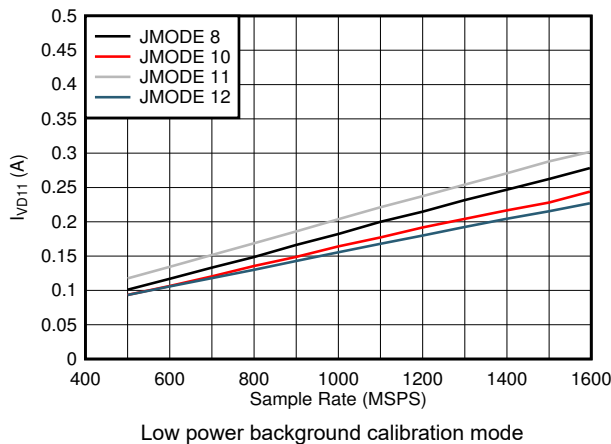
图 7-107. Single Channel, I_{VD11} vs F_S and JMODE 8 - 12
