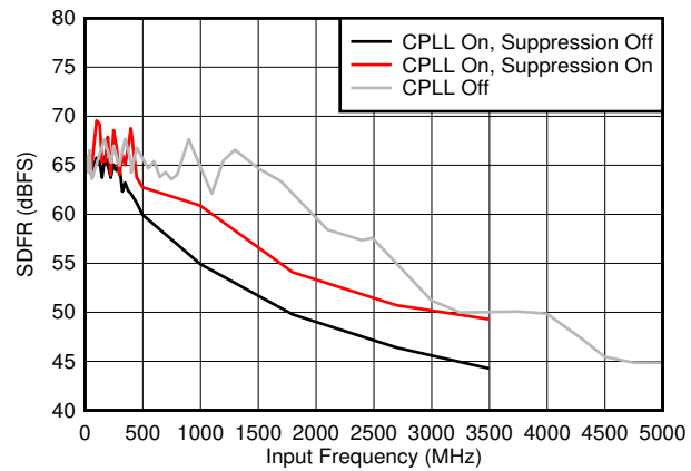
图 7-40. SFDR vs F_{IN} and C-PLL modes
