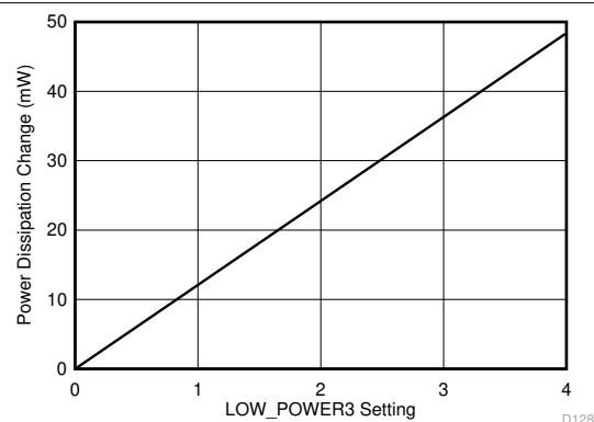
图 8-11. Power Dissipation Change vs LOW_POWER3 register setting
