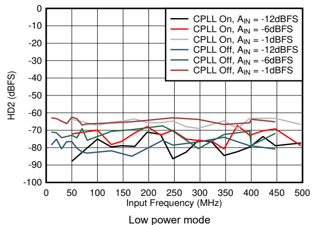
图 7-58. HD2 vs A_{IN} and C-PLL
