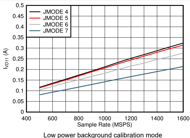
图 7-106. Single Channel, I_{VD11} vs F_S and JMODE 4 - 7
