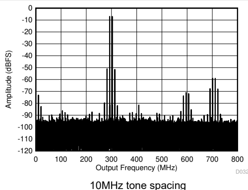
图 7-71. Two Tone FFT at 3498MHz
