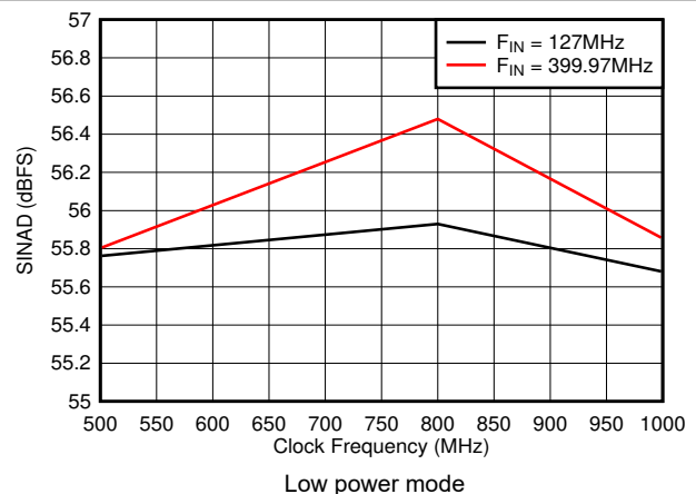
图 7-30. SINAD vs Sample Rate
