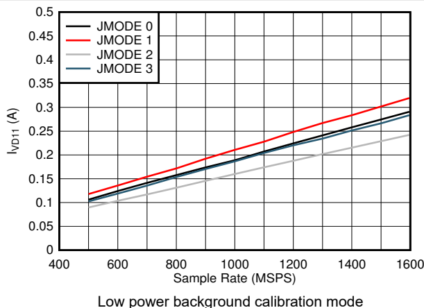
图 7-105. Single Channel, I_{VD11} vs F_S and JMODE 0 - 3
