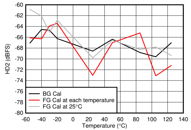
图 7-66. HD2 vs Temperature
