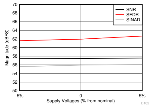
All supplies changed together, low power mode, F_S = 1000 MSPS 图 7-62. SNR, SFDR and SINAD vs Supply Voltages
