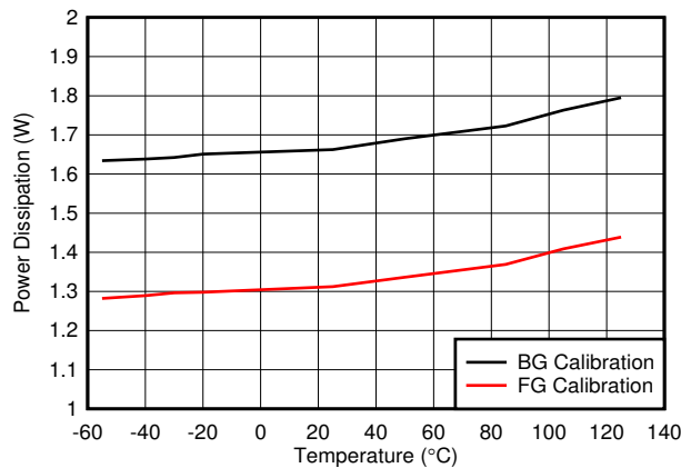
图 7-123. Single Channel, Power Dissipation vs Temperature
