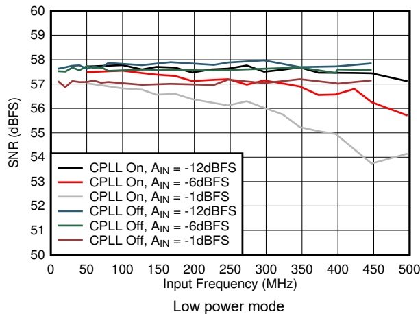
图 7-55. SNR vs A_{IN} and C-PLL
