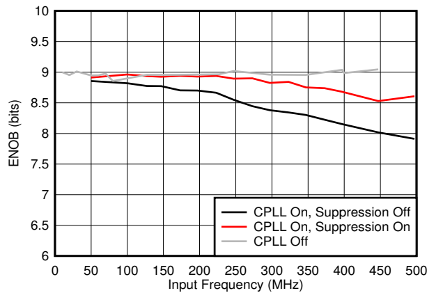
图 7-47. ENOB vs F_{IN} and C-PLL modes
