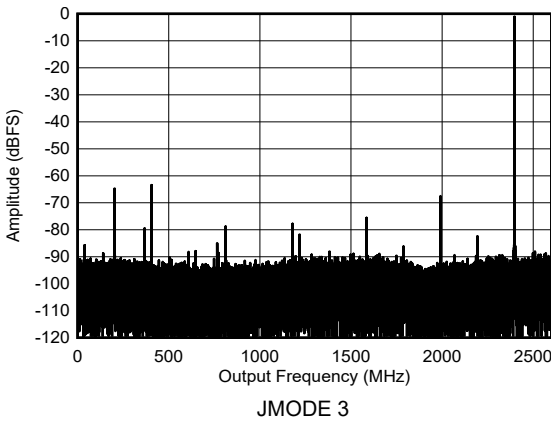
图 5-49. Dual Channel Mode: Single Tone Spectrum at 2397 MHz
