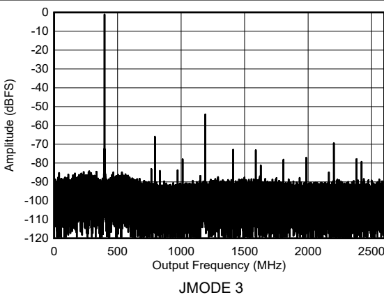
图 5-51. Dual Channel Mode: Single Tone Spectrum at 5597 MHz
