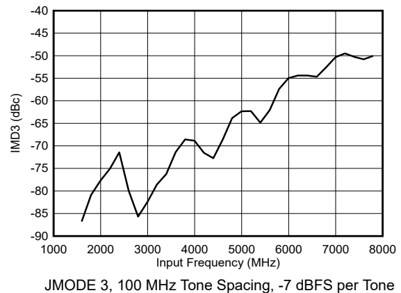
图 5-44. Dual Channel Mode: IMD3 vs Input Frequency
