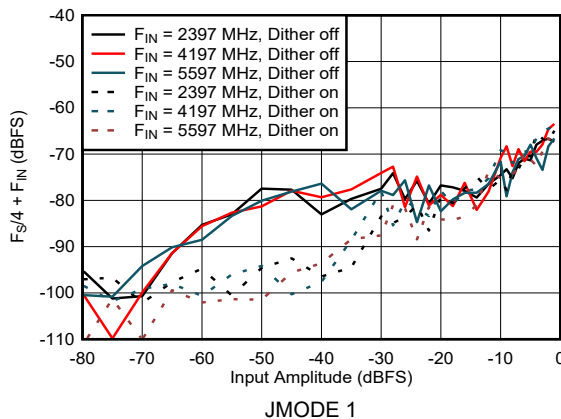
图 5-21. DES Mode: F_S/4 + F_{\text{IN}} vs Input Amplitude
