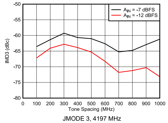
图 5-48. Dual Channel Mode: IMD3 vs Tone Spacing
