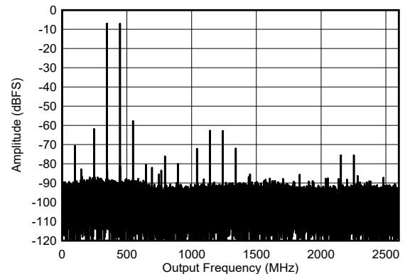
图 5-54. Dual Channel Mode: Dual Tone Spectrum at 5597 MHz
