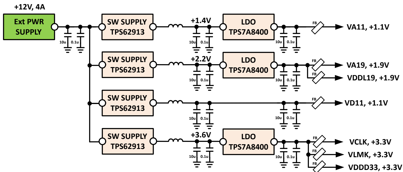
图 7-5. LDO Linear Regulator Approach Example
