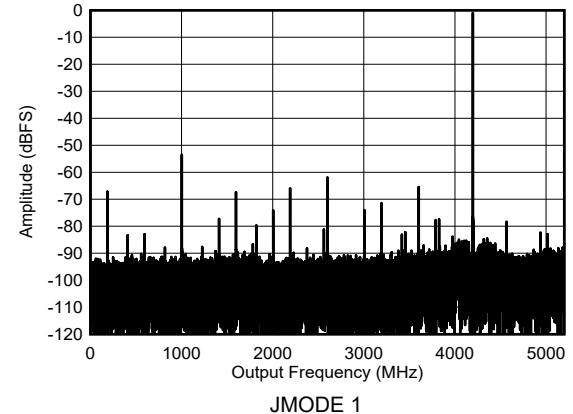
图 5-28. DES Mode: Single Tone Output Spectrum at 4197 MHz
