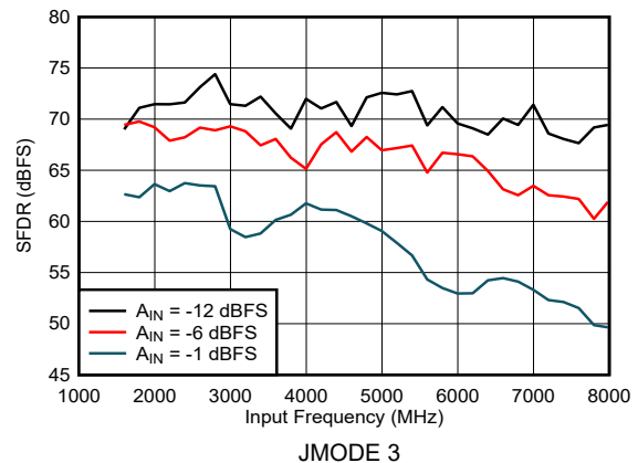
图 5-34. Dual Channel Mode: SFDR vs Input Frequency
