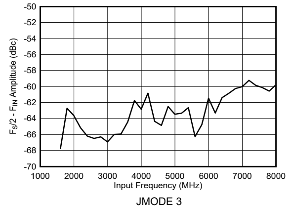
图 5-38. Dual Channel Mode: F_S/2 - F_{\text{IN}} vs Input Frequency
