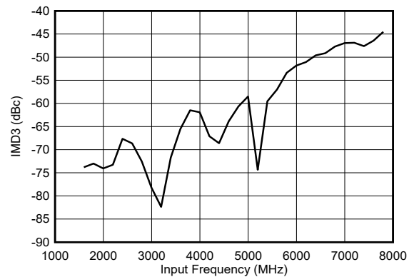
图 5-22. DES Mode: IMD3 vs Input Frequency
