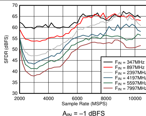
图 6-32. DES Mode: SFDR vs Sample Rate and Input Frequency
