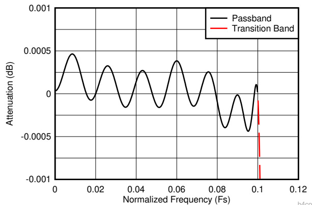
图 7-12. Decimate-by-4 Composite Zoomed Pass-Band Response
