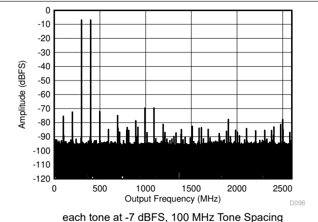
图 6-23. Dual Channel Mode: Two Tone FFT at 347 MHz
