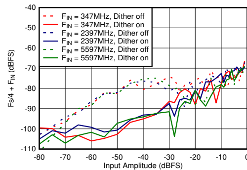
图 6-68. DES Mode: F_s/2 - F_{\text{IN}} vs Input Amplitude and Dither
