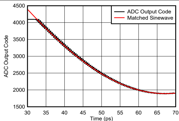
FIG 6-151. Sinewave Overdrive Recovery
