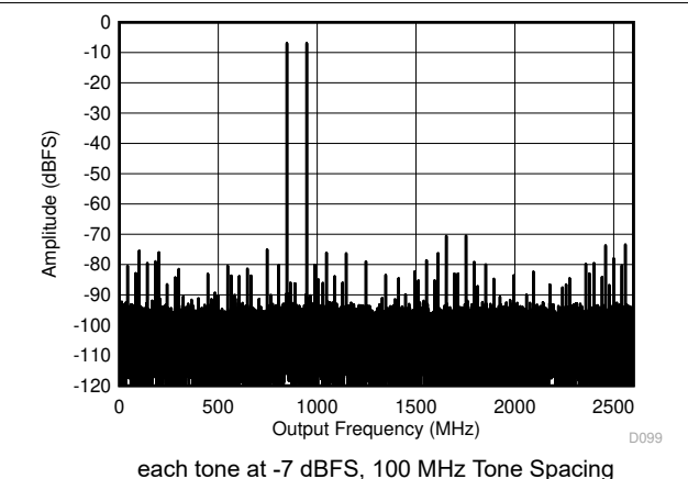
图 6-24. Dual Channel Mode: Two Tone FFT at 897 MHz
