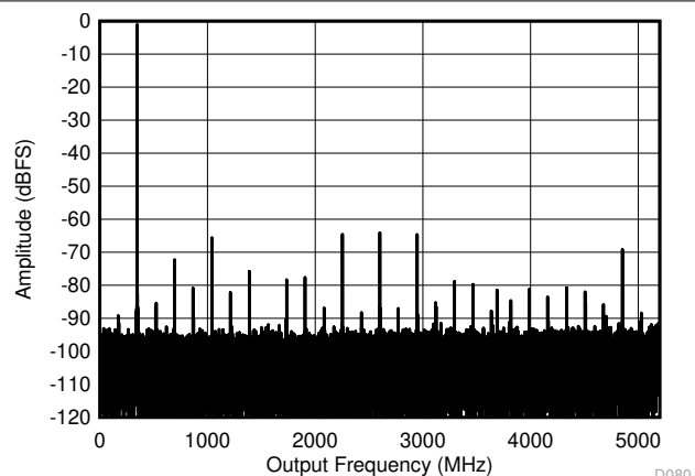
图 6-5. DES Mode: Single Tone FFT at 347 MHz
