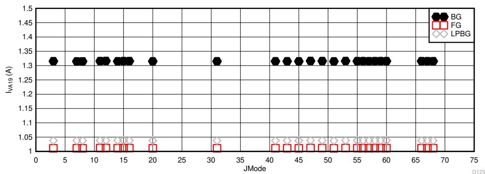
图 6-114. DES Mode: Power Dissipation vs JMODE at 10.4GSPS
