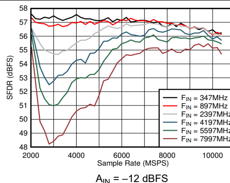
图 6-34. DES Mode: SFDR vs Sample Rate and Input Frequency
