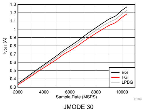
图 6-127. DES Mode: I_{VD11} vs Sample Rate
