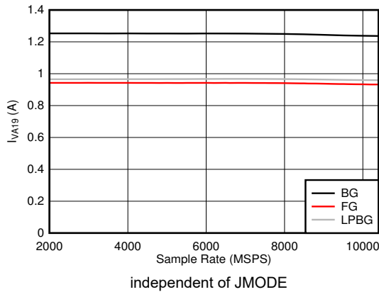
图 6-123. DES Mode: I_{VA19} vs Sample Rate
