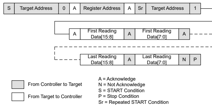
图 7-24. Read Same Register Multiple Times
