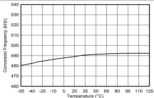
图 6-39. Conversion Frequency vs Temperature
