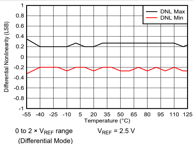
图 6-31. Differential Linearity Error vs Temperature
