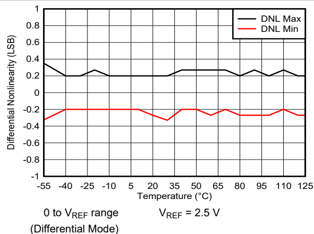
图 6-30. Differential Linearity Error vs Temperature
