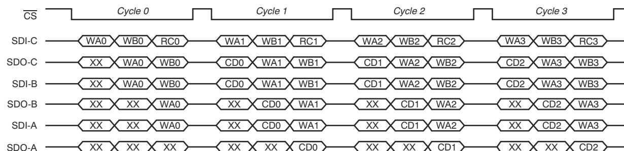
图 7-32. Writing to Devices A and B, and Reading Device C
