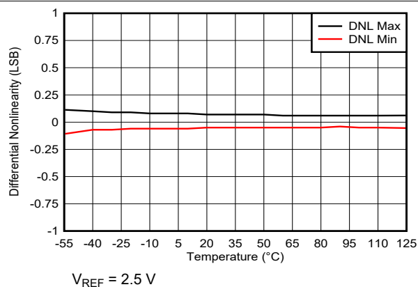
图 6-8. Differential Linearity Error vs Temperature
