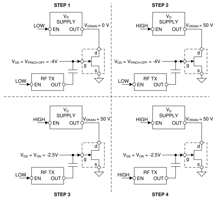
图 8-2. GaN Power Sequencing
