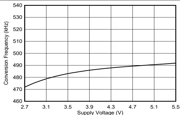
图 6-38. Conversion Frequency vs Supply
