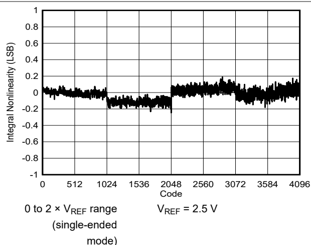
图 6-23. Integral Linearity Error vs Code
