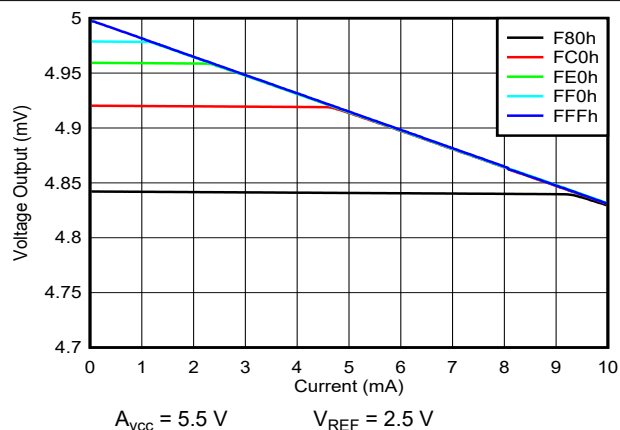
图 6-13. Output Voltage vs Source Current Capability
