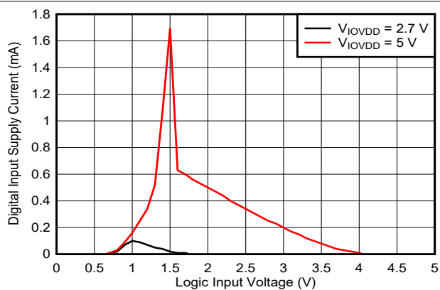
图 6-50. Supply Current vs Input Voltage
