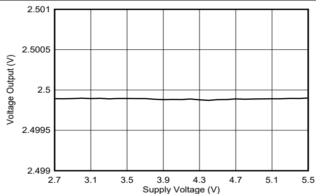
图 6-44. Output Voltage vs Supply
