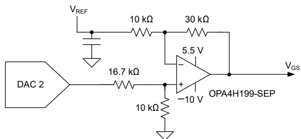
图 8-3. Differential Operational Amplifier Circuit
