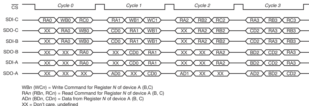
图 7-31. Mixed Operation: Reading Devices A and C, and Writing to Device B; Then Reading A, and Writing to B and C; Then Reading A, B, and C Twice
