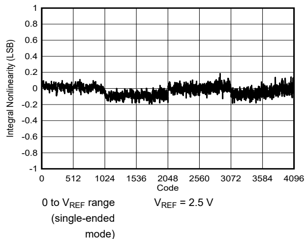
图 6-21. Integral Linearity Error vs Code
