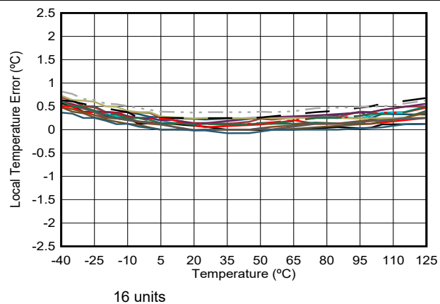
图 6-48. Local Temperature Error vs Temperature
