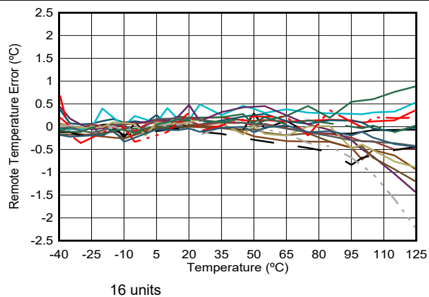
图 6-49. Remote Temperature Error vs Temperature
