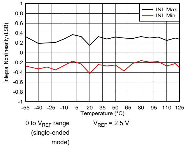
图 6-32. Integral Linearity Error vs Temperature
