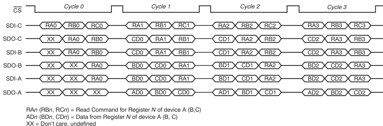
图 7-30. Reading Multiple Registers
