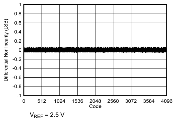
图 6-6. Differential Linearity Error vs Code
