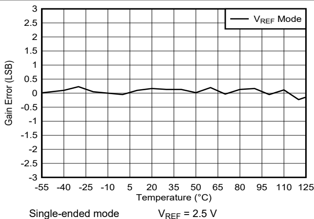
图 6-36. Gain Error vs Temperature
