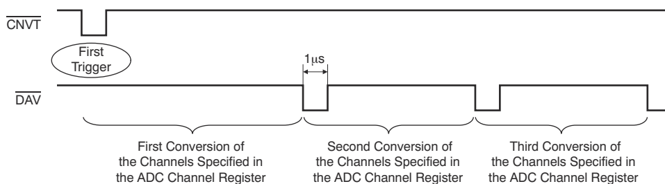
图 7-20. ADC External Trigger
