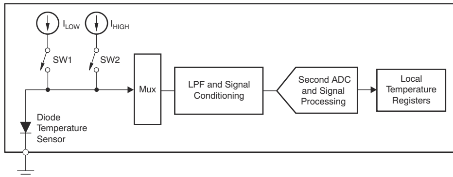
图 7-4. Integrated Local Temperature Sensor
