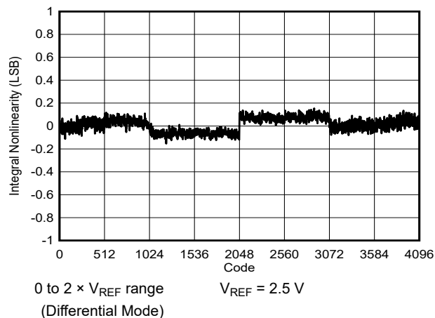
图 6-27. Integral Linearity Error vs Code
