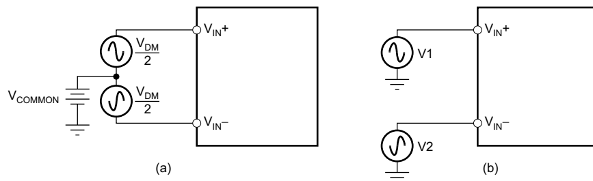
图 7-2. Fully Differential Analog Input
