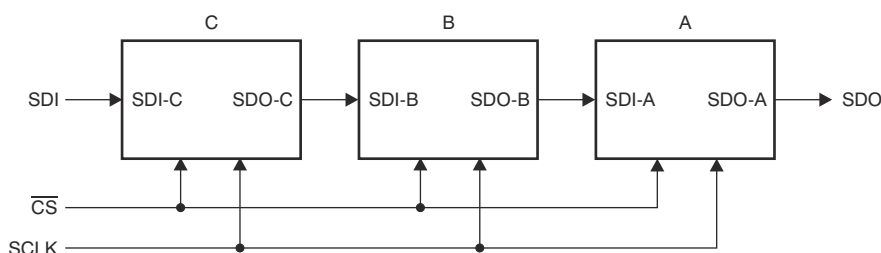
图 7-29. Three devices in a Daisy-Chain Configuration
