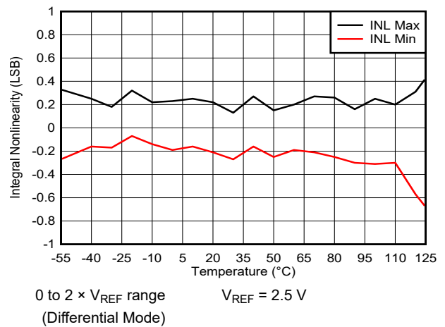
图 6-35. Integral Linearity Error vs Temperature
