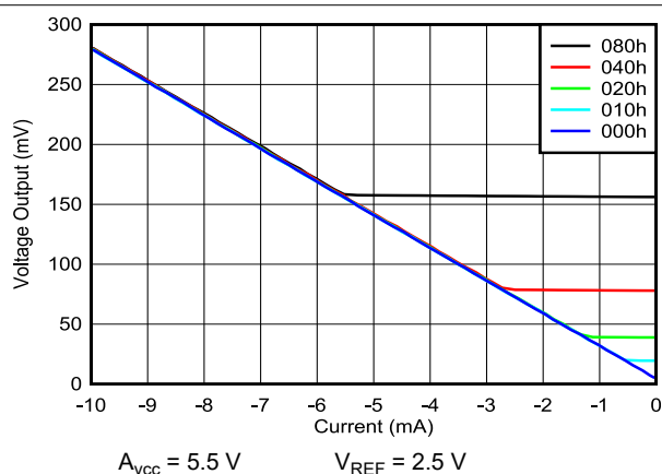
图 6-14. Output Voltage vs Sink Current Capability
