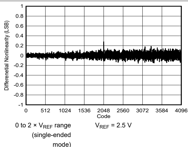
图 6-22. Differential Linearity Error vs Code
