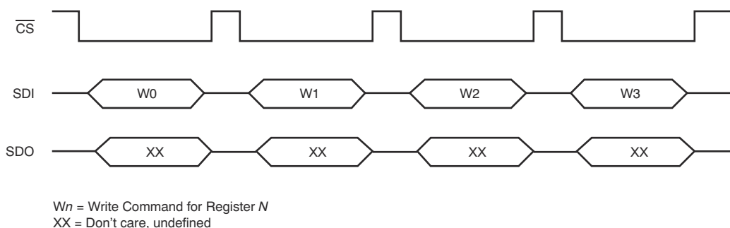
图 7-27. Write Operation in Standalone Mode
