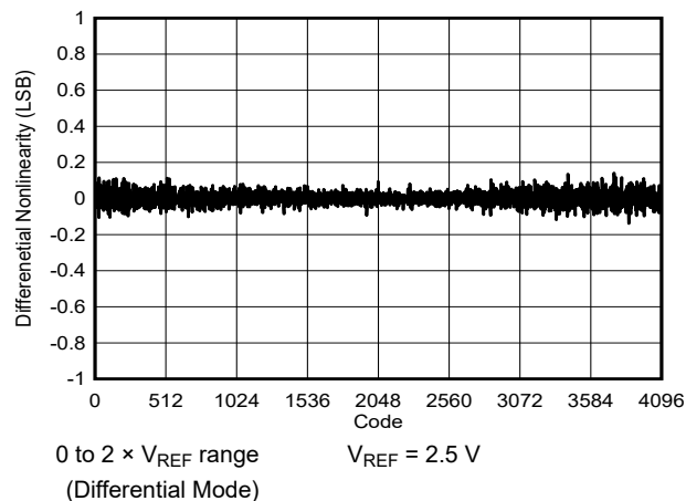
图 6-26. Differential Linearity Error vs Code
