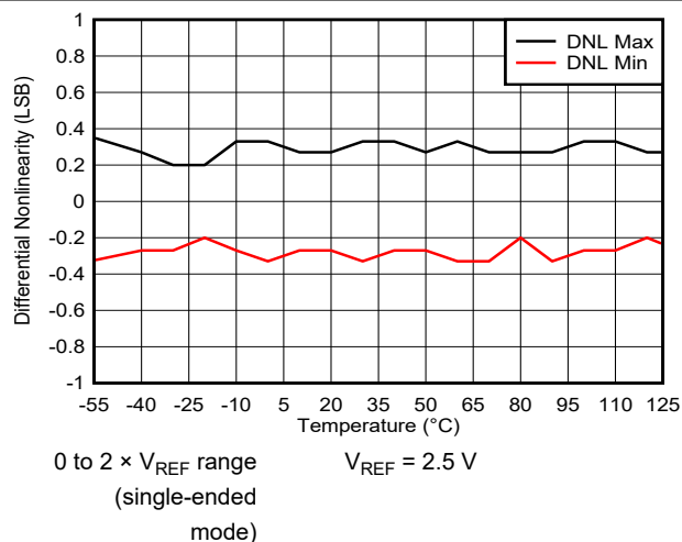
图 6-29. Differential Linearity Error vs Temperature
