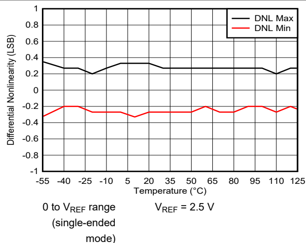
图 6-28. Differential Linearity Error vs Temperature
