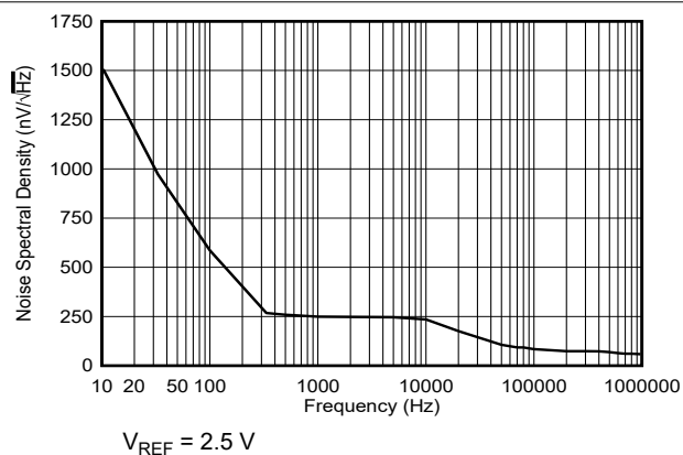
图 6-16. DAC Noise Voltage vs Frequency
