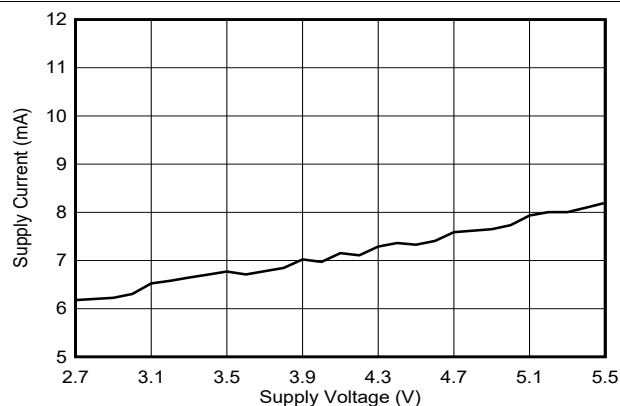
图 6-40. Supply Current vs Supply Voltage
