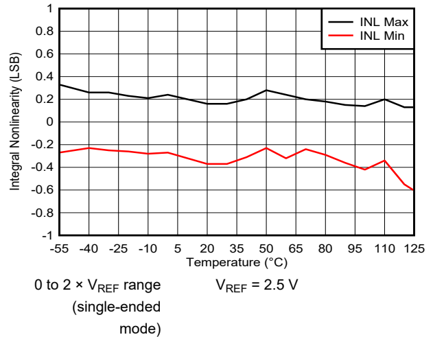
图 6-33. Integral Linearity Error vs Temperature
