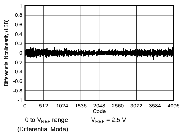
图 6-24. Differential Linearity Error vs Code
