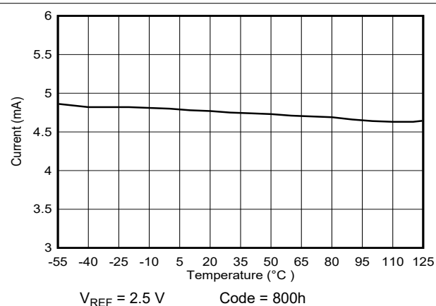
图 6-15. Supply Current vs Temperature
