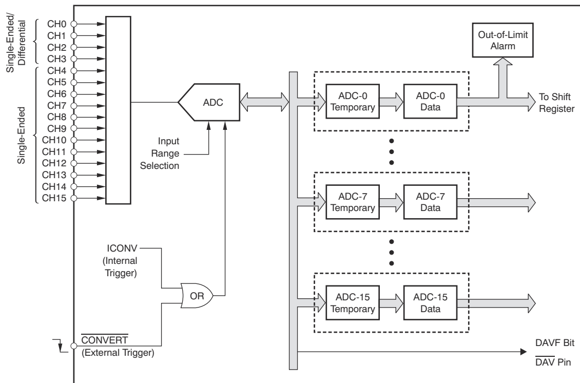
图 7-3. Double-Buffered ADC Structure
