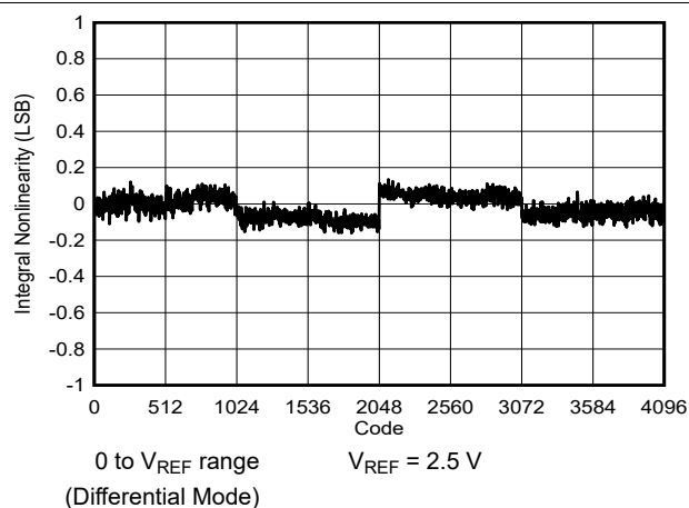
图 6-25. Integral Linearity Error vs Code
