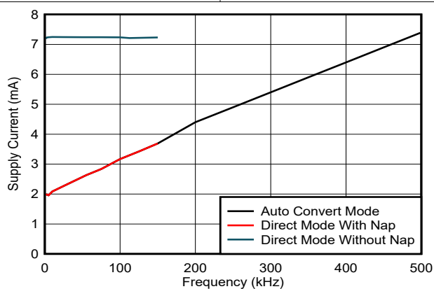
图 6-42. Supply Current vs Conversion Rate
