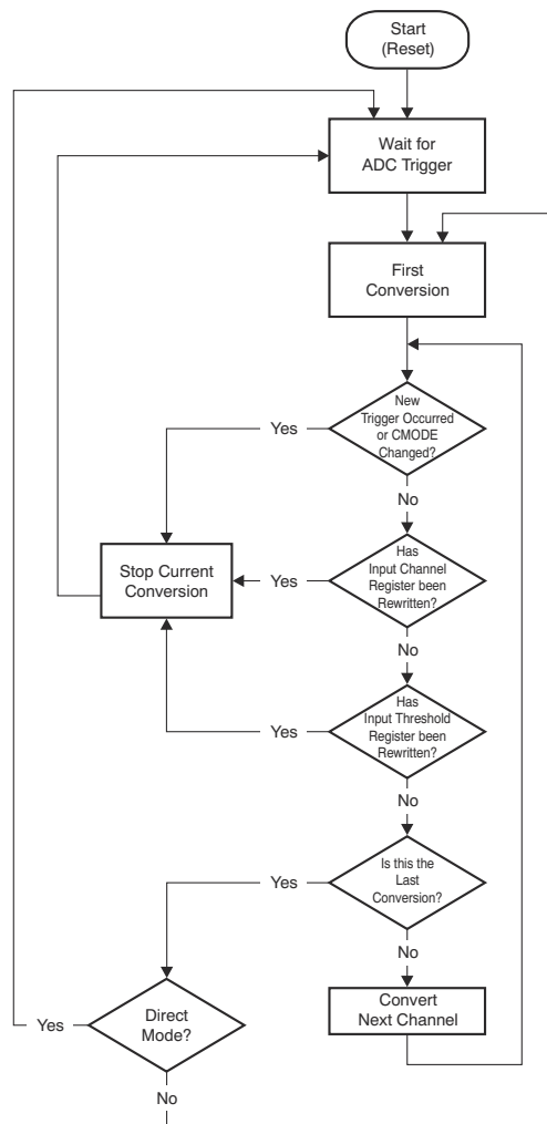
图 7-18. ADC Conversion Sequence
