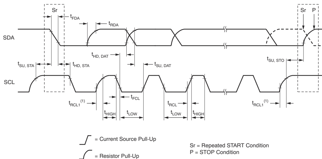
图 6-2. Timing for High-Speed (Hs) Mode Devices on I 2 C Bus
