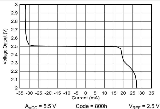
图 6-12. Output Voltage vs Output Current
