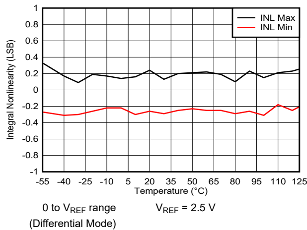
图 6-34. Integral Linearity Error vs Temperature
