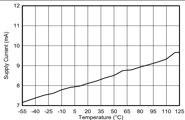
图 6-41. Supply Current vs Temperature
