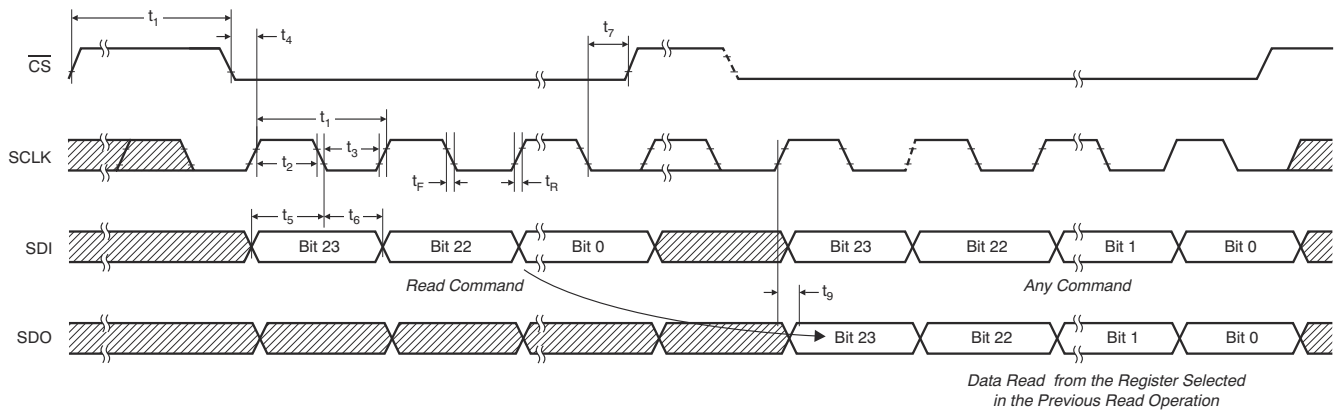
图 6-4. Timing for SPI Single-Chip Read Operation
