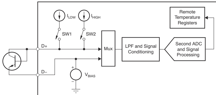
图 7-5. Remote Temperature Sensor
