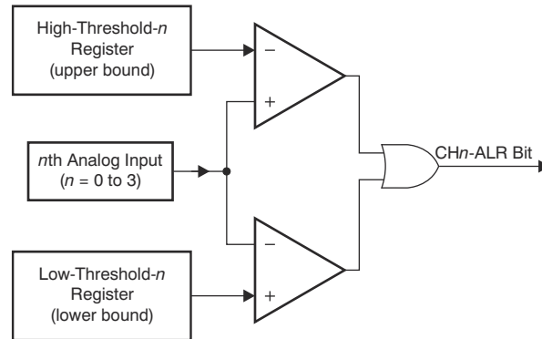
图 7-13. Chn Out-of-Range Alarm
