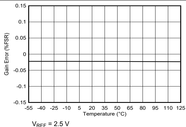
图 6-10. Gain Error vs Temperature
