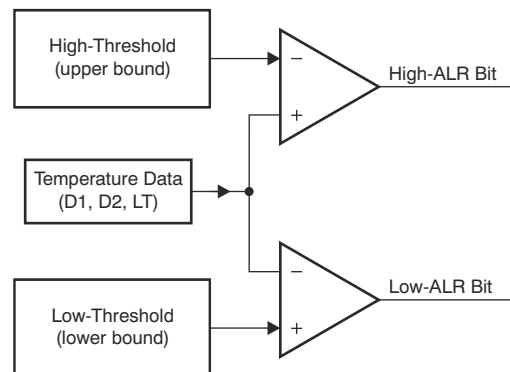
图 7-14. Temperature Out-of-Range Alarm
