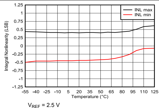
图 6-9. Integral Linearity Error vs Temperature
