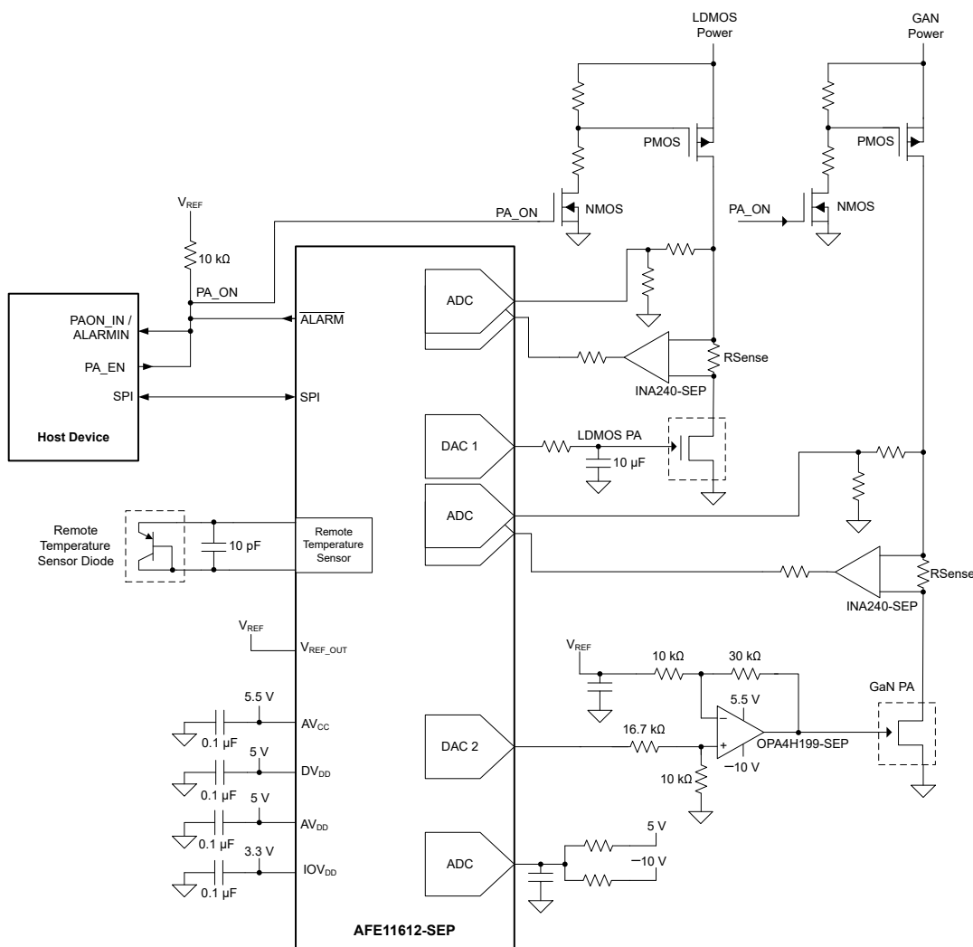
图 8-1. Power Amplifier (PA) Biasing
