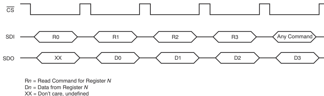
图 7-28. Read Operation in Standalone Mode
