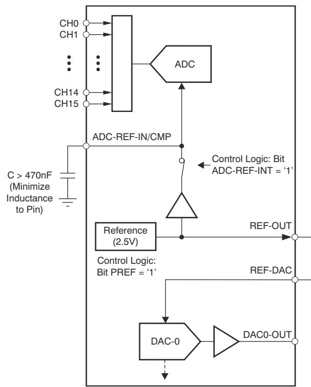
图 7-8. Use of the Internal Reference
