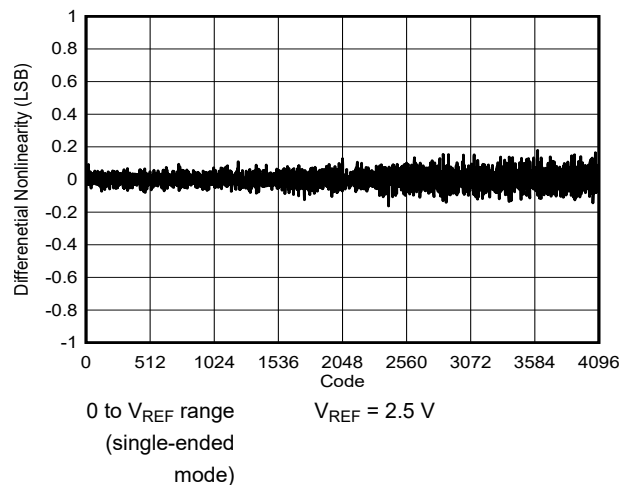
图 6-20. Differential Linearity Error vs Code
