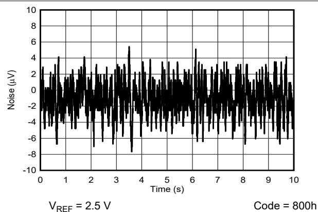
图 6-17. DAC Noise (0.1 Hz to 10 Hz)
