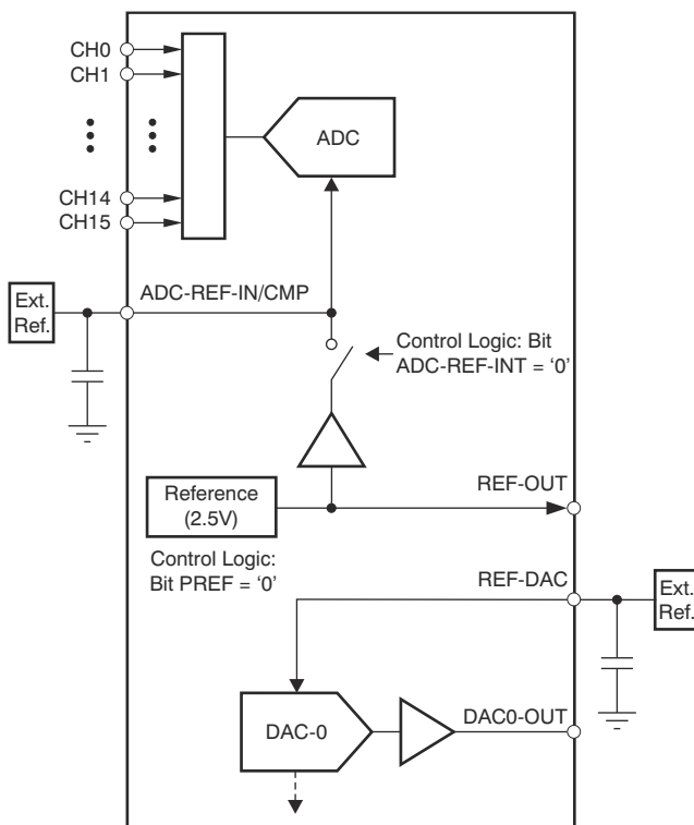
图 7-7. Use of the External Reference
