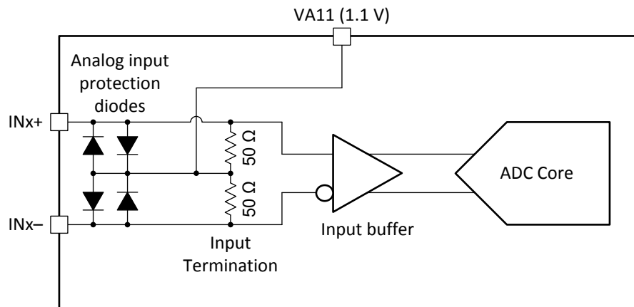
图 8-2. Analog Input Internal Termination and Protection Diagram
