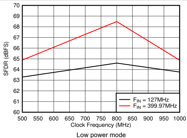
图 7-29. SFDR vs Sample Rate
