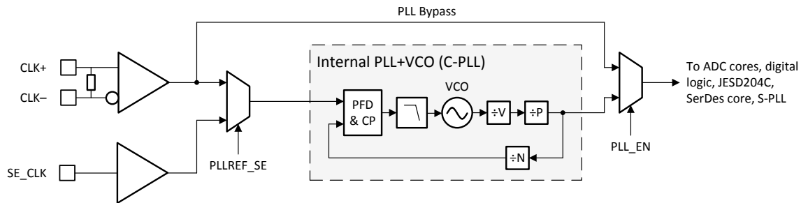
图 8-4. Converter PLL (C-PLL) Architecture
