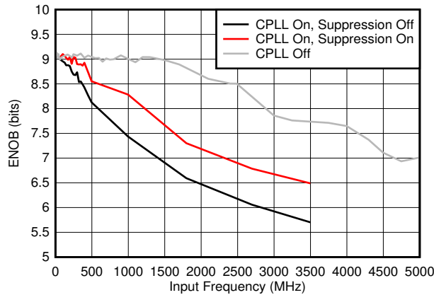
图 7-43. ENOB vs F_{IN} and C-PLL modes
