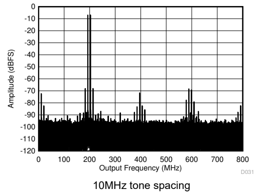
图 7-70. Two Tone FFT at 1798MHz
