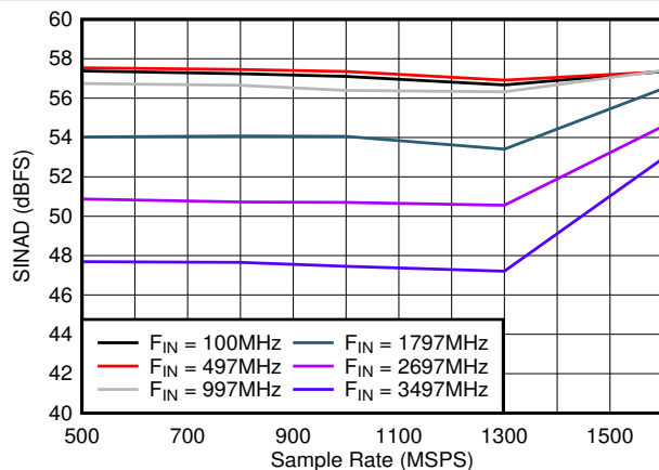
图 7-25. SINAD vs Sample Rate
