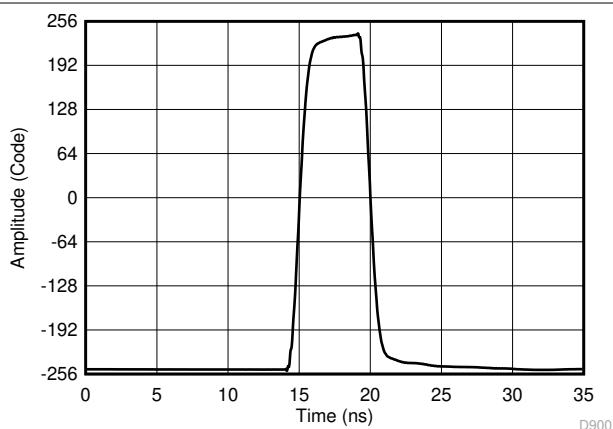
图 9-2. Measured Pulse using Sub-Sampling Technique for Equivalent 32 GSPS Measurement
