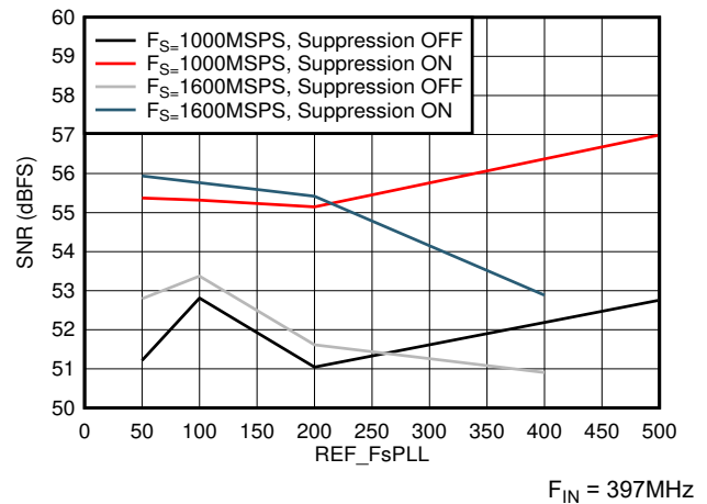
图 7-38. SNR vs F_{REF} and Suppression
