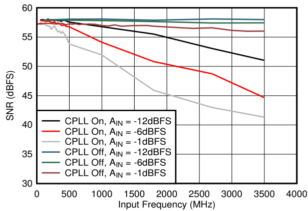
图 7-49. SNR vs A_{IN} and C-PLL
