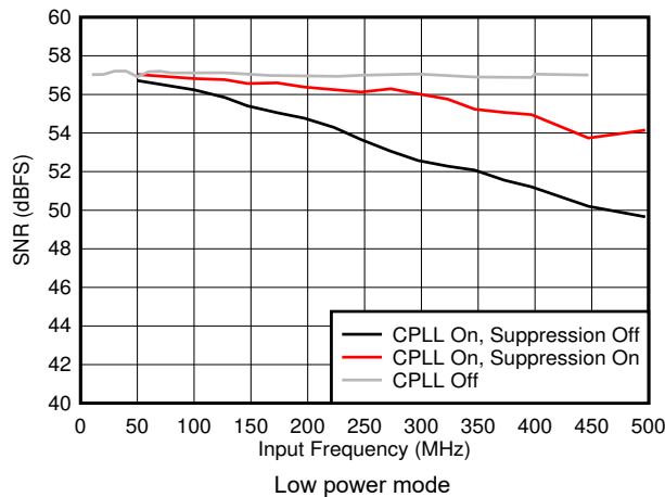
图 7-45. SNR vs F_{IN} and C-PLL modes
