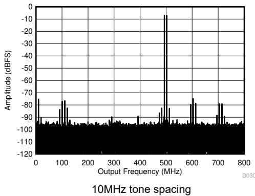
图 7-69. Two Tone FFT at 498MHz
