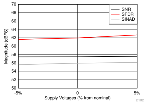
图 7-62. SNR, SFDR and SINAD vs Supply Voltages
