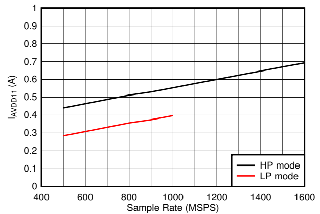
图 7-84. Quad Channel, I_{VDD11} vs F_S
