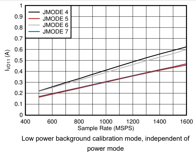
图 7-86. Quad Channel, I_{VD11} vs F_S and JMODE 4 - 7
