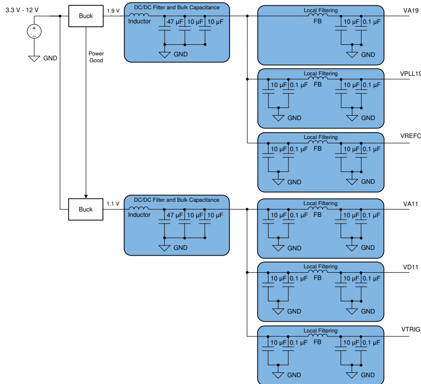
图 9-4. Switcher-Only Approach Example
