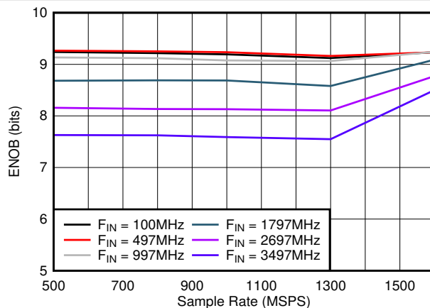
图 7-26. ENOB vs Sample Rate
