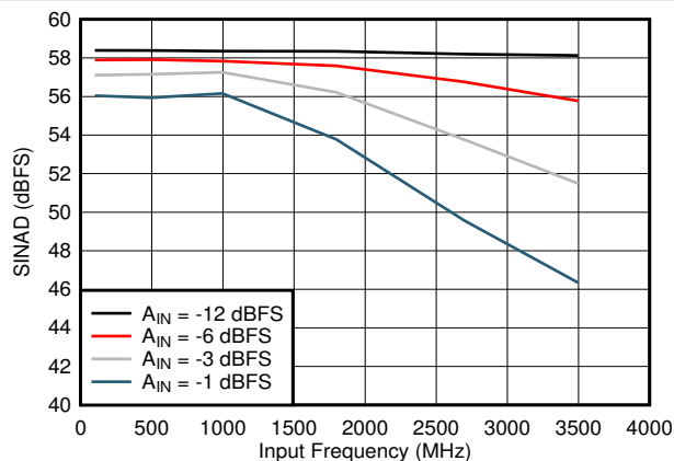
图 7-19. SINAD vs Input Frequency
