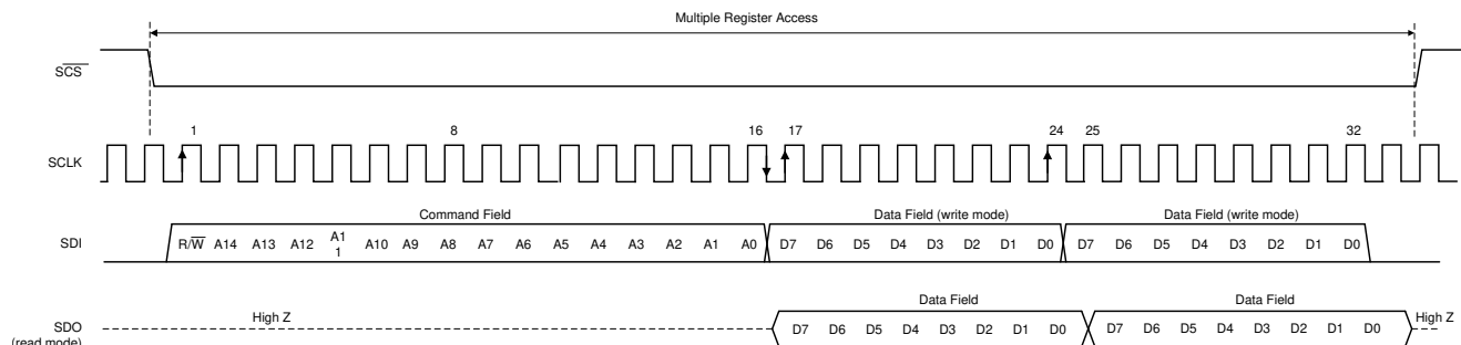
图 8-17. Serial Interface Protocol: Streaming Read/Write
