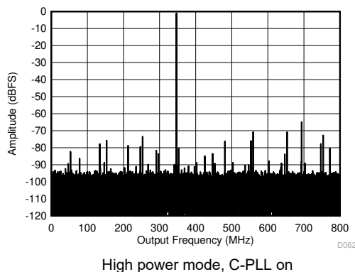
图 7-5. Single Tone FFT at 347 MHz and -1 dBFS
