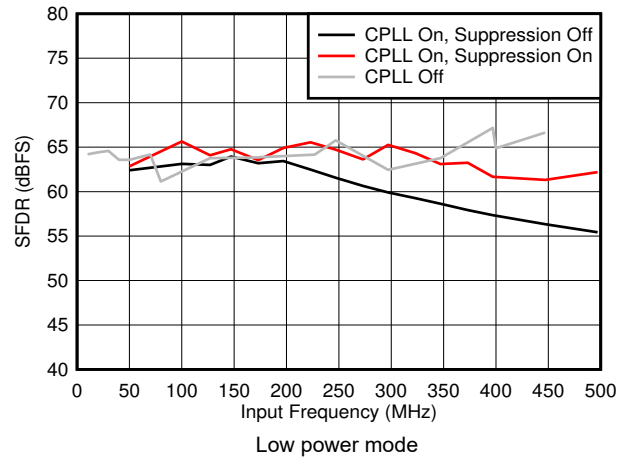
图 7-44. SFDR vs F_{IN} and C-PLL modes
