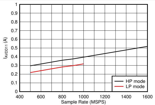
图 7-104. Single Channel, I_{VA11} vs F_S
