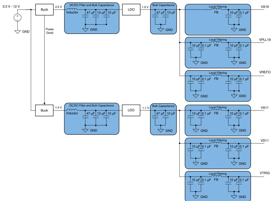
图 9-3. LDO Linear Regulator Approach Example
