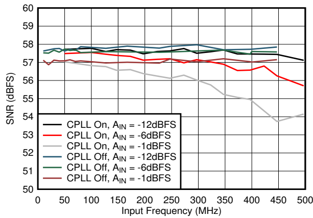
图 7-55. SNR vs A_{IN} and C-PLL
