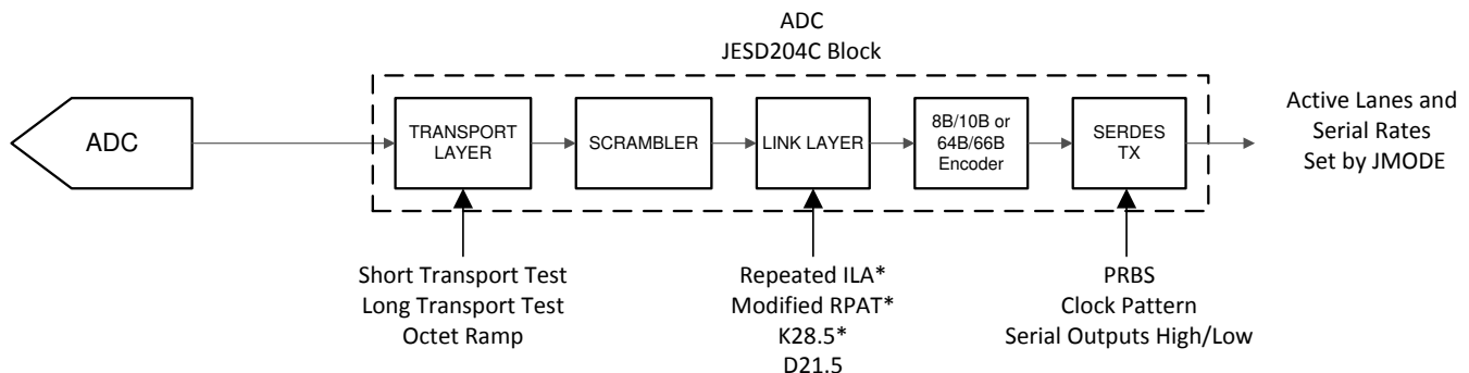
图 8-12. Test Mode Insertion Points
