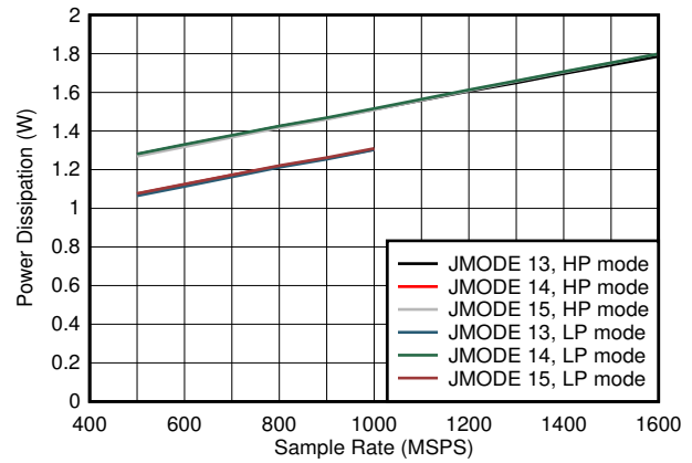
图 7-92. Dual Channel, Power Dissipation vs F_S and JMODE 13 - 15
