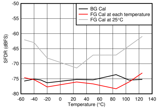
图 7-68. Worst Spur vs Temperature
