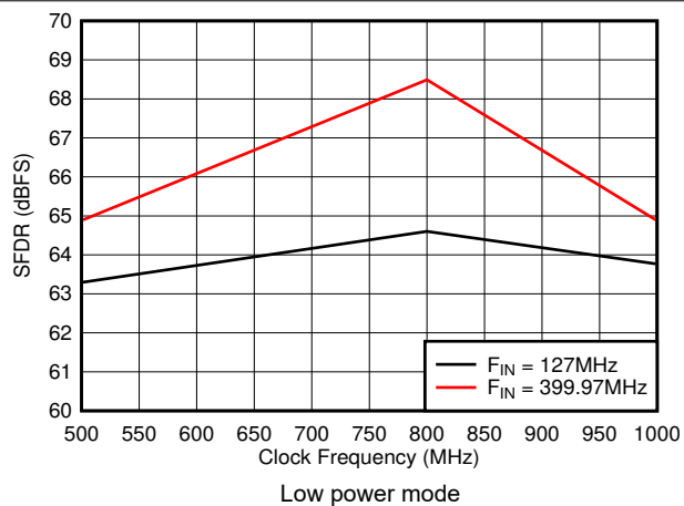
图 7-27. SFDR vs Sample Rate
