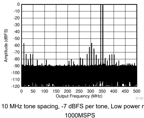
图 7-72. Two Tone FFT at 348 MHz
