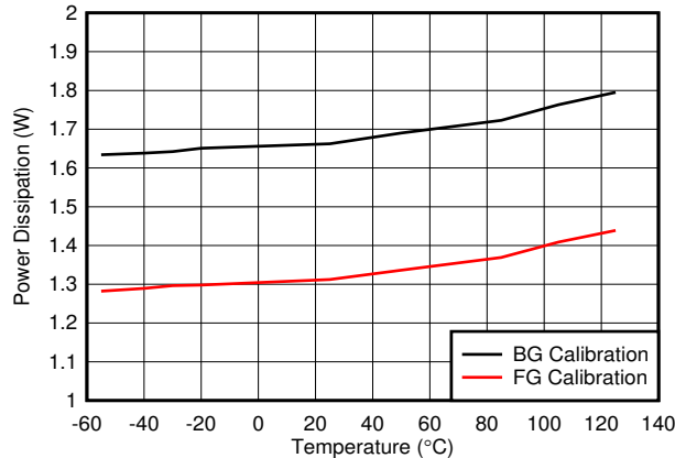
图 7-121. Quad Channel, Power Dissipation vs Temperature
