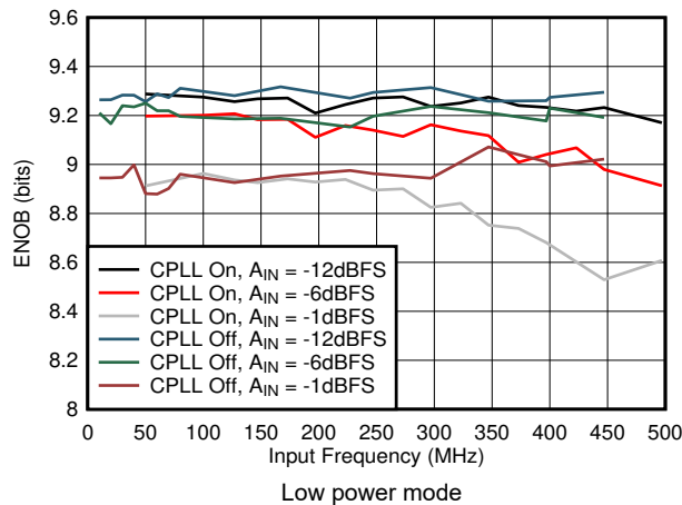
图 7-57. ENOB vs A_{IN} and C-PLL
