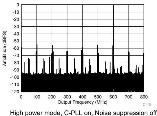
图 7-9. Single Tone FFT at 997 MHz and -1 dBFS
