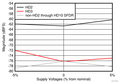
图 7-61. HD2, HD3 and Worst non-HD Spur vs Supply Voltage
