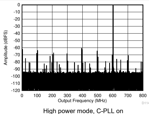
图 7-8. Single Tone FFT at 997 MHz and -1 dBFS
