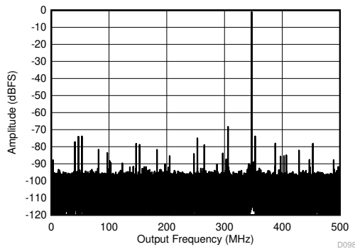
图 7-13. Single Tone FFT at 347 MHz and -1 dBFS
