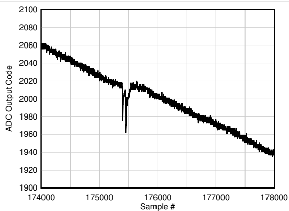
图 7-127. Background Calibration Core Transition (AC Signal Zoomed)
