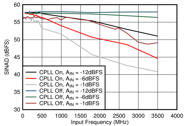
图 7-50. SINAD vs A_{IN} and C-PLL
