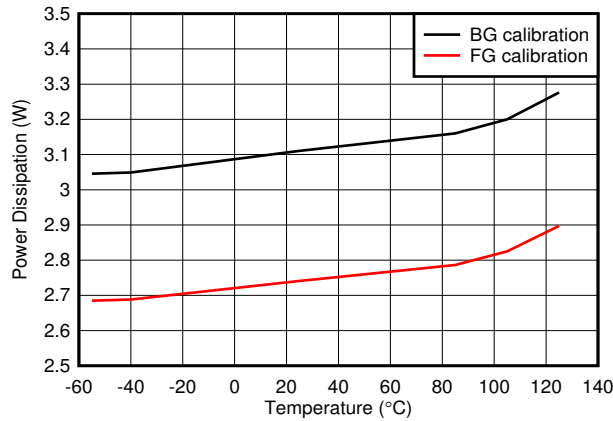
图 7-121. Quad Channel, Power Dissipation vs Temperature
