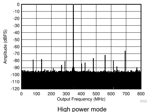
图 7-4. Single Tone FFT at 347 MHz and -1 dBFS
