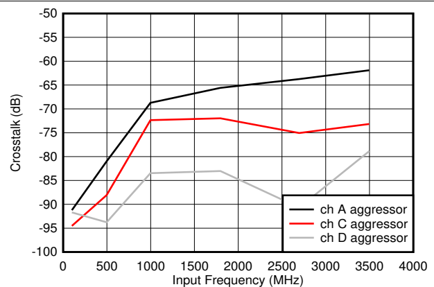
图 7-78. Crosstalk to Channel B vs F_{IN}
