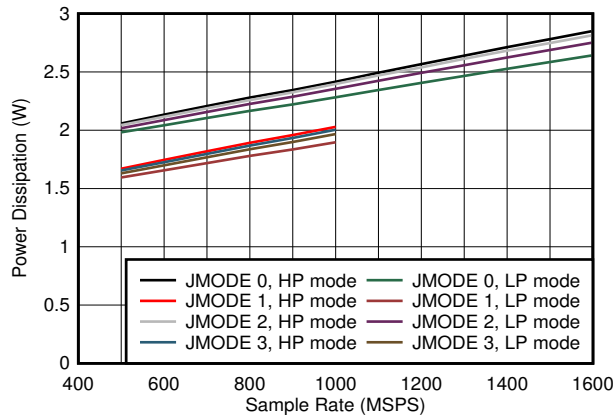
图 7-79. Quad Channel, Power Dissipation vs F_S and JMODES 0 - 3
