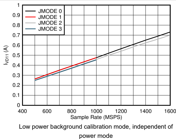
图 7-85. Quad Channel, I_{VD11} vs F_S and JMODE 0 - 3
