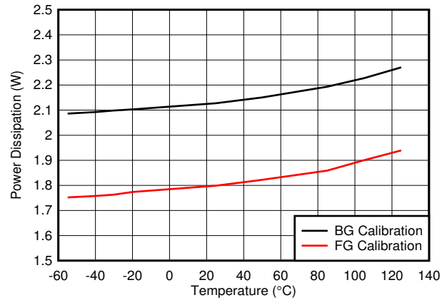
图 7-122. Dual Channel, Power Dissipation vs Temperature
