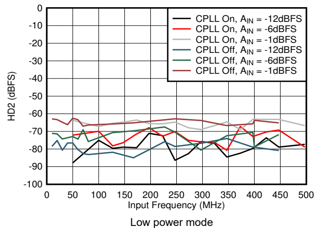
图 7-58. HD2 vs A_{IN} and C-PLL
