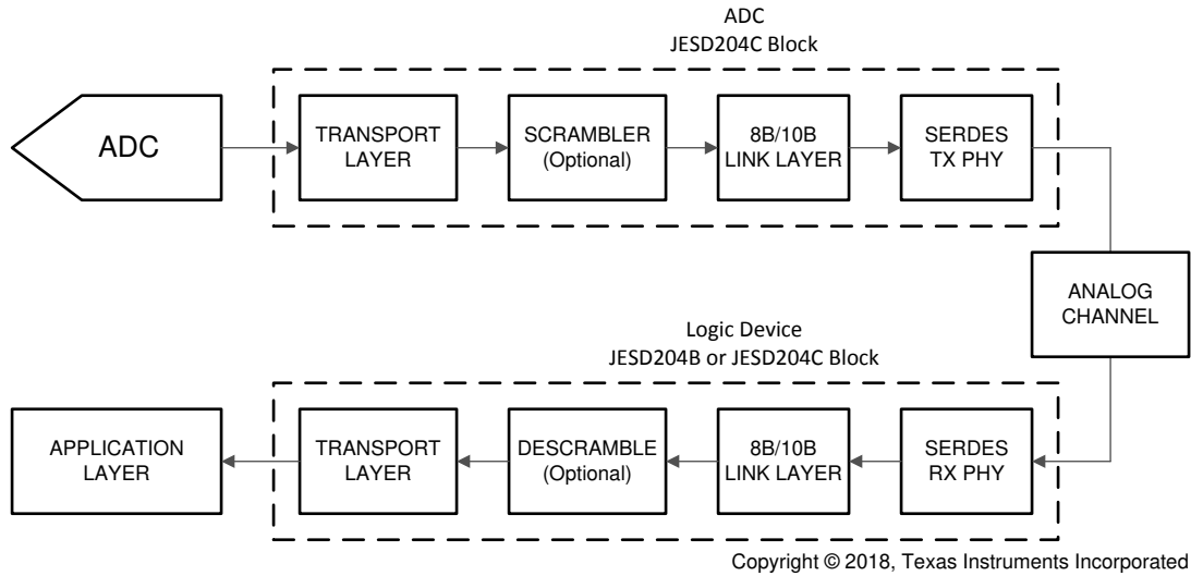
图 8-5. Simplified 8B/10B Encoded JESD204C Interface Diagram
