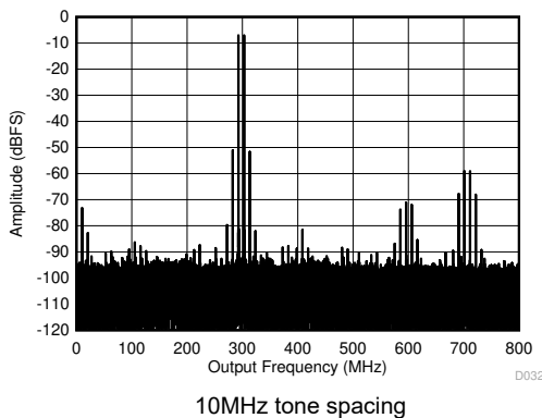
图 7-71. Two Tone FFT at 3498MHz
