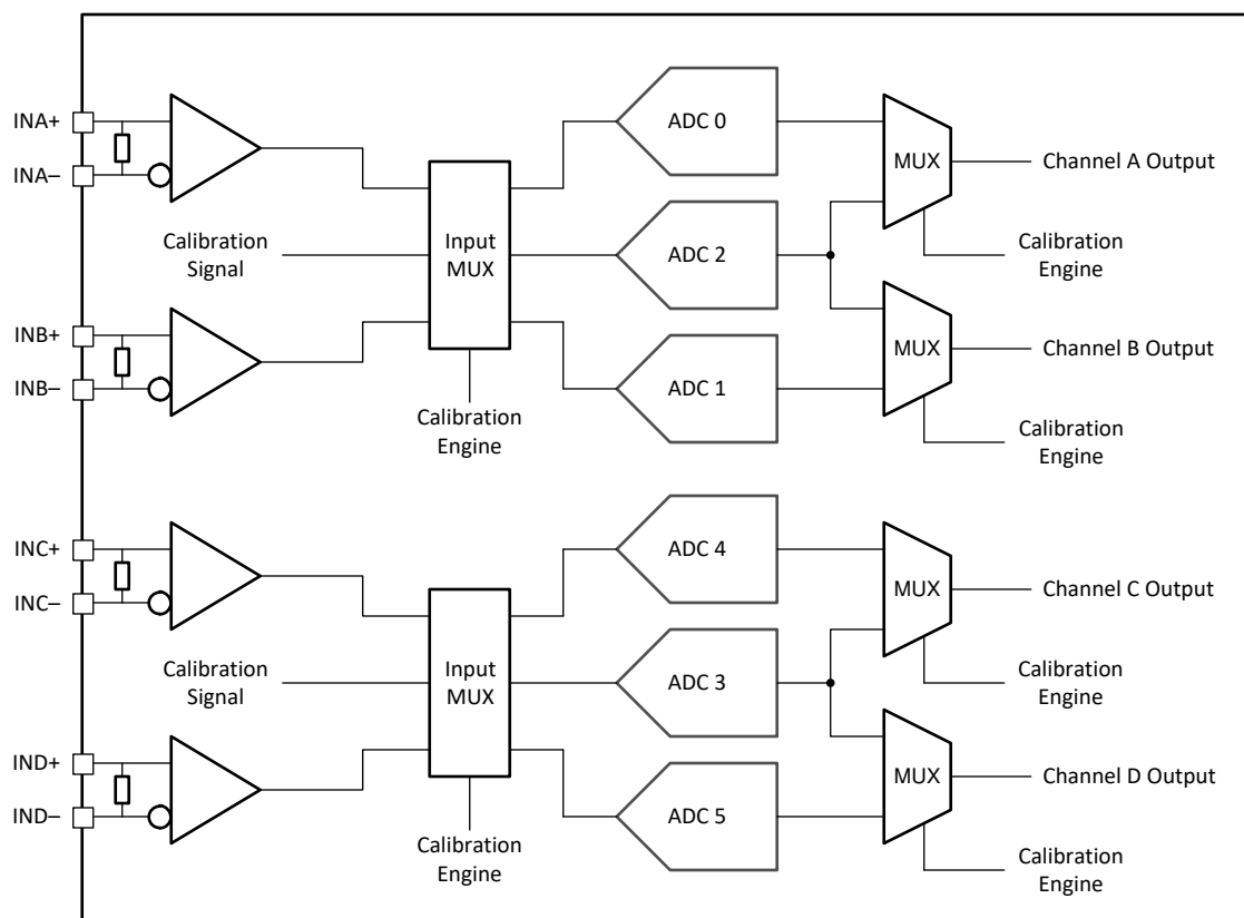
图 8-13. Quad Channel Calibration System Block Diagram
