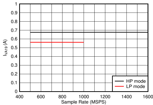
图 7-83. Quad Channel, I_{VA19} vs F_S
