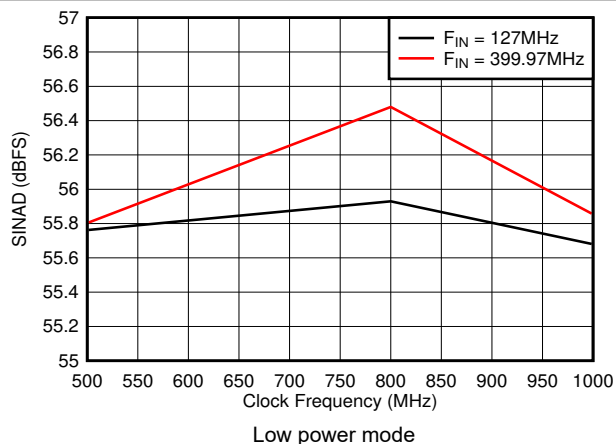
图 7-30. SINAD vs Sample Rate
