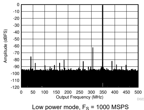
图 7-12. Single Tone FFT at 347 MHz and -1 dBFS
