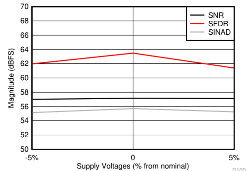
All supplies changed together, high power mode 图 7-60. SNR, SFDR and SINAD vs Supply Voltage
