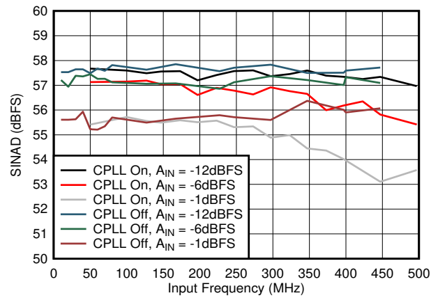
图 7-56. SINAD vs A_{IN} and C-PLL
