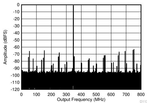
图 7-6. Single Tone FFT at 347 MHz and -1 dBFS
