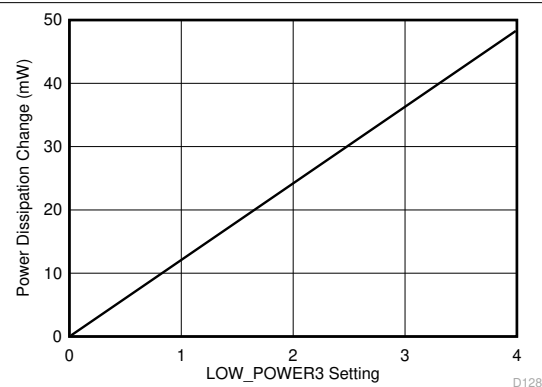
图 8-11. Power Dissipation Change vs LOW_POWER3 register setting
