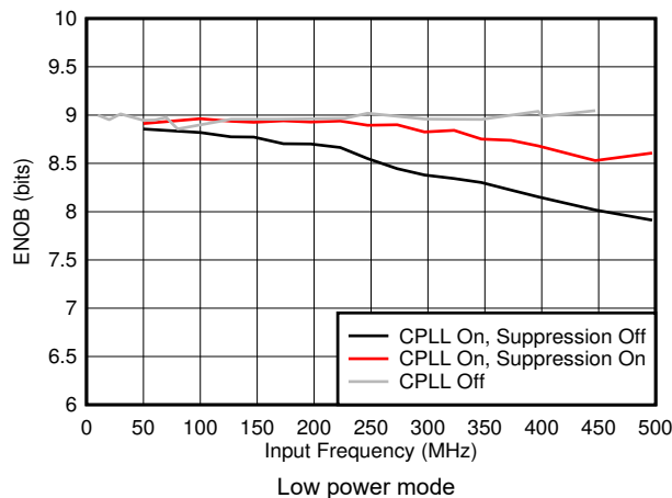
图 7-47. ENOB vs F_{IN} and C-PLL modes
