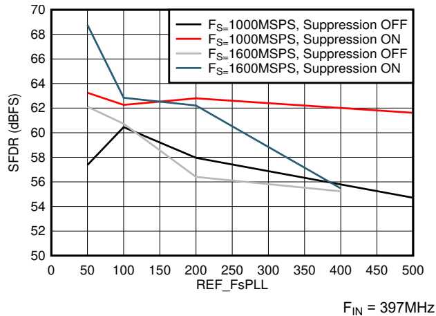
图 7-39. SFDR vs F_{REF} and Suppression
