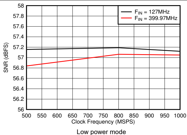
图 7-28. SNR vs Sample Rate
