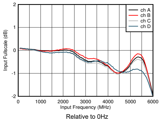
图 7-3. Input Fullscale vs Frequency
