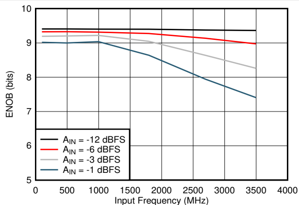
图 7-20. ENOB vs Input Frequency
