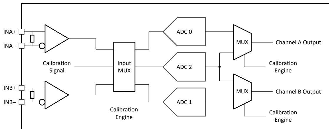
图 8-14. DualChannel Calibration System Block Diagram
