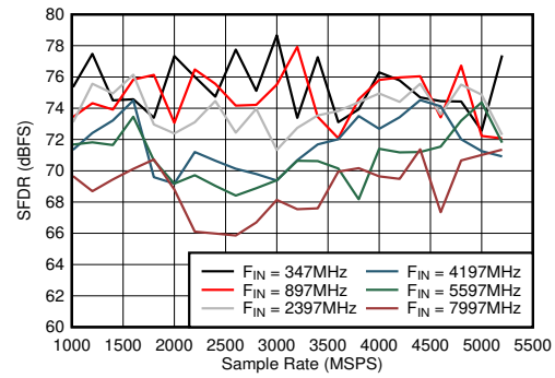
图 5-50. Dual Channel Mode: SFDR vs Sample Rate and Input Frequency
