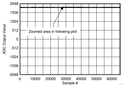
图 5-146. Background Calibration Core Transition (DC Signal)
