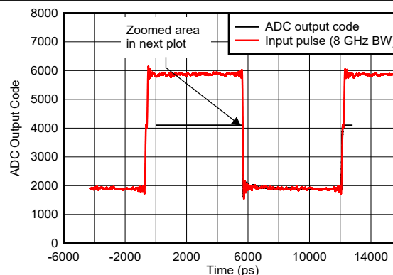
图 5-148. Pulse Overdrive Recovery
