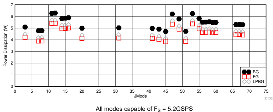
图 5-118. Dual Channel Mode: Power Dissipation vs JMODE at 5.2GSPS
