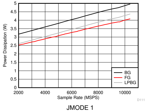
图 5-129. DES Mode: Power Dissipation vs Sample Rate
