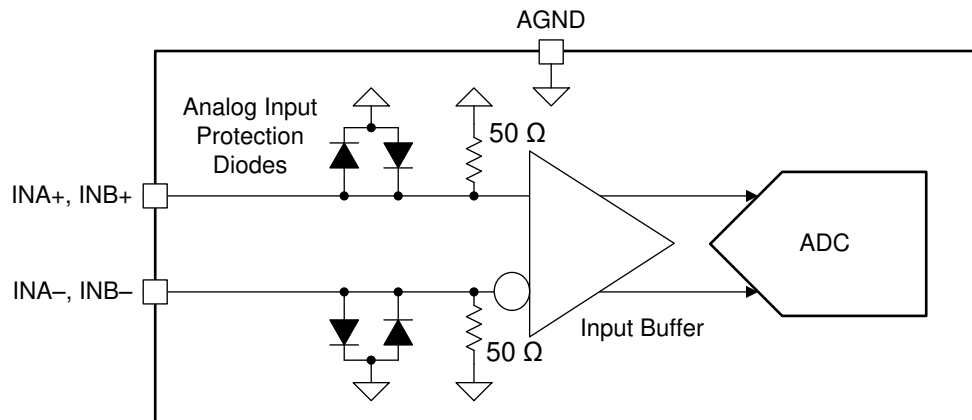
图 6-1. ADC12DJ5200-EP Analog Input Internal Termination and Protection Diagram
