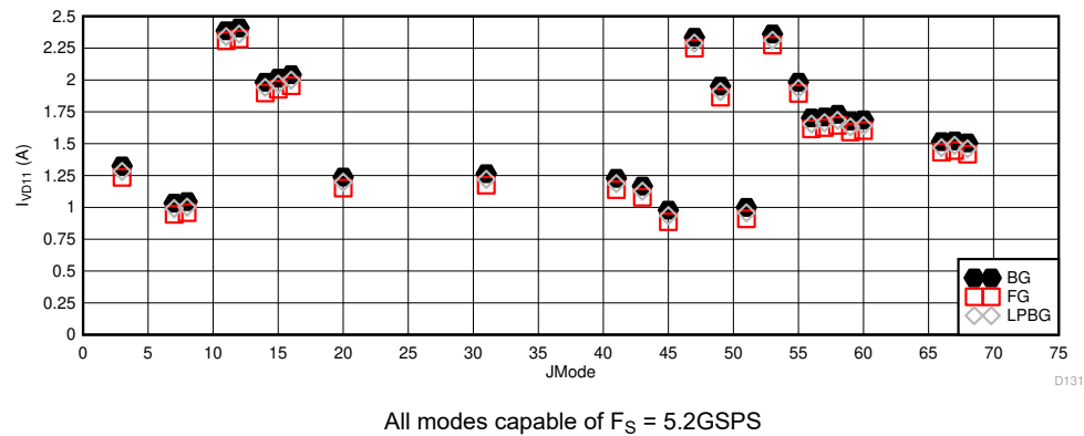
图 5-117. Dual Channel Mode: I_{VD11} vs JMODE at 5.2GSPS
