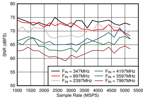
图 5-49. Dual Channel Mode: SNR vs Sample Rate and Input Frequency
