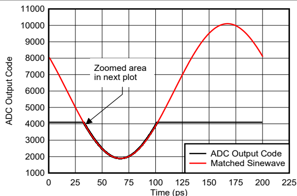
图 5-150. Sinewave Overdrive Recovery
