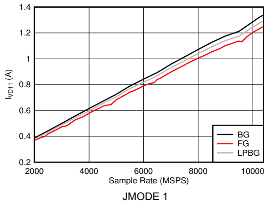
图 5-125. DES Mode: I_{VD11} vs Sample Rate
