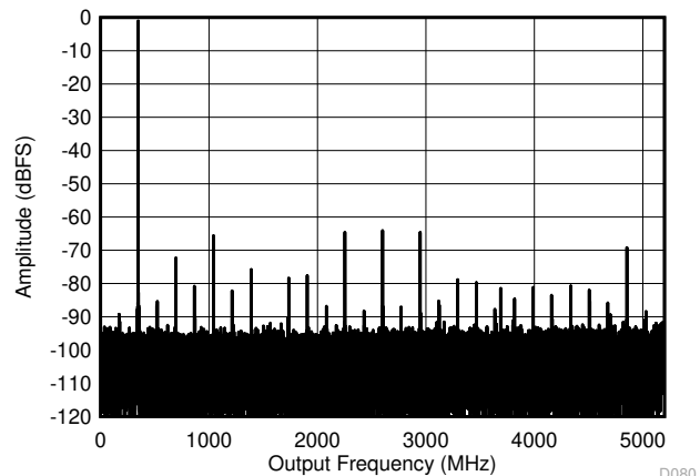
图 5-5. DES Mode: Single Tone FFT at 347 MHz
