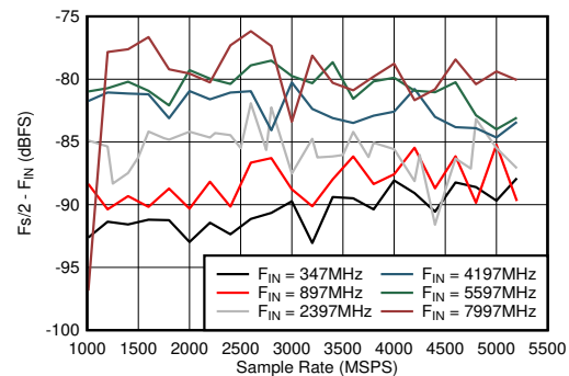
图 5-58. Dual Channel Mode: F_{\text{s}}/2 - F_{\text{IN}} vs Sample Rate and Input Frequency
