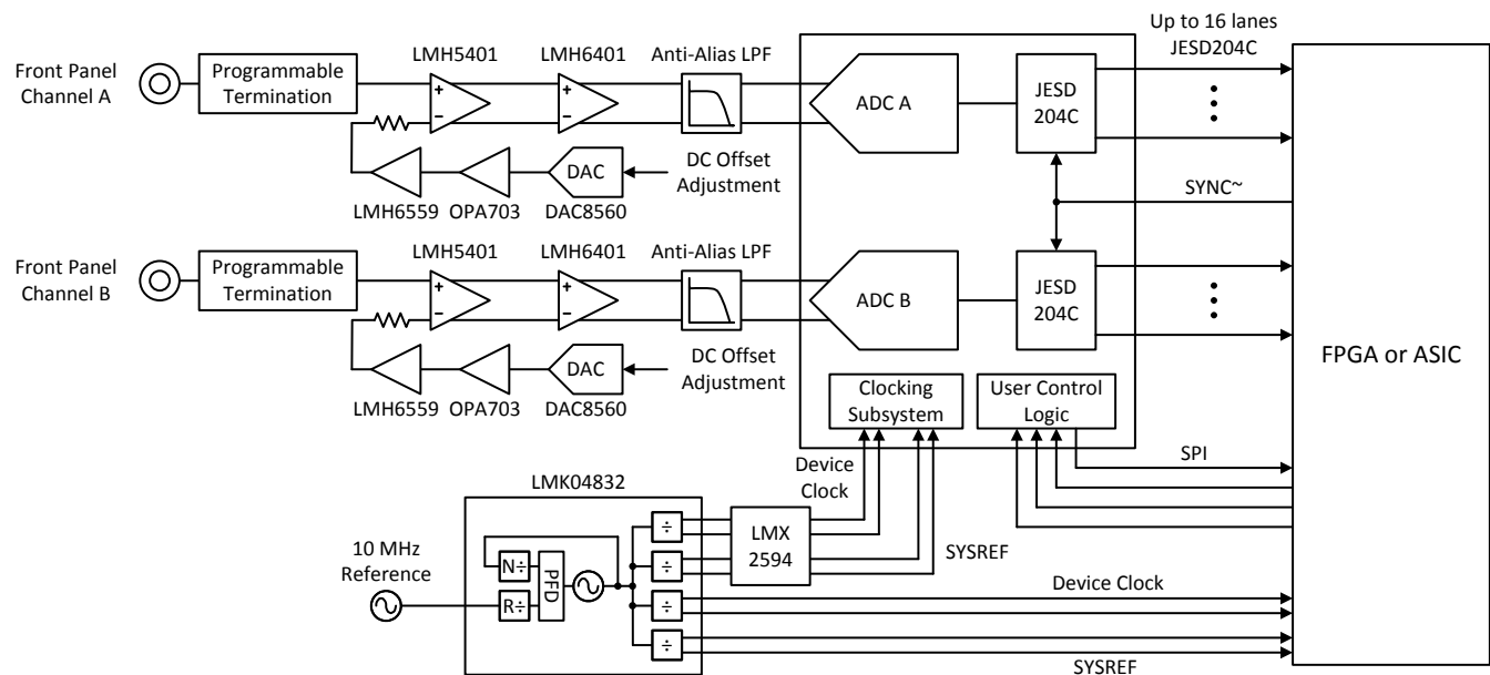
图 7-2. Typical Configuration for Reconfigurable Oscilloscope
