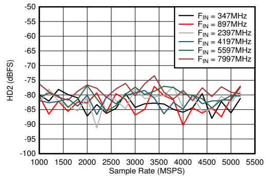
图 5-54. Dual Channel Mode: HD2 vs Sample Rate and Input Frequency
