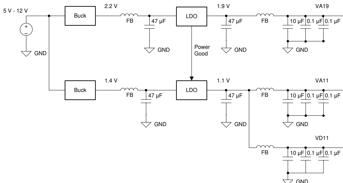
图 7-3. LDO Linear Regulator Approach Example
