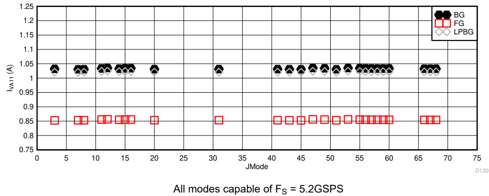
图 5-116. Dual Channel Mode: I_{VA11} vs JMODE at 5.2GSPS
