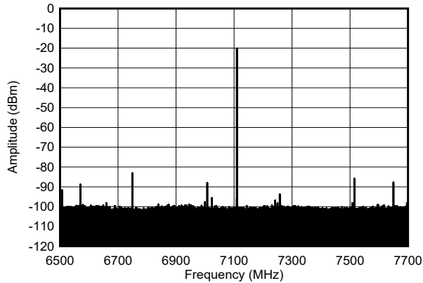
图 6-582. Single Tone Output Spectrum at 7.1 GHz, -12 dBFS (narrow span)
