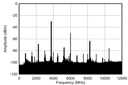
图 6-493. TX Dual Tone Output Spectrum at 3.75 GHz, -13 dBFS each ( 0 - f_{\text{DAC}} )
