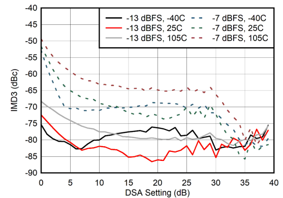
图 6-290. IMD3 vs DSA Setting at 400 MHz
