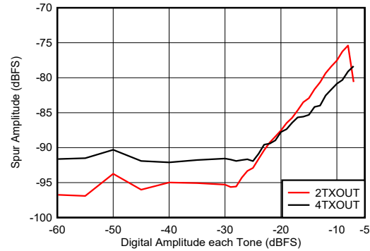
图 6-471. Two Tone Inband SFDR vs Digital Amplitude at 3.75 GHz
