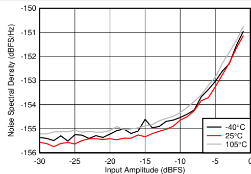
图 6-116. RX Noise Spectral Density vs Input Amplitude and Temperature at 2.6 GHz
