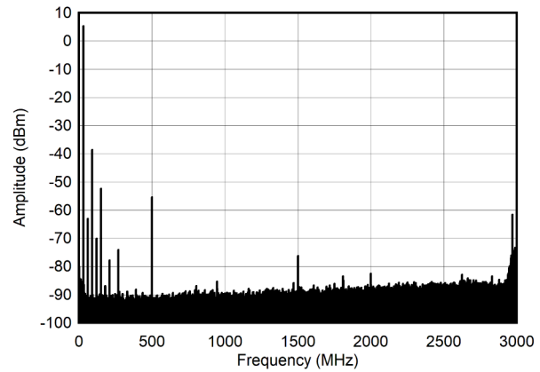
图 6-240. Single Tone Spectrum at 30 MHz and -1 dBFS (Nyquist)
