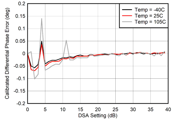
图 6-266. Calibrated TX Differential Phase Error (DNL) at 400 MHz
