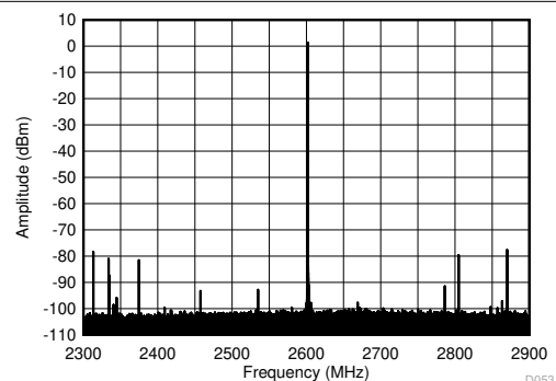
图 6-419. TX Single Tone ( - 6 dBFS) Output Spectrum at 2.6 GHz ( \pm 300 MHz)
