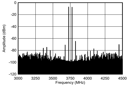
图 6-492. TX Dual Tone Output Spectrum at 3.75 GHz, -7 dBFS each ( \pm 600 MHz)
