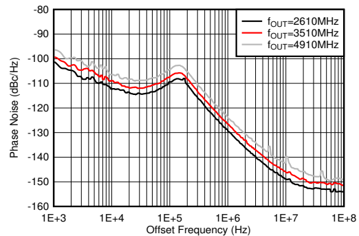
图 6-617. Phase Noise for 9-GHz VCO vs Offset Frequency and f_{OUT} at 25°C
