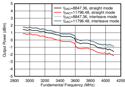
图 6-445. TX Output Power vs Frequency
