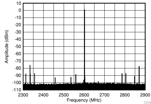
图 6-427. TX Single Tone ( - 1 dBFS) Output Spectrum at 2.6 GHz ( \pm 300 MHz)
