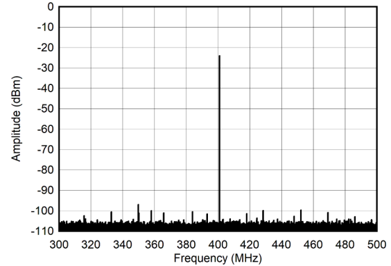
图 6-276. Single Tone Spectrum at 400 MHz and -30 dBFS (±100MHz)
