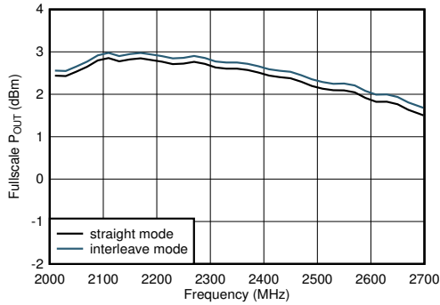
图 6-374. TX Full Scale vs RF Frequency at 5898.24 MSPS
