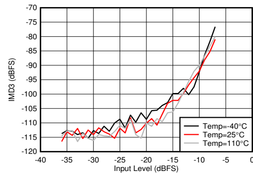
图 6-120. RX IMD3 vs Input Level and Temperature at 2.6 GHz
