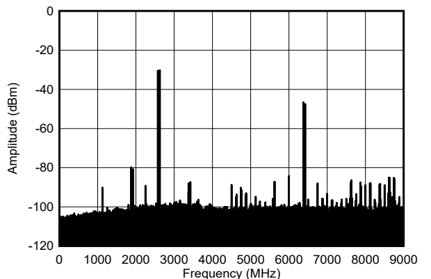
图 6-432. TX Dual Tone Output Spectrum at 2.6 GHz, -30 dBFS each (0 - DAC)
