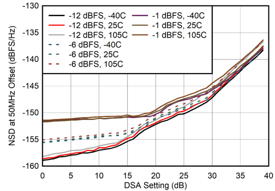
图 6-288. Noise Spectral Density vs DSA Setting at 400 MHz
