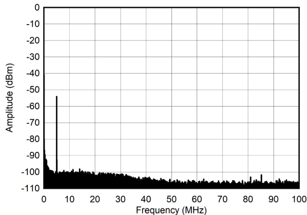
图 6-239. Single Tone Spectrum at 5 MHz and -60 dBFS (0 - 100 MHz)
