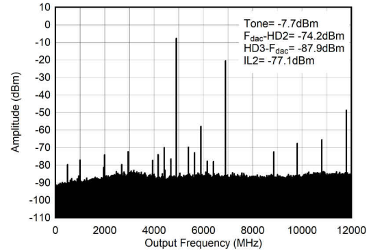
图 6-539. TX Single Tone ( - 6 dBFS) Output Spectrum at 4.9 GHz ( 0-f_{\text{DAC}} )
