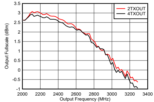
图 6-375. TX Full Scale vs RF Frequency at 8847.36 MSPS
