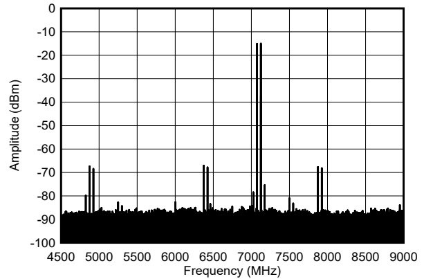
图 6-581. Single Tone Output Spectrum at 7.1 GHz, -12 dBFS (Nyquist)
