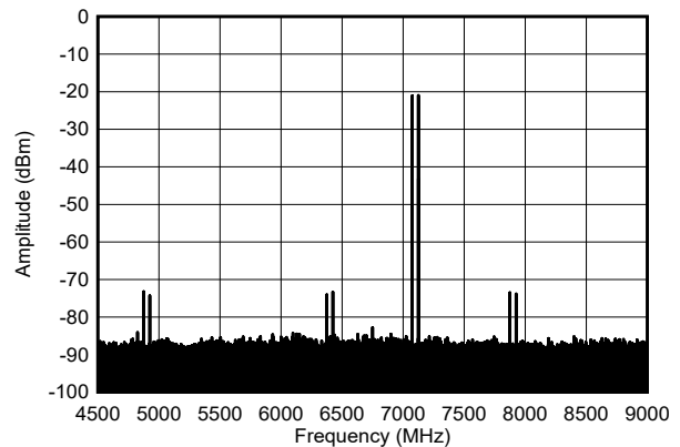
图 6-583. Two Tone Output Spectrum at 7.1 GHz, -7 dBFS each (Nyquist)
