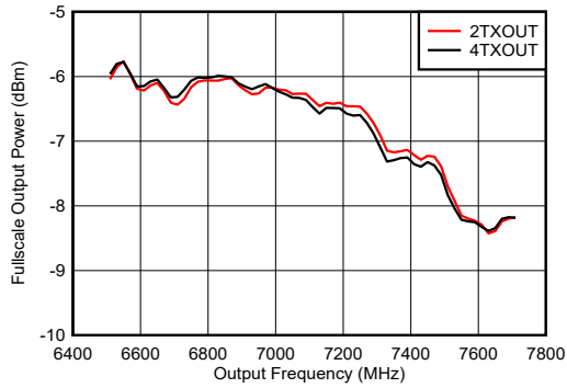
图 6-544. TX Full Scale vs RF Frequency and Channel
