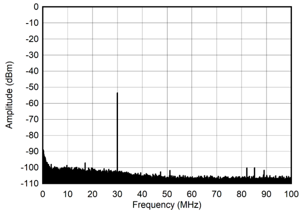
图 6-249. Single Tone Spectrum at 30 MHz and -60 dBFS (0 - 100 MHz)
