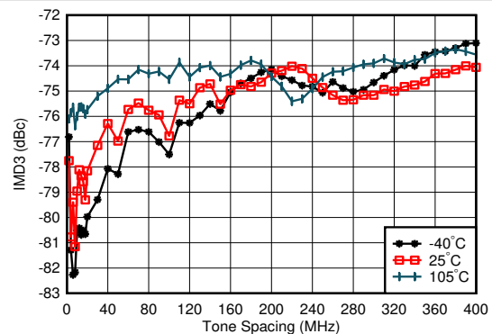
图 6-322. TX IMD3 vs Tone Spacing and Temperature at 0.85 GHz
