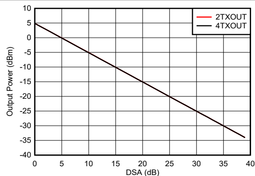
图 6-300. TX Output Power vs DSA Setting and Channel at 0.85 GHz
