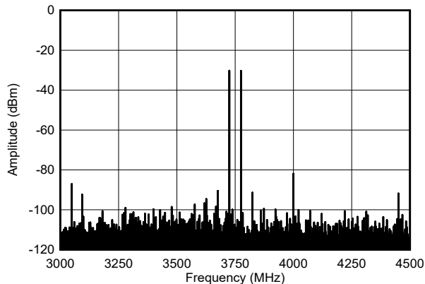
图 6-494. TX Dual Tone Output Spectrum at 3.75 GHz, -13 dBFS each ( \pm 600 MHz)
