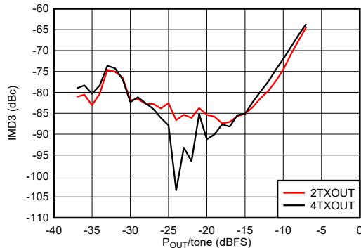
图 6-325. TX IMD3 vs Digital Level at 0.85 GHz
