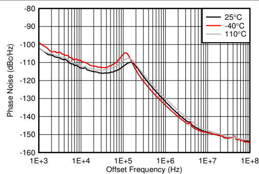
图 6-621. Phase Noise for 8-GHz VCO vs Offset Frequency and Temperature at f_{OUT} = 1910 MHz
