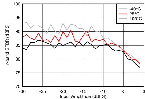
图 6-132. RX In-Band SFDR ( \pm 300\text{ MHz} ) vs Input Amplitude and Temperature at 2.6 GHz
