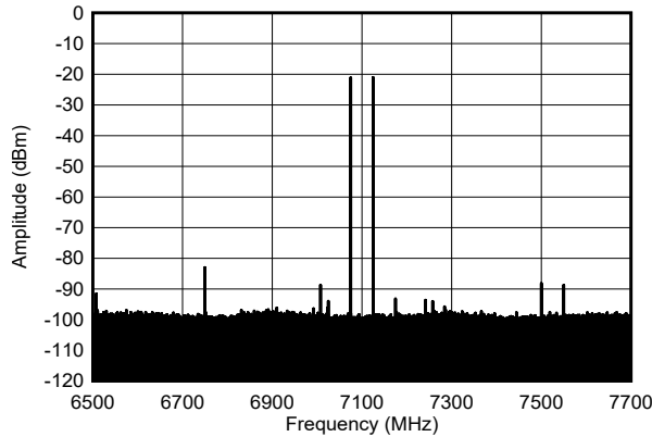
图 6-586. Two Tone Output Spectrum at 7.1 GHz, -13 dBFS each (narrow span)
