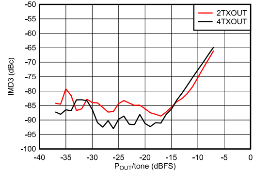
图 6-326. TX IMD3 vs Digital Level at 0.85 GHz
