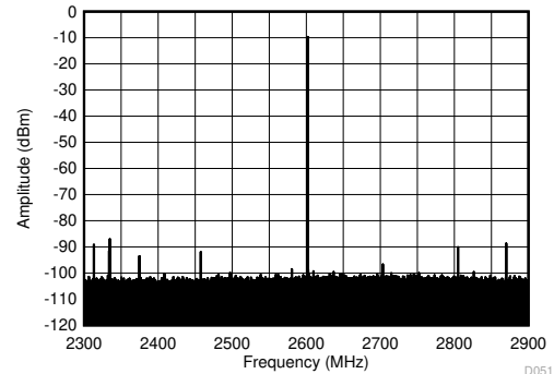
图 6-417. TX Single Tone ( - 12 dBFS) Output Spectrum at 2.6 GHz ( \pm 300 MHz)
