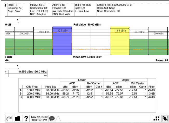
图 6-474. TX 2 carrier 100-MHz NR Output Spectrum at 3.45 GHz and 3.75 GHz
