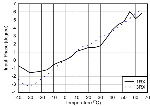
图 6-52. RX Input Phase vs Temperature and DSA at f_{\text{OUT}} = 0.8\text{ GHz}
