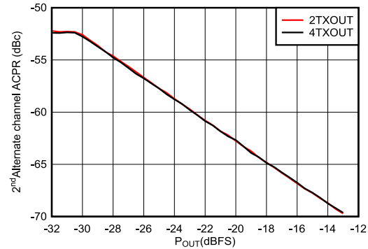
图 6-332. TX 20-MHz LTE alt2-ACPR vs Digital Level at 0.85 GHz
