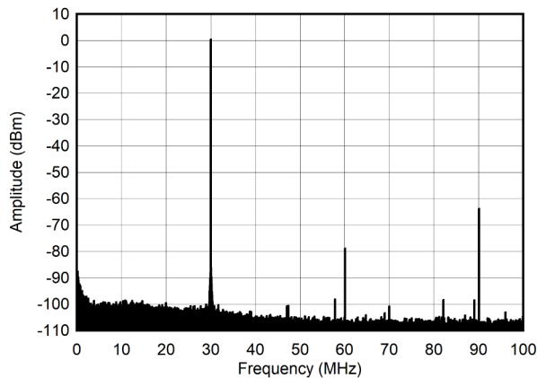
图 6-243. Single Tone Spectrum at 30 MHz and -6 dBFS (0 - 100 MHz)
