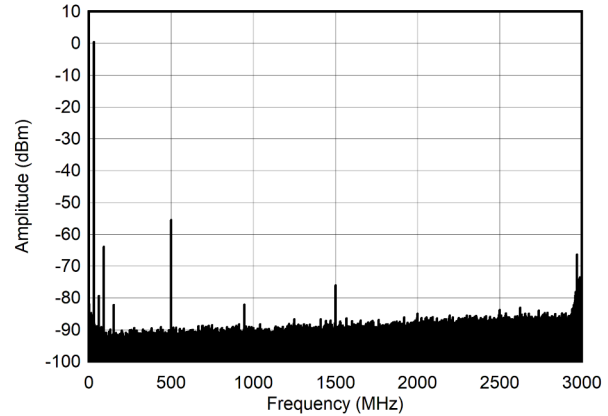
图 6-242. Single Tone Spectrum at 30 MHz and -6 dBFS (Nyquist)
