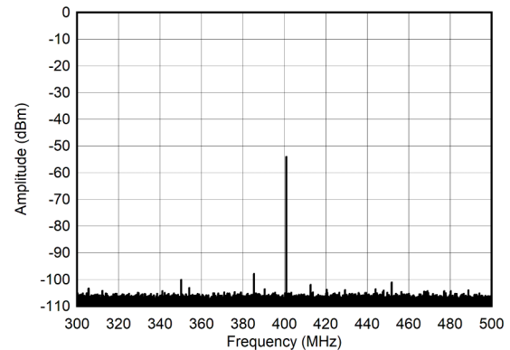
图 6-278. Single Tone Spectrum at 400 MHz and -60 dBFS (±100MHz)
