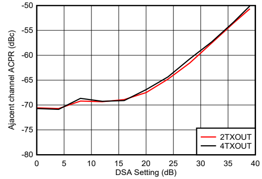
图 6-475. TX 20-MHz LTE ACPR vs DSA Setting at 3.5 GHz
