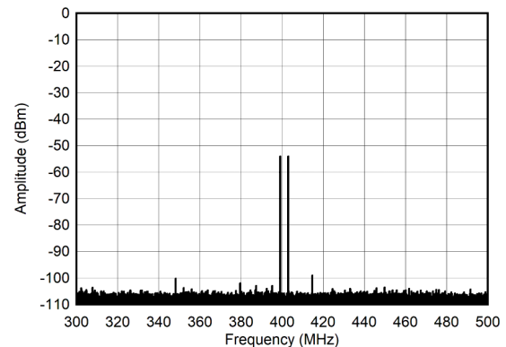
图 6-286. Dual Tone Spectrum at 400 MHz and -60 dBFS (±100MHz)
