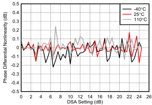
图 6-208. RX Calibrated Differential Phase Error at 6.851 GHz
