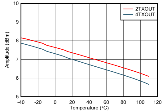
图 6-224. TX Output Fullscale vs Temperature at 30 MHz
