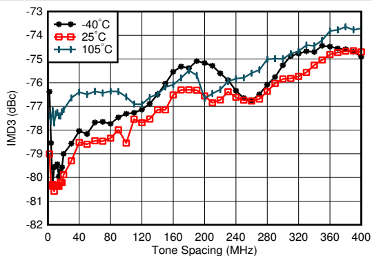
图 6-321. TX IMD3 vs Tone Spacing and Channel at 0.85 GHz
