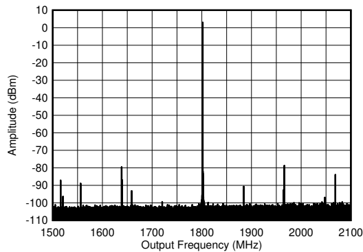
图 6-365. TX Single Tone ( - 6 dBFS) Output Spectrum at 1.8 GHz ( \pm 300\text{ MHz} )
