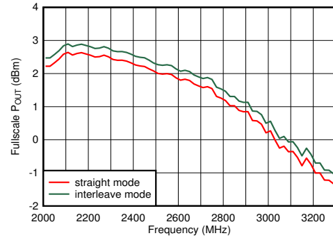
图 6-375. TX Full Scale vs RF Frequency at 8847.36 MSPS
