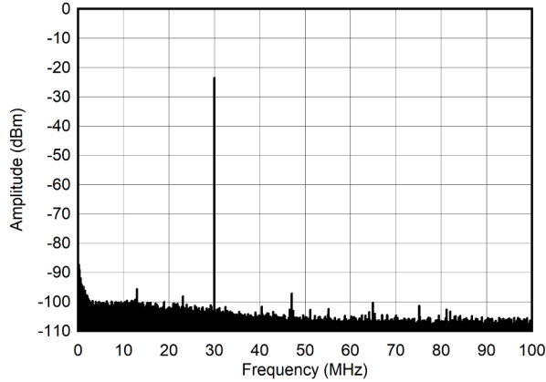
图 6-247. Single Tone Spectrum at 30 MHz and -30 dBFS (0 - 100 MHz)
