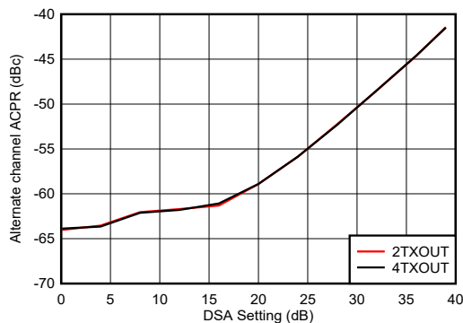
图 6-476. TX 20-MHz LTE alt-ACPR vs DSA Setting at 3.5 GHz
