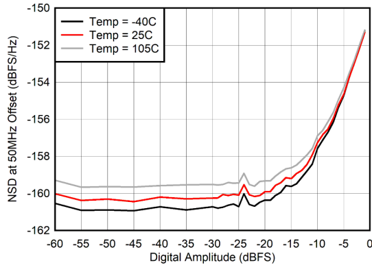
图 6-287. Noise Spectral Density vs Digital Amplitude at 400 MHz
