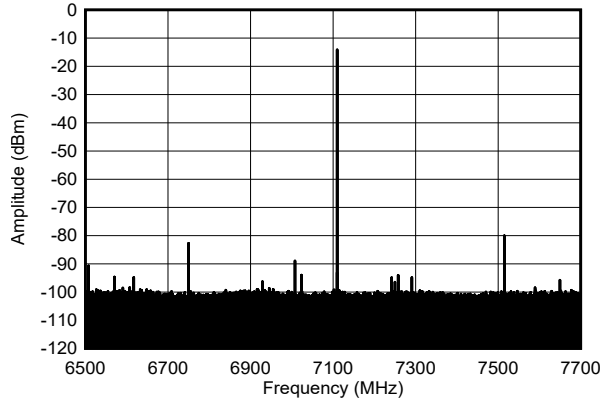
图 6-580. Single Tone Output Spectrum at 7.1 GHz, -6 dBFS (narrow span)
