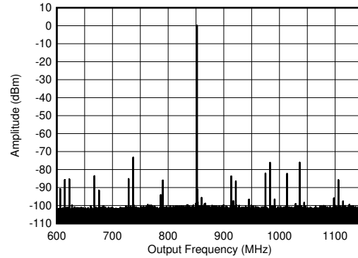
图 6-344. TX Single Tone ( - 6 dBFS) Output Spectrum at 0.85 GHz ( \pm 300 MHz)
