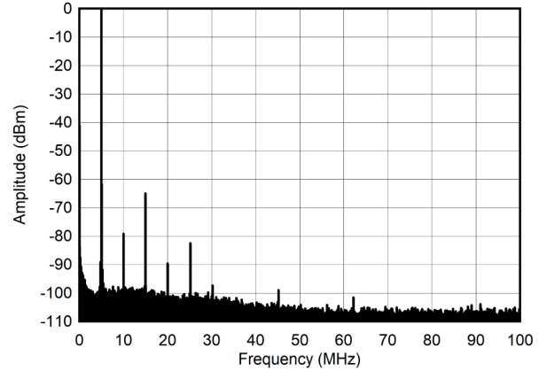
图 6-236. Single Tone Spectrum at 5 MHz and -6 dBFS (0 - 100 MHz)
