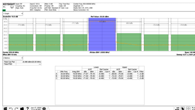
图 6-329. TX 20-MHz LTE Output Spectrum at 0.85 GHz
