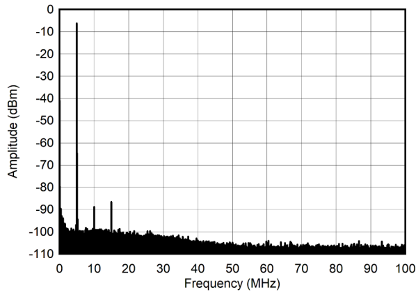
图 6-237. Single Tone Spectrum at 5 MHz and -12 dBFS (0 - 100 MHz)
