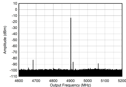
图 6-542. TX Single Tone ( - 12 dBFS) Output Spectrum at 4.9 GHz ( \pm 300 MHz)
