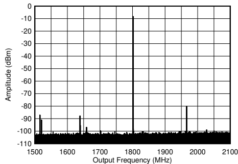
图 6-367. TX Single Tone ( - 1 dBFS) Output Spectrum at 1.8 GHz ( \pm 300\text{ MHz} )
