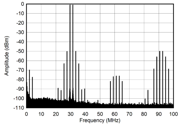
图 6-250. Dual Tone Spectrum at 30 MHz and -7 dBFS (0 - 100 MHz)
