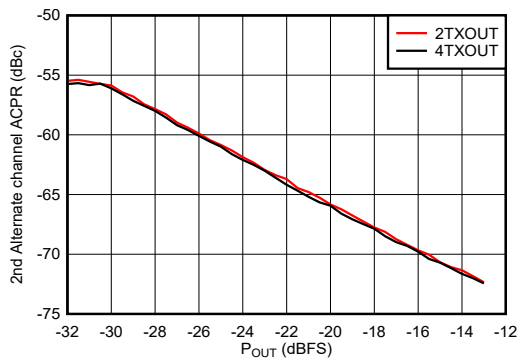
图 6-357. TX 20-MHz LTE alt2-ACPR vs Digital Level at 1.8425 GHz
