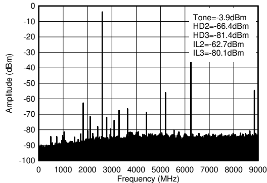
图 6-422. TX Single Tone ( - 12 dBFS) Output Spectrum at 2.6 GHz ( 0-f_{\text{DAC}} )
