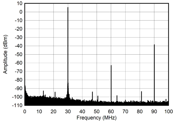
图 6-241. Single Tone Spectrum at 30 MHz and -1 dBFS (0 - 100 MHz)
