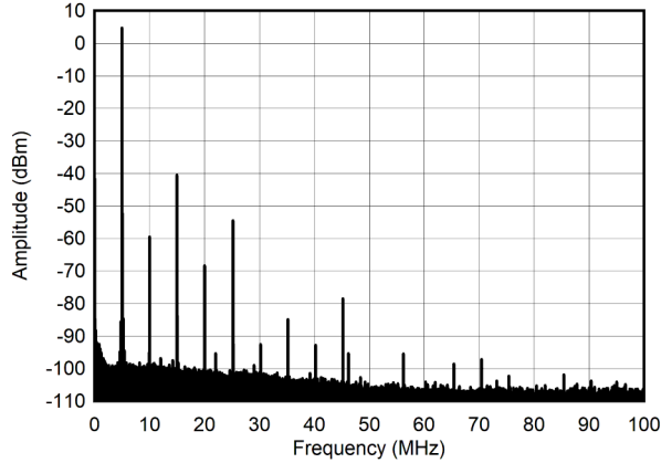
图 6-235. Single Tone Spectrum at 5 MHz and -1 dBFS (0 - 100 MHz)
