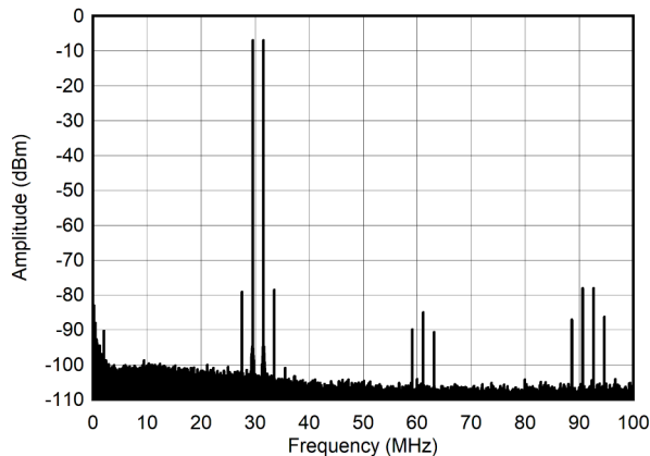
图 6-251. Dual Tone Spectrum at 30 MHz and -13 dBFS (0 - 100 MHz)
