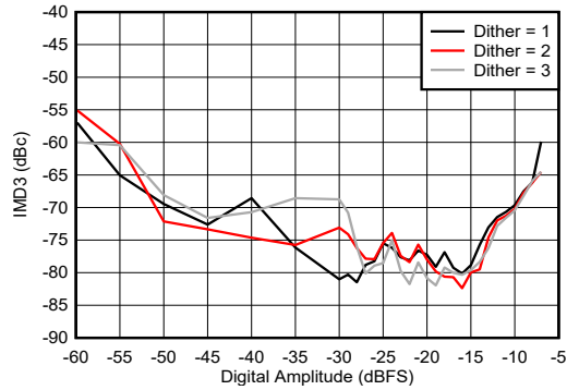
图 6-470. TX IMD3 vs Digital Amplitude and Dither at 3.75 GHz
