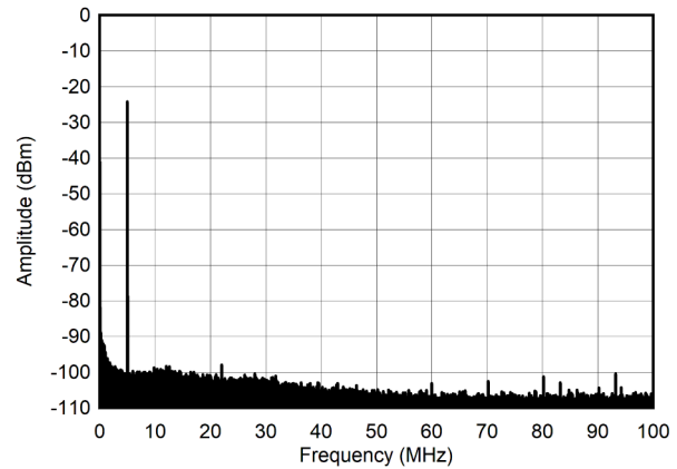
图 6-238. Single Tone Spectrum at 5 MHz and -30 dBFS (0 - 100 MHz)
