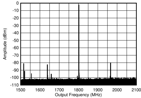
图 6-371. TX Single Tone ( - 6 dBFS) Output Spectrum at 1.8 GHz (±300 MHz)
