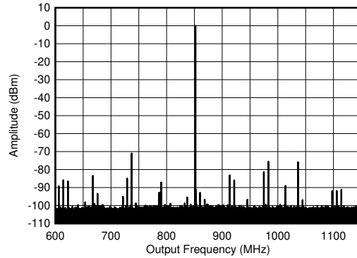
图 6-350. TX Single Tone ( - 6 dBFS) Output Spectrum at 0.85 GHz ( \pm 300 MHz)
