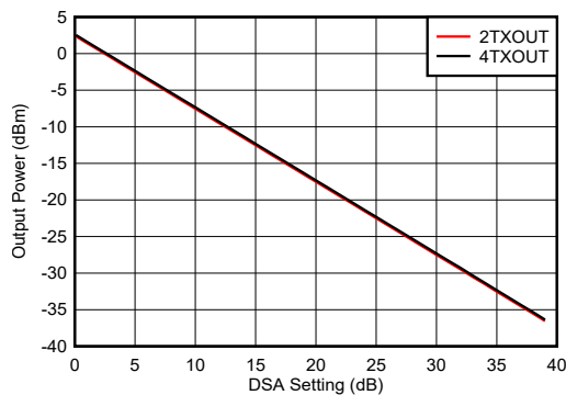
图 6-378. TX Output Power vs DSA Setting and Channel at 2.6 GHz
