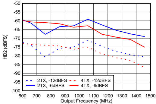
图 6-337. TX HD2 vs Digital Amplitude and Output Frequency at 0.85 GHz
