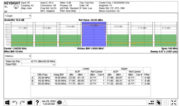
图 6-354. TX 20-MHz LTE Output Spectrum at 1.8425 GHz
