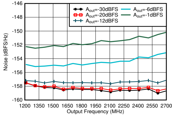
图 6-353. TX Single Tone Output Noise vs Frequency and Amplitude at 1.8 GHz
