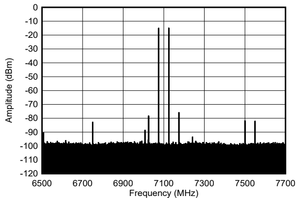
图 6-584. Two Tone Output Spectrum at 7.1 GHz, -7 dBFS each (narrow band)
