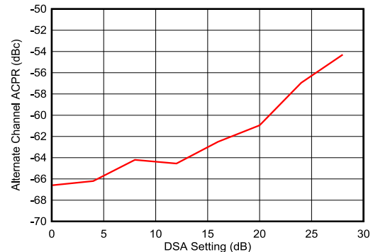
图 6-334. TX 20-MHz LTE alt-ACPR vs DSA at 0.85 GHz
