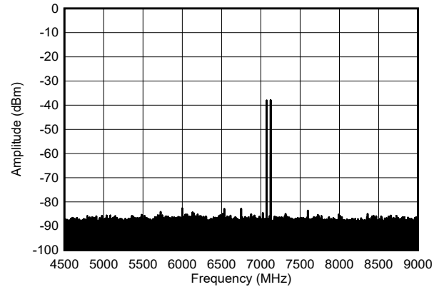
图 6-587. Two Tone Output Spectrum at 7.1 GHz, -30 dBFS each (Nyquist)
