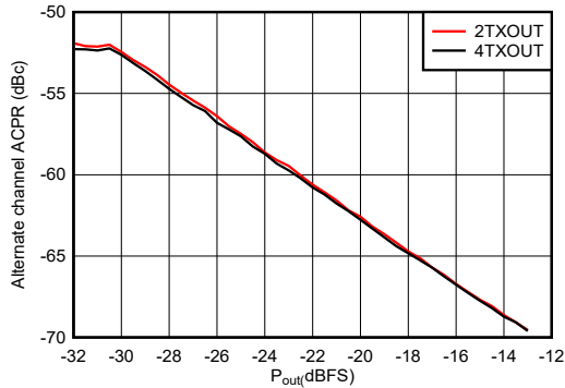
图 6-331. TX 20-MHz LTE alt-ACPR vs Digital Level at 0.85 GHz
