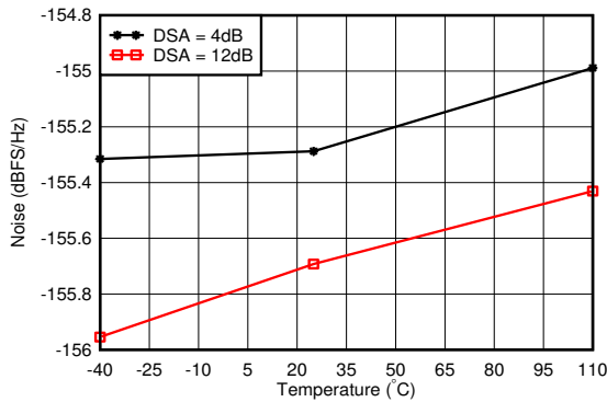
图 6-185. RX Noise Spectral Density vs Temperature at 4.9 GHz
