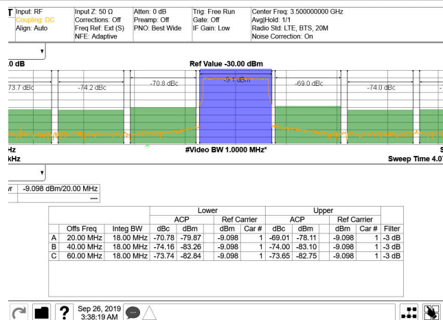
图 6-472. TX 20-MHz LTE Output Spectrum at 3.5 GHz (Band 42)
