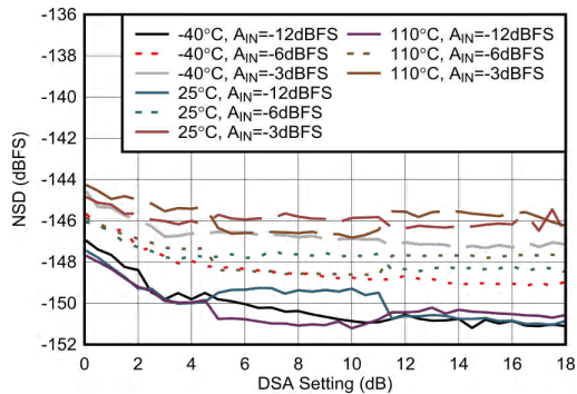
图 6-220. RX NSD vs DSA Setting at 6.851 GHz
