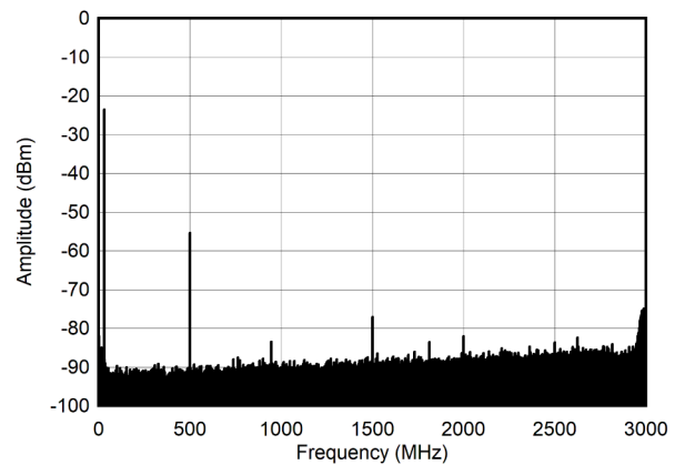
图 6-246. Single Tone Spectrum at 30 MHz and -30 dBFS (Nyquist)
