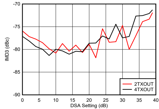
图 6-521. TX IMD3 vs DSA Setting at 4.9 GHz
