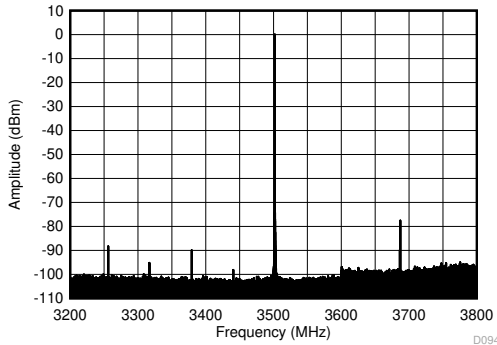
图 6-486. TX Single Tone ( - 1 dBFS) Output Spectrum at 3.5 GHz ( \pm 300 MHz)
