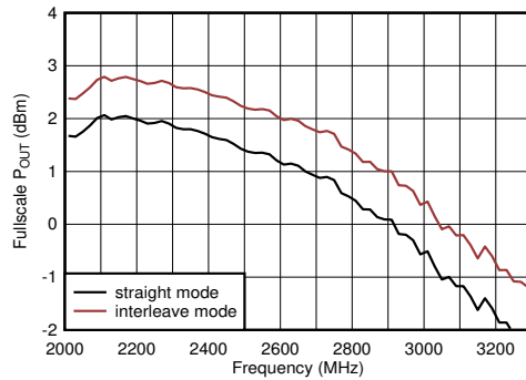
图 6-374. TX Full Scale vs RF Frequency at 5898.24 MSPS
