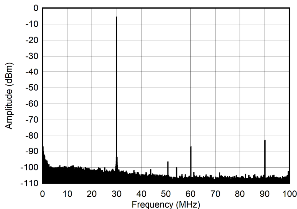
图 6-245. Single Tone Spectrum at 30 MHz and -12 dBFS (0 - 100 MHz)
