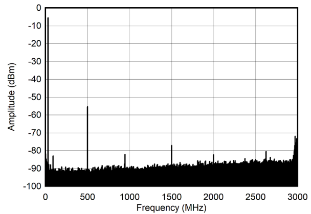
图 6-244. Single Tone Spectrum at 30 MHz and -12 dBFS (Nyquist)
