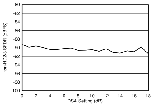
图 6-133. RX Non-HD2/3 vs DSA Setting at 2.6 GHz
