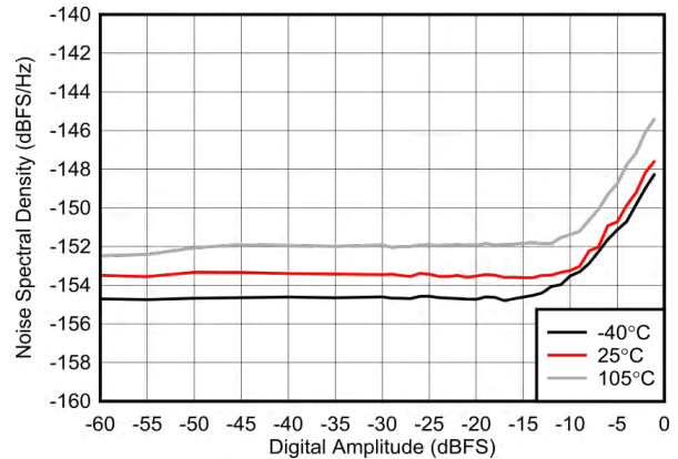
图 6-575. NSD vs Digital Amplitude and Temperature at 7.1 GHz
