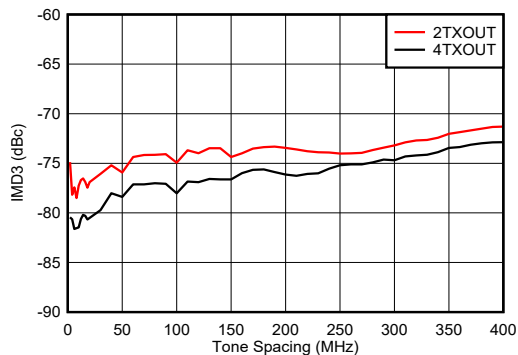
图 6-319. TX IMD3 vs Tone Spacing and Channel at 0.85 GHz
