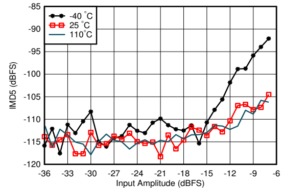
图 6-69. RX IMD5 vs Input Level and Temperature at 0.8 GHz
