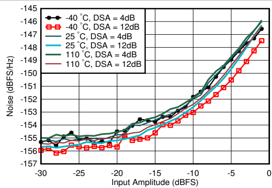
图 6-186. RX Noise Spectral Density vs Input Amplitude and Temperature at 4.9 GHz
