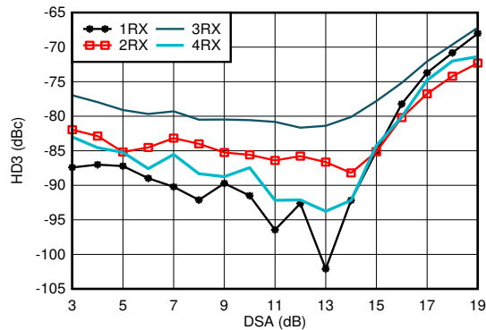
图 6-103. RX HD3 vs DSA Setting and Channel at 1.9 GHz
