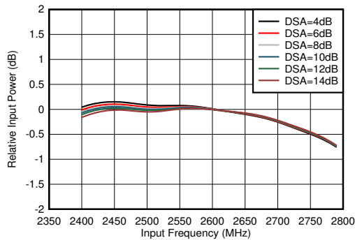
图 6-111. RX Inband Gain Flatness, f_{\text{IN}} = 2600\text{ MHz}
