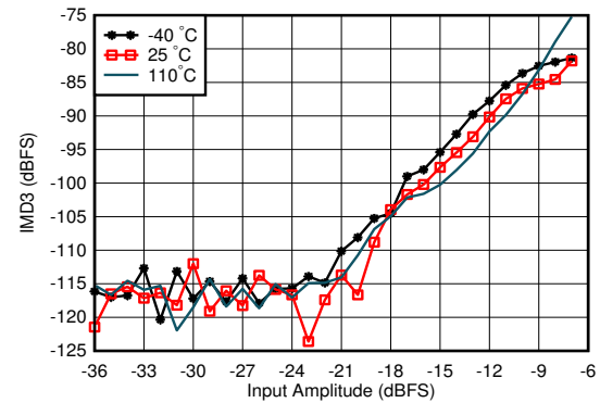
图 6-190. RX IMD3 vs Input Level and Temperature at 4.9 GHz
