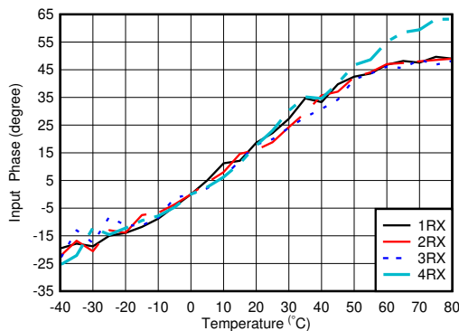
图 6-175. RX Input Phase vs Temperature and DSA at f_{\text{OUT}} = 4.9\text{ GHz}
