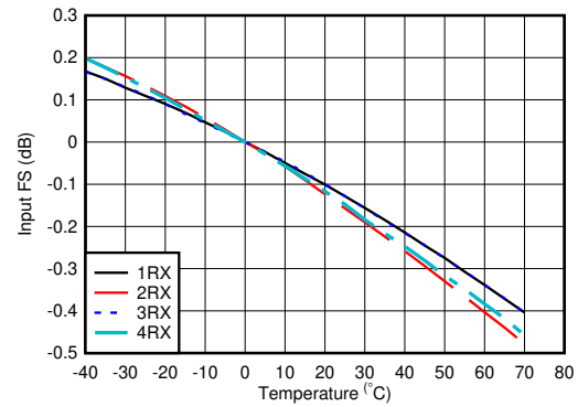
图 6-82. RX Input Fullscale vs Temperature and Channel at 1.75 GHz
