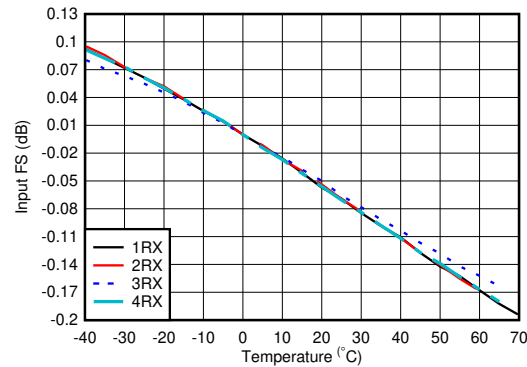
图 6-51. RX Input Fullscale vs Temperature and Channel at 800MHz
