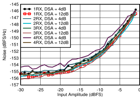
图 6-187. RX Noise Spectral Density vs Input Amplitude and Channel at 4.9 GHz
