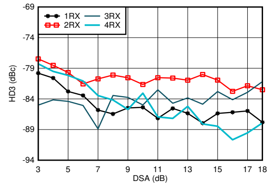
图 6-73. RX HD3 vs DSA Setting and Channel at 0.8 GHz
