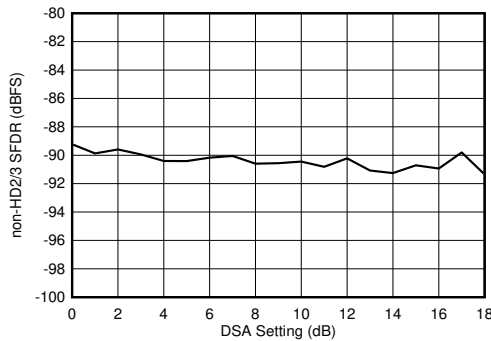
图 6-133. RX Non-HD2/3 vs DSA Setting at 2.6 GHz
