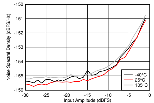
图 6-116. RX Noise Spectral Density vs Input Amplitude and Temperature at 2.6 GHz
