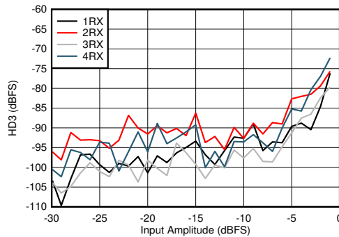
图 6-129. RX HD3 vs Input Level and Channel at 2.6 GHz
