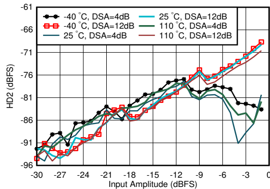
图 6-72. RX HD2 vs Input Level and Temperature at 0.8 GHz
