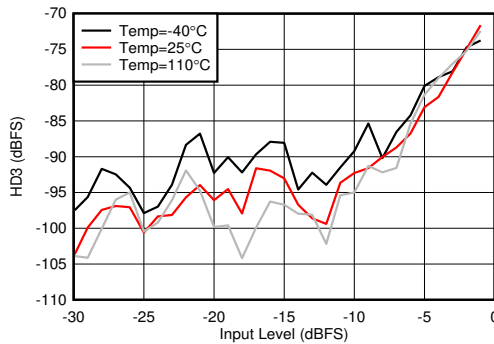
图 6-161. RX HD3 vs Input Level and Temperature at 3.6 GHz
