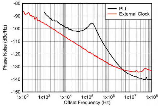
图 6-229. Phase Noise vs Offset Frequency for PLL and External Clock at 12GHz
