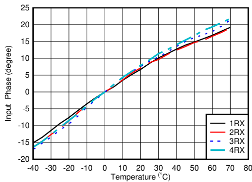
图 6-83. RX Input Phase vs Temperature and DSA at f_{\text{IN}} = 1.75\text{ GHz}
