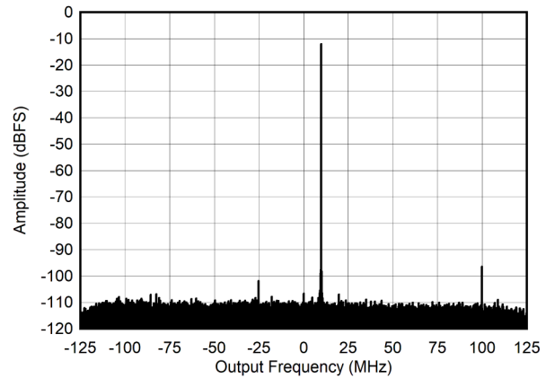
图 6-40. RX Output FFT at 405 MHz and -12dBFS
