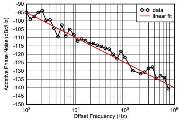
图 6-230. RX Additive Phase Noise at 9.61GHz
