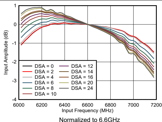
图 6-202. RX In-Band Gain Flatness
