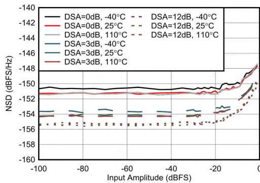
图 6-165. RX Noise Spectral Density vs Input Level at 3.76GHz
