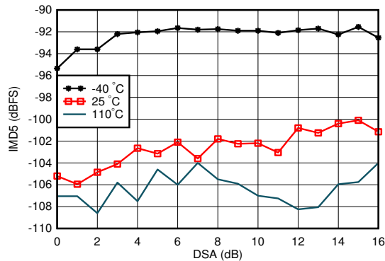
图 6-66. RX IMD5 vs DSA Setting and Temperature at 0.8 GHz
