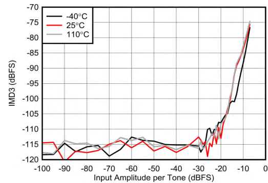
图 6-122. RX IMD3 vs Input Level at 2.6 GHz (Ext. Clock)
