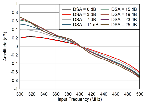
图 6-29. RX In-Band Gain Flatness, f_{\text{IN}} = 400\text{ MHz}
