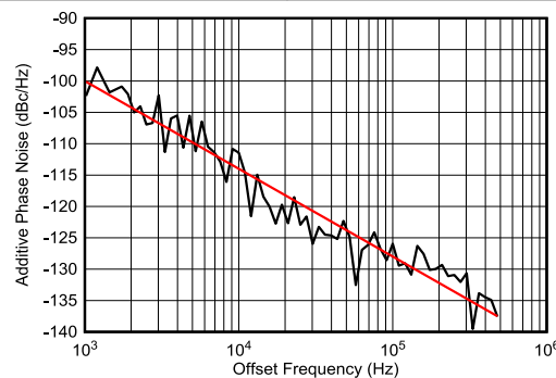
图 6-228. RX Additive Phase Noise at 6.85GHz
