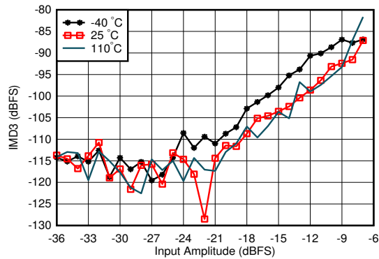
图 6-189. RX IMD3 vs Input Level and Temperature at 4.9 GHz
