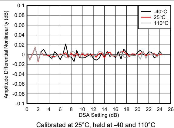
图 6-204. RX Calibrated Differential Amplitude Error at 6.851GHz
