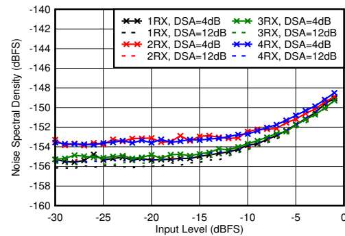
图 6-164. RX Noise Spectral Density vs Input Level and DSA Setting at 3.6 GHz
