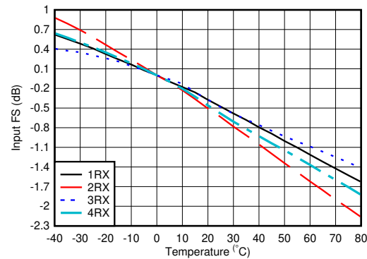
图 6-174. RX Input Fullscale vs Temperature and Channel at 4.9 GHz
