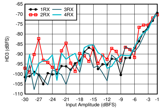
图 6-196. RX HD3 vs Input Level and Channel at 4.9 GHz
