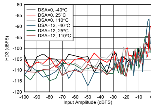
图 6-225. RX HD3 vs Input Amplitude at 6.851GHz
