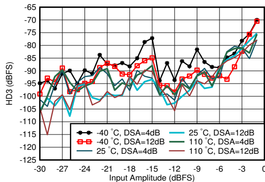
图 6-74. RX HD3 vs DSA Setting and Temperature at 0.8 GHz
