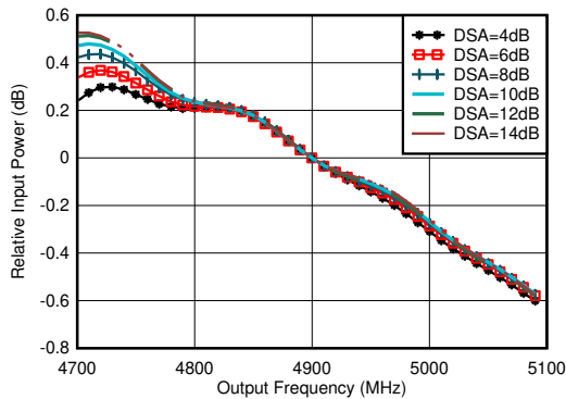
图 6-173. RX Inband Gain Flatness, f_{\text{IN}} = 4900\text{ MHz}
