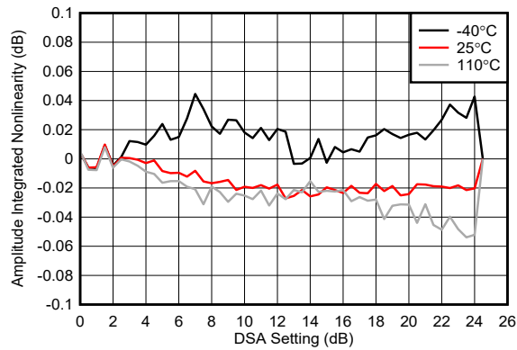
图 6-206. RX Calibrated Integrated Amplitude Error at 6.851GHz
