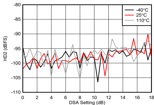
图 6-224. RX HD2 vs DSA Setting at 6.851GHz
