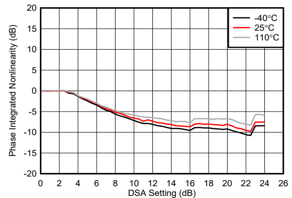
图 6-209. RX Uncalibrated Integrated Phase Error at 6.851GHz
