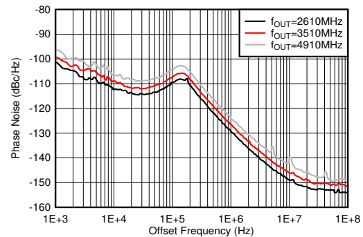
图 6-256. Phase Noise for 9-GHz VCO vs Offset Frequency and f_{OUT} at 25°C
