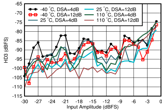
图 6-104. RX HD3 vs DSA Setting and Temperature at 1.9 GHz
