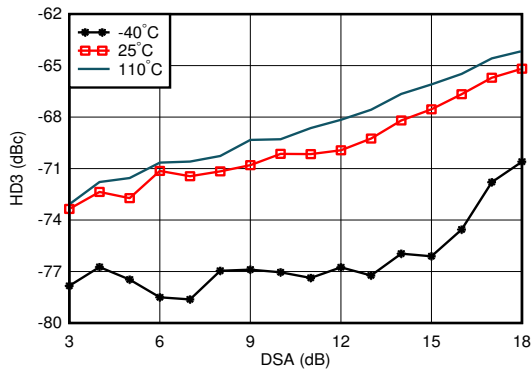
图 6-195. RX HD3 vs DSA Setting and Temperature at 4.9 GHz
