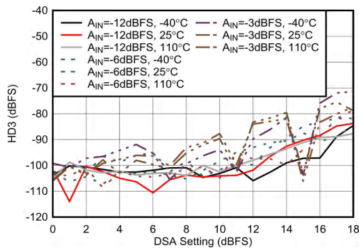
图 6-226. RX HD3 vs DSA Setting at 6.851GHz
