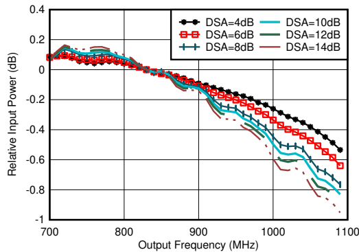
图 6-50. RX In-Band Gain Flatness for Channel 1RX, f_{\text{IN}} = 830\text{ MHz}
