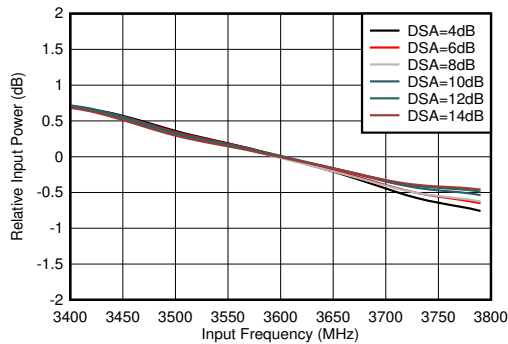
图 6-137. RX In-Band Gain Flatness, f_{\text{IN}} = 3600\text{ MHz}
