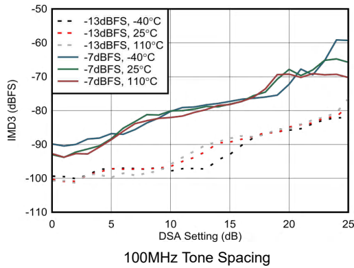
图 6-218. RX IMD3 vs DSA Setting at 6.851GHz
