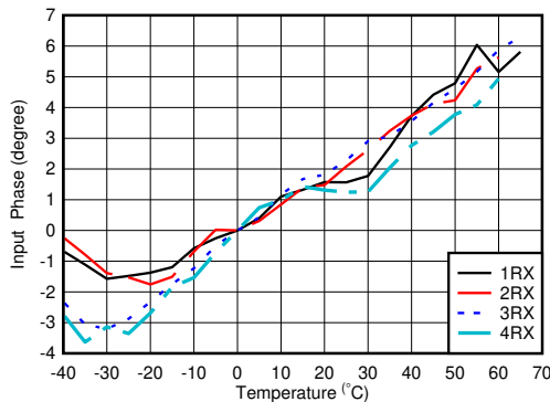
图 6-52. RX Input Phase vs Temperature and DSA at f_{\text{OUT}} = 0.8\text{ GHz}
