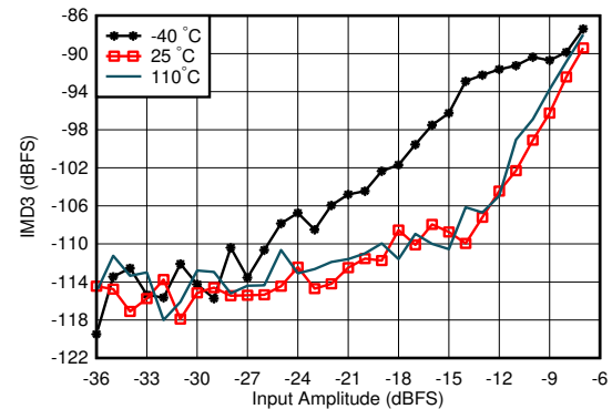
图 6-67. RX IMD3 vs Input Level and Temperature at 0.8 GHz
