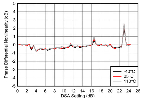
图 6-207. RX Uncalibrated Differential Phase Error at 6.851GHz
