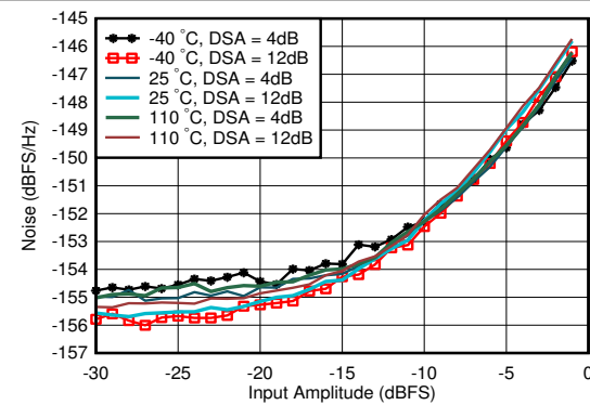
图 6-94. RX Noise Spectral Density vs Input Amplitude and Temperature at 1.75 GHz
