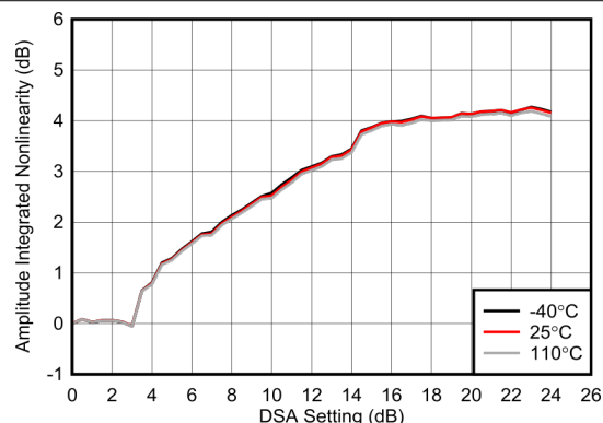
图 6-205. RX Uncalibrated Integrated Amplitude Error at 6.851GHz
