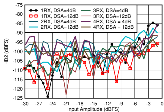
图 6-99. RX HD2 vs DSA Setting and Channel at 1.9 GHz
