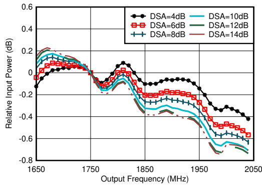
图 6-81. RX In-Band Gain Flatness, f_{\text{IN}} = 1750\text{ MHz}
