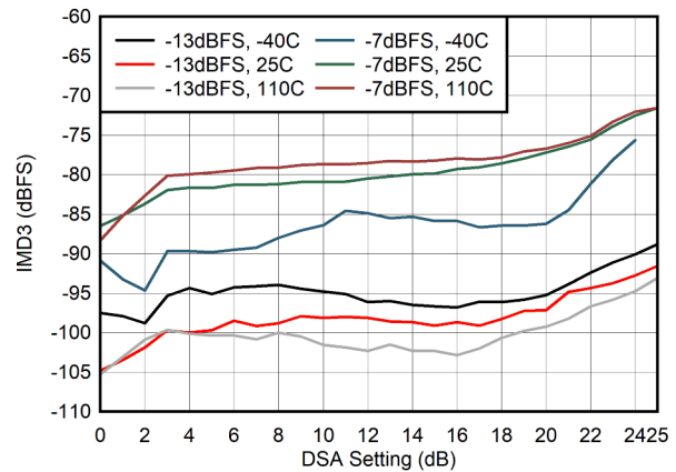
图 6-46. IMD3 vs DSA Setting at 400MHz
