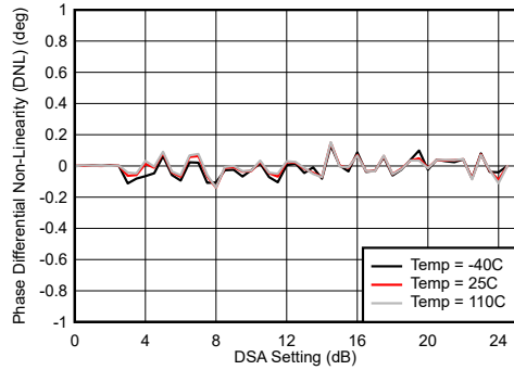
图 6-7. RX Calibrated Differential Phase Error vs DSA Setting at 30 MHz
