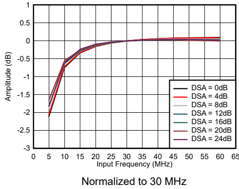
图 6-1. RX In-Band Gain Flatness, f_{\text{IN}} = 30\text{ MHz}
