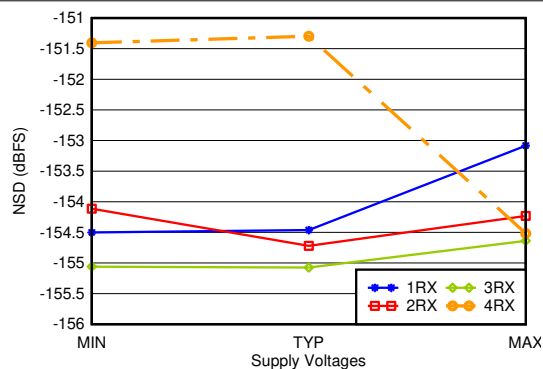
图 6-201. RX Noise Spectral Density vs Supply and Channel at 4.9 GHz
