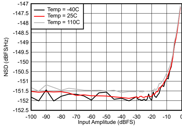
图 6-21. NSD vs Input Amplitude at 30 MHz with DSA = 12
