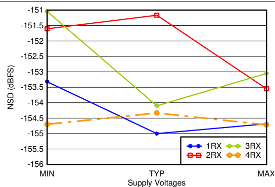
图 6-110. RX Noise Spectral Density vs Supply and Channel at 1.75 GHz
