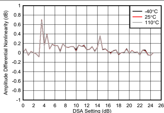
图 6-203. RX Uncalibrated Differential Amplitude Error at 6.851GHz
