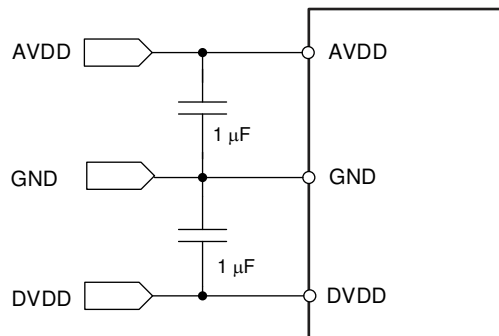
图 9-1. Power-Supply Decoupling
