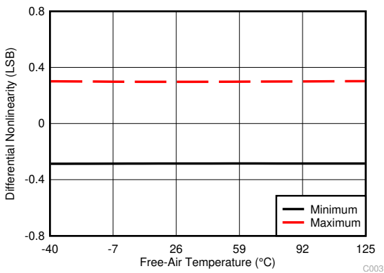
图 6-3. Typical DNL
