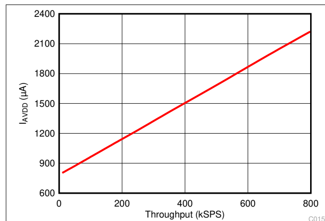
图 6-21. Analog Supply Current vs Throughput
