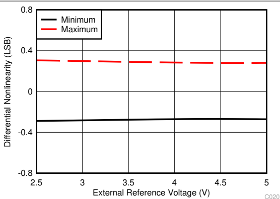
图 6-7. DNL vs External Reference Voltage
