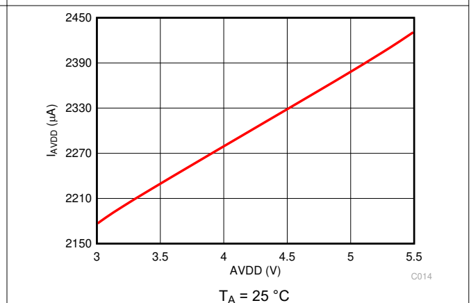
图 6-20. Analog Supply Current vs AVDD
