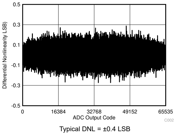
图 6-3. Typical DNL
