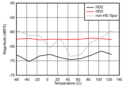
图 6-93. DES Mode: HD2, HD3 and Worst non-HD Spur vs Temperature
