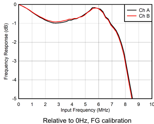
图 6-4. Input Response vs Input Frequency (zoomed)
