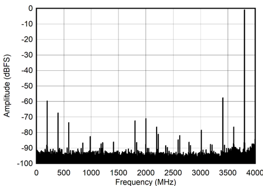
图 6-11. DES Mode: Single Tone FFT at 4197 MHz
