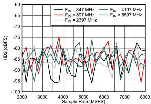
图 6-34. DES Mode: HD2 vs Sample Rate and Input Frequency
