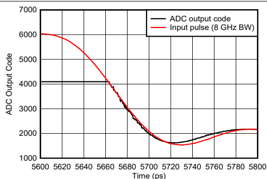
图 6-142. Pulse Overdrive Recovery Zoomed
