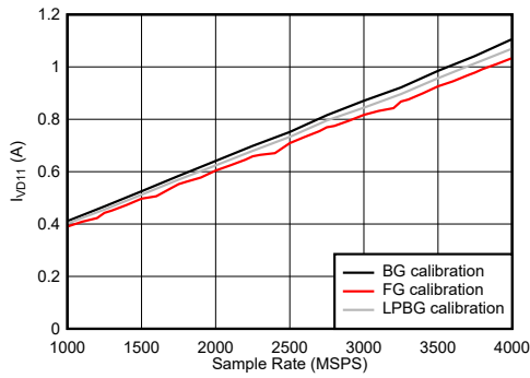
图 6-118. DES Mode: I_{VD11} vs Sample Rate
