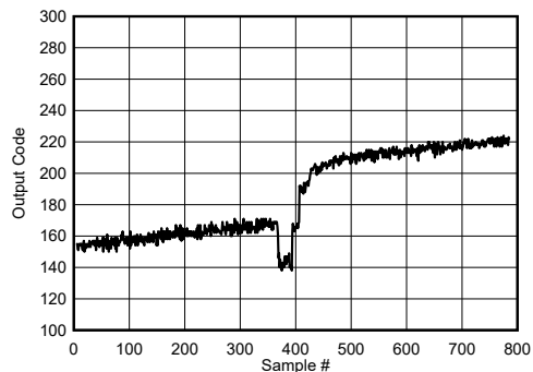
图 6-140. Background Calibration Core Transition (AC Signal Zoomed)
