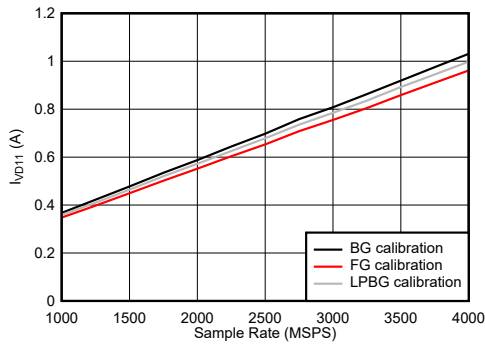
图 6-130. Dual Channel Mode: I_{VD11} vs Sample Rate
