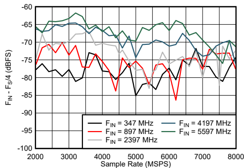
图 6-41. DES Mode: F_{\text{IN}} \pm F_S/4 vs Sample Rate and Input Frequency
