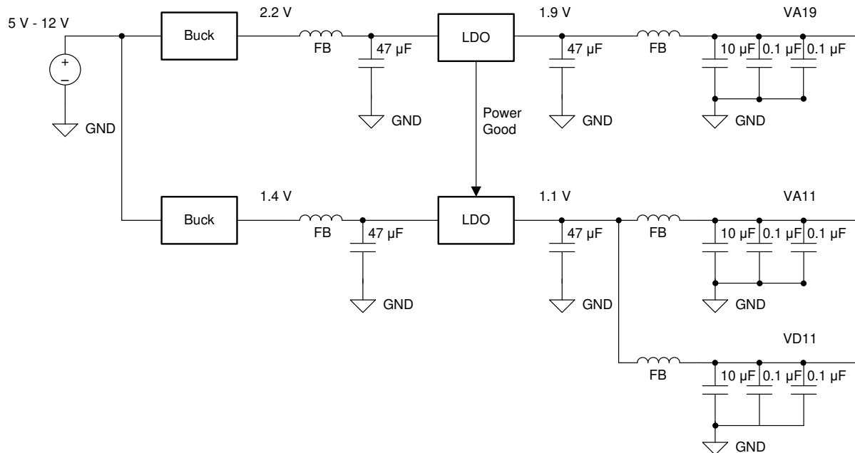
图 8-4. LDO Linear Regulator Approach Example
