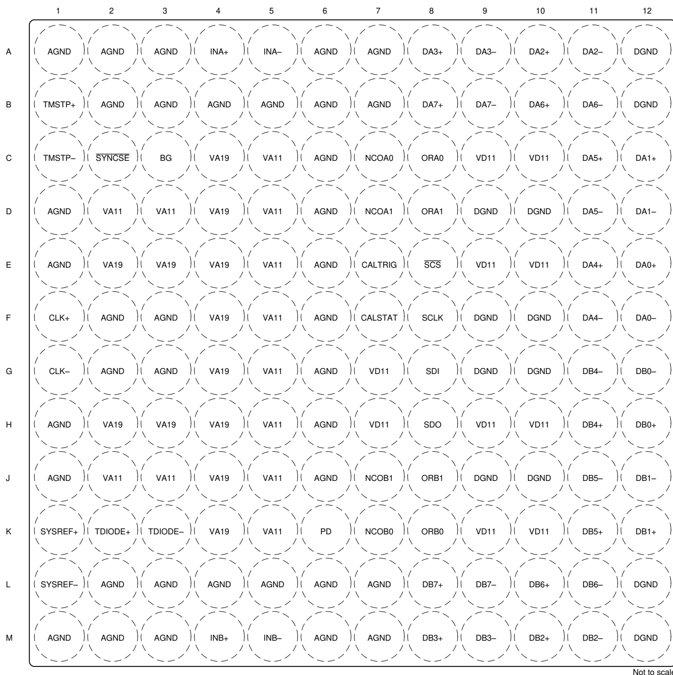
图 5-1. AAV Package, 144-Ball Flip Chip BGA, Top View
