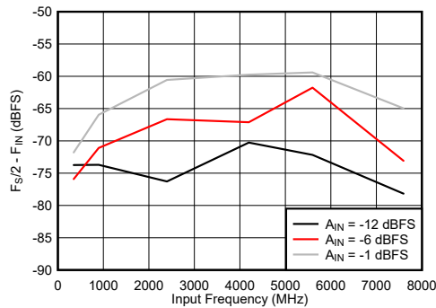
图 6-81. DES Mode: F_S/2 - F_{\text{IN}} vs Input Frequency
