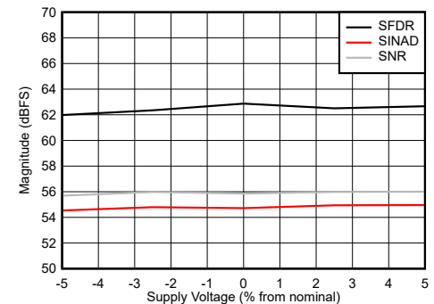
图 6-102. Dual Channel Mode: SNR, SINAD and SFDR vs Supply Voltage
