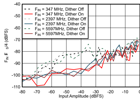
图 6-66. DES Mode: F_{\text{IN}} \pm F_{\text{IN}}/4 vs Input Amplitude and Dither
