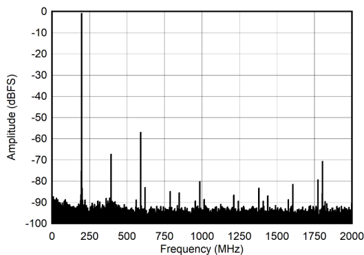
图 6-21. Dual Channel Mode: Single Tone FFT at 4197 MHz
