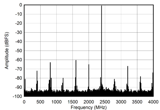
图 6-10. DES Mode: Single Tone FFT at 2397 MHz
