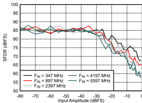
图 6-57. DES Mode: SFDR vs Input Amplitude and Frequency
