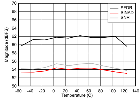
图 6-92. DES Mode: SNR, SINAD and SFDR vs Temperature
