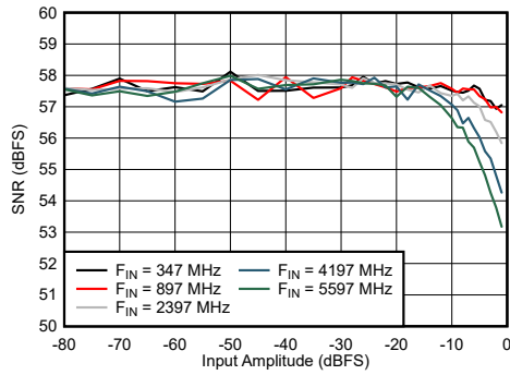
图 6-67. Dual Channel Mode: SNR vs Input Amplitude and Frequency
