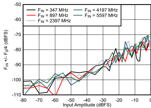
图 6-65. DES Mode: F_{\text{IN}} \pm F_{\text{IN}}/4 vs Input Amplitude and Frequency
