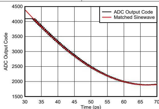
图 6-144. Sinewave Overdrive Recovery
