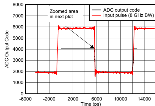
图 6-141. Pulse Overdrive Recovery
