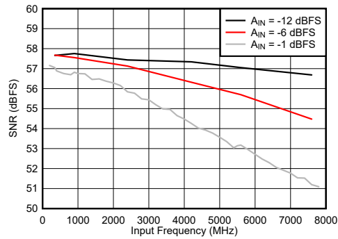
图 6-83. Dual Channel Mode: SNR vs Input Frequency
