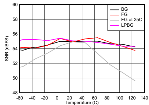
图 6-94. Dual Channel Mode: SNR, SINAD and SFDR vs Temperature
