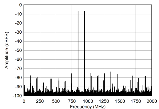
图 6-24. Dual Channel Mode: Two Tone FFT at 897 MHz
