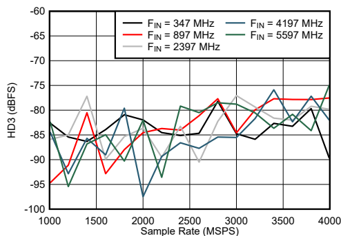
图 6-51. Dual Channel Mode: HD3 vs Sample Rate and Input Frequency
