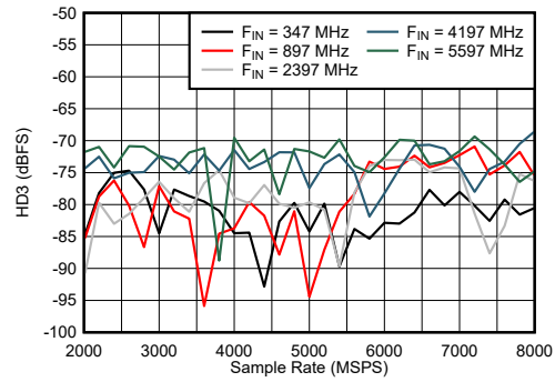
图 6-38. DES Mode: HD3 vs Sample Rate and Input Frequency
