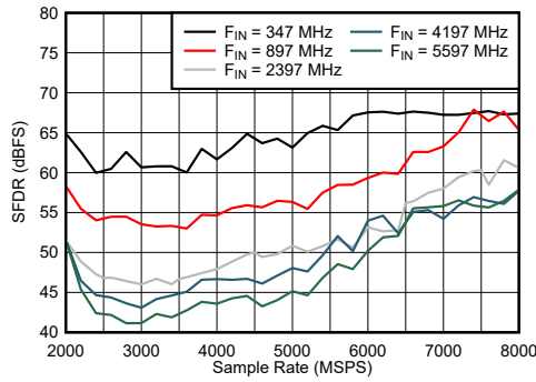
图 6-31. DES Mode: SFDR vs Sample Rate and Input Frequency
