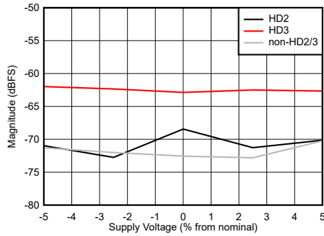
图 6-103. Dual Channel Mode: HD2, HD3 and Worst non-HD Spur vs Supply Voltage
