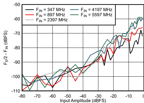
图 6-63. DES Mode: F_{\text{S}}/2 - F_{\text{IN}} vs Input Amplitude and Frequency
