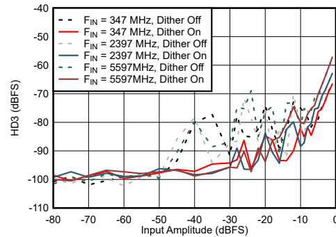
图 6-74. Dual Channel Mode: HD3 vs Input Amplitude and Dither
