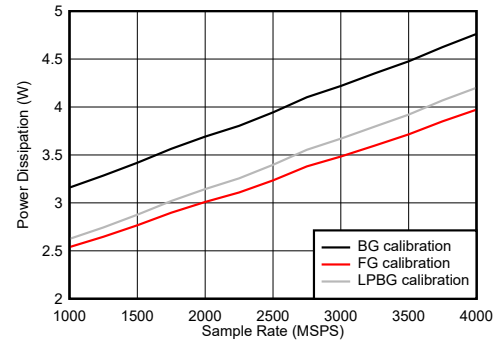
图 6-125. DES Mode: Power Dissipation vs Sample Rate
