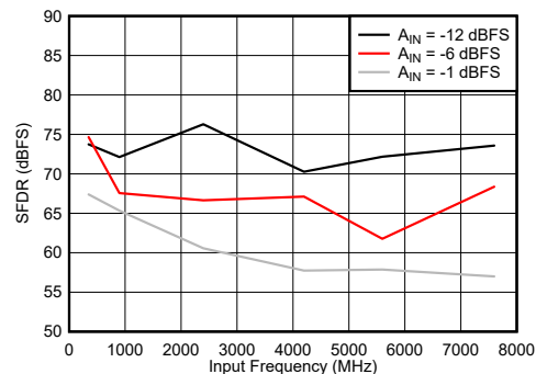
图 6-78. DES Mode: SFDR vs Input Frequency
