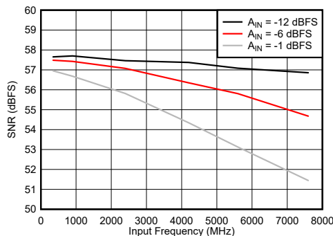
图 6-77. DES Mode: SNR vs Input Frequency
