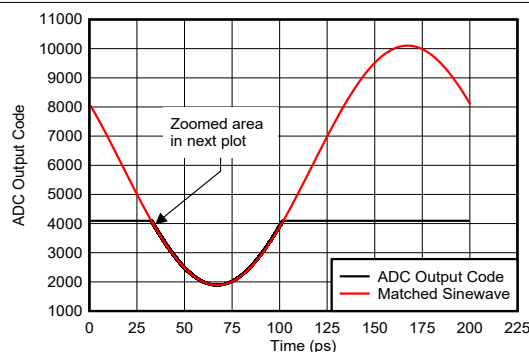
图 6-143. Sinewave Overdrive Recovery
