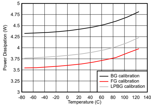
图 6-136. DES Mode: Power Dissipation vs Temperature
