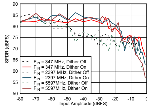
图 6-70. Dual Channel Mode: SFDR vs Input Amplitude and Dither
