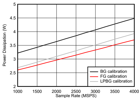
图 6-132. Dual Channel Mode: Power Dissipation vs Sample Rate
