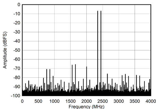
图 6-15. DES Mode: Two Tone FFT at 2397 MHz
