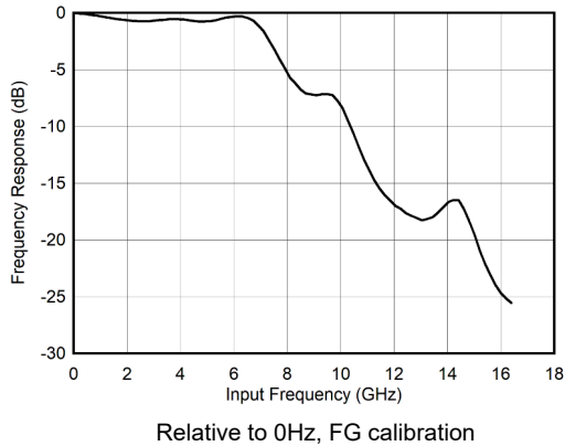
图 6-1. DES Mode: Input Amplitude vs Input Frequency
