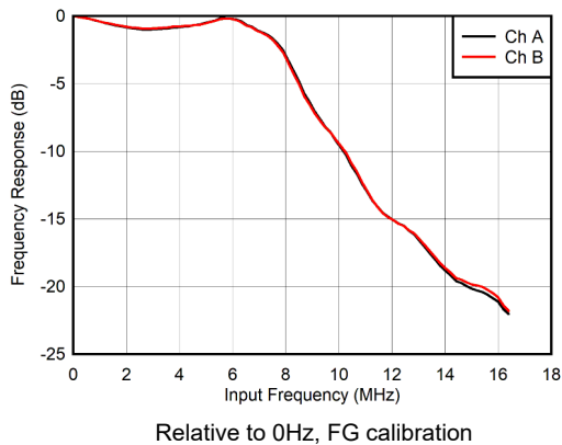
图 6-3. Dual Channel Mode: Input Amplitude vs Input Frequency
