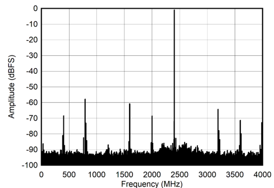
图 6-12. DES Mode: Single Tone FFT at 5597 MHz
