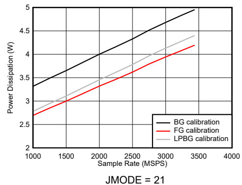
图 6-123. DES Mode: Power Dissipation vs Sample Rate
