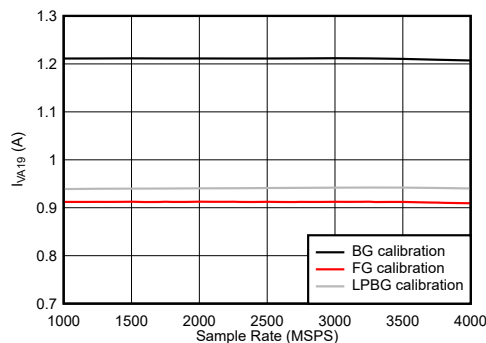
图 6-116. DES Mode: I_{V_{A19}} vs Sample Rate
