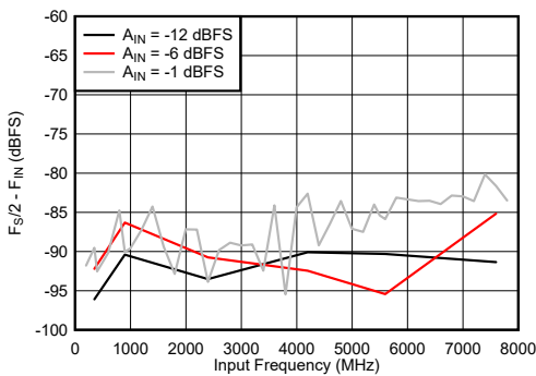
图 6-87. Dual Channel Mode: F_S/2 - F_{\text{IN}} vs Input Frequency
