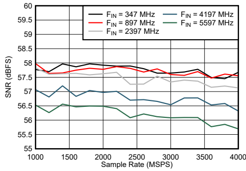
图 6-43. Dual Channel Mode: SNR vs Sample Rate and Input Frequency
