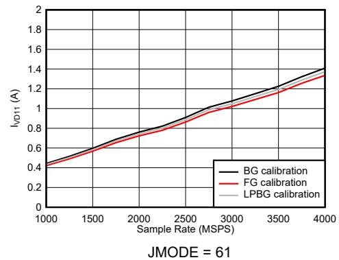
图 6-121. DES Mode: I_{VD11} vs Sample Rate
