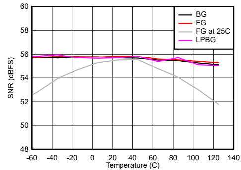
图 6-98. Dual Channel Mode: SNR vs Temperature and Calibration Mode
