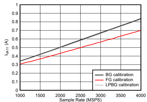
图 6-117. DES Mode: I_{V_{A11}} vs Sample Rate
