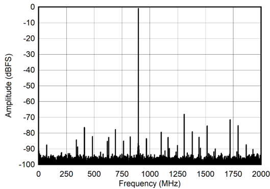
图 6-19. Dual Channel Mode: Single Tone FFT at 897 MHz
