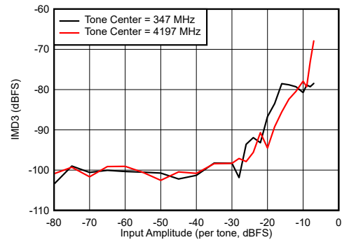
图 6-106. DES Mode: IMD3 vs Input Amplitude
