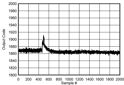
图 6-138. Background Calibration Core Transition (DC Offset Signal)
