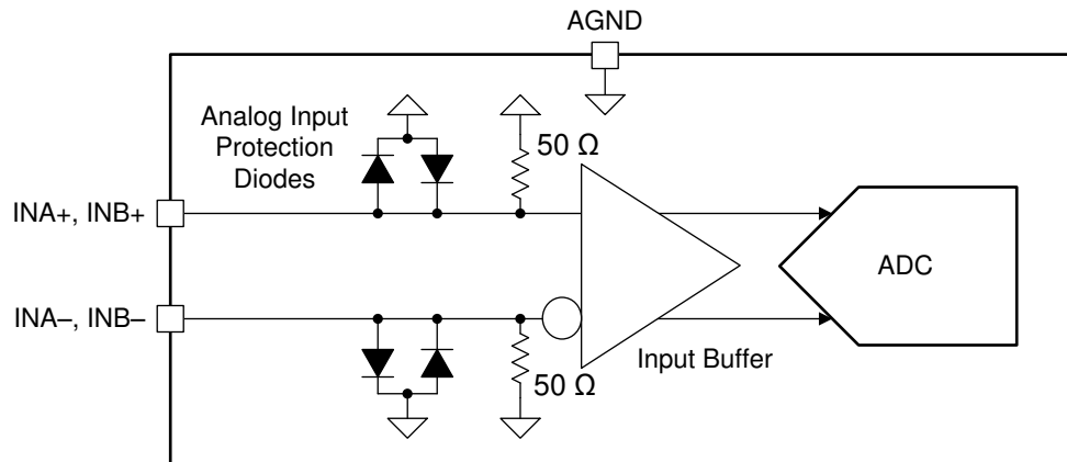
图 7-1. ADC12DJ4000RF Analog Input Internal Termination and Protection Diagram
