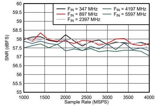
图 6-44. Dual Channel Mode: SNR vs Sample Rate and Input Frequency
