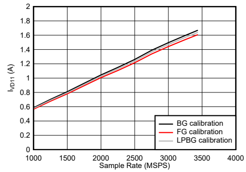
图 6-119. DES Mode: I_{VD11} vs Sample Rate
