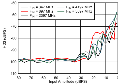
图 6-61. DES Mode: HD3 vs Input Amplitude and Frequency
