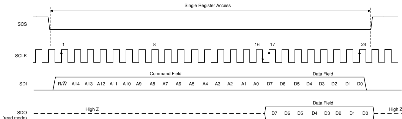
图 7-27. Serial Interface Protocol: Single Read/Write
