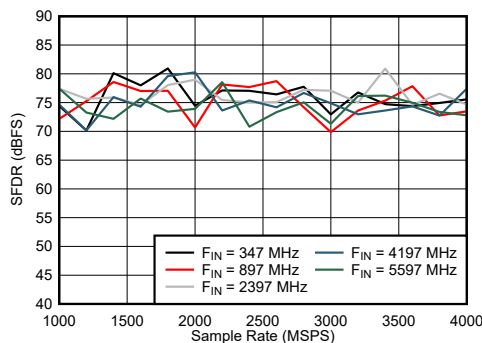
图 6-45. Dual Channel Mode: SFDR vs Sample Rate and Input Frequency
