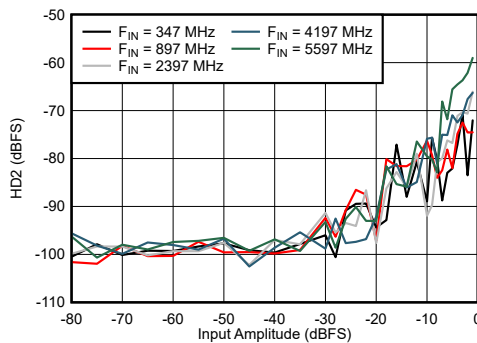
图 6-71. Dual Channel Mode: HD2 vs Input Amplitude and Frequency
