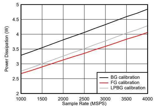
图 6-133. Dual Channel Mode: Power Dissipation vs Sample Rate
