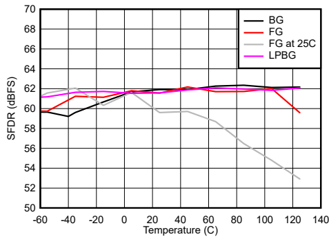
图 6-97. DES Mode: SFDR vs Temperature and Calibration Mode
