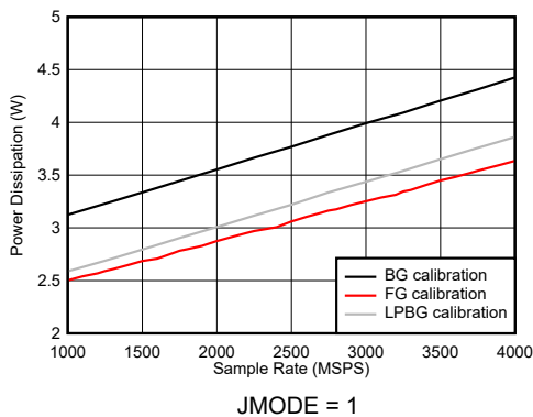
图 6-122. DES Mode: Power Dissipation vs Sample Rate
