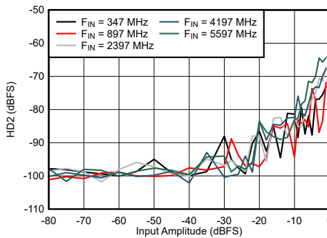
图 6-59. DES Mode: HD2 vs Input Amplitude and Frequency
