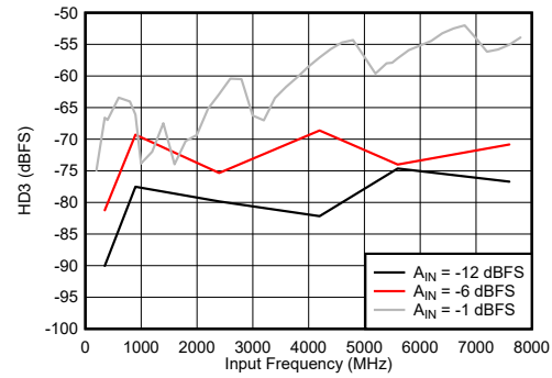
图 6-86. Dual Channel Mode: HD3 vs Input Frequency
