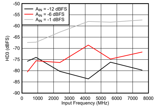
图 6-80. DES Mode: HD3 vs Input Frequency
