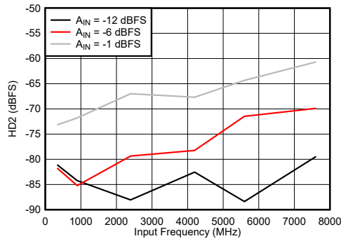
图 6-79. DES Mode: HD2 vs Input Frequency
