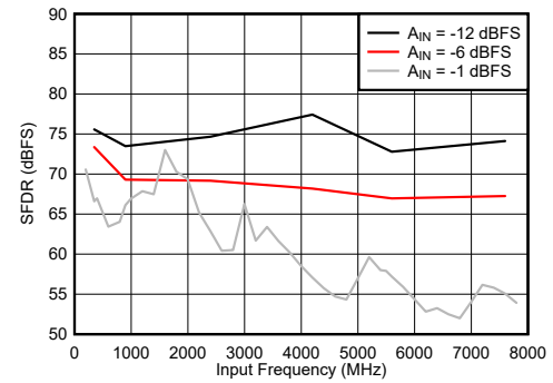
图 6-84. Dual Channel Mode: SFDR vs Input Frequency
