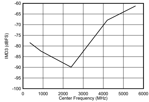
图 6-104. DES Mode: IMD3 vs Input Frequency
