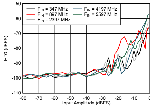
图 6-73. Dual Channel Mode: HD3 vs Input Amplitude and Frequency
