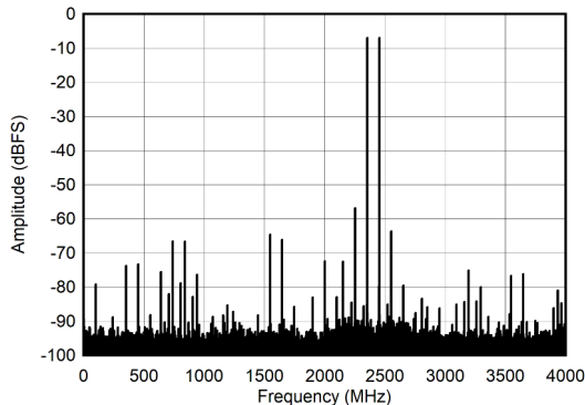
图 6-17. DES Mode: Two Tone FFT at 5597 MHz
