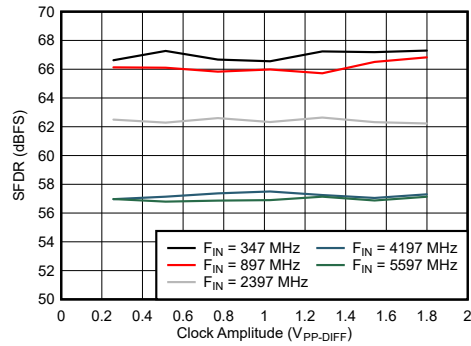
图 6-91. Dual Channel Mode: SFDR vs Clock Amplitude
