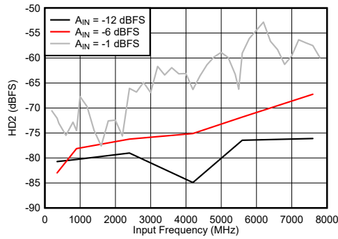
图 6-85. Dual Channel Mode: HD2 vs Input Frequency
