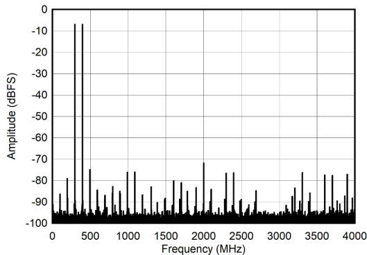
图 6-13. DES Mode: Two Tone FFT at 347 MHz
