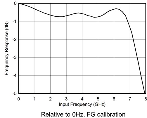
图 6-2. DES Mode: Input Response vs Input Frequency
