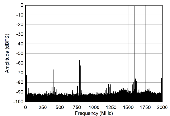
图 6-22. Dual Channel Mode: Single Tone FFT at 5597 MHz
