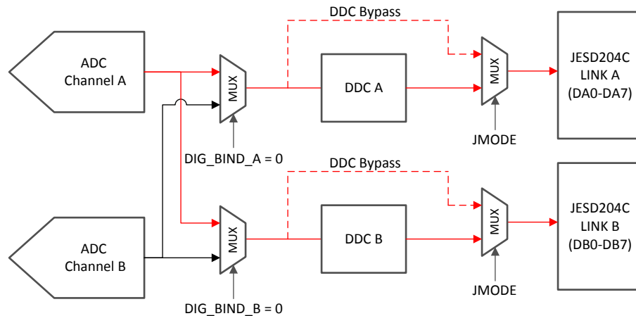
图 7-24. Dual DDC Mode or Redundant Data Mode for Channel A
