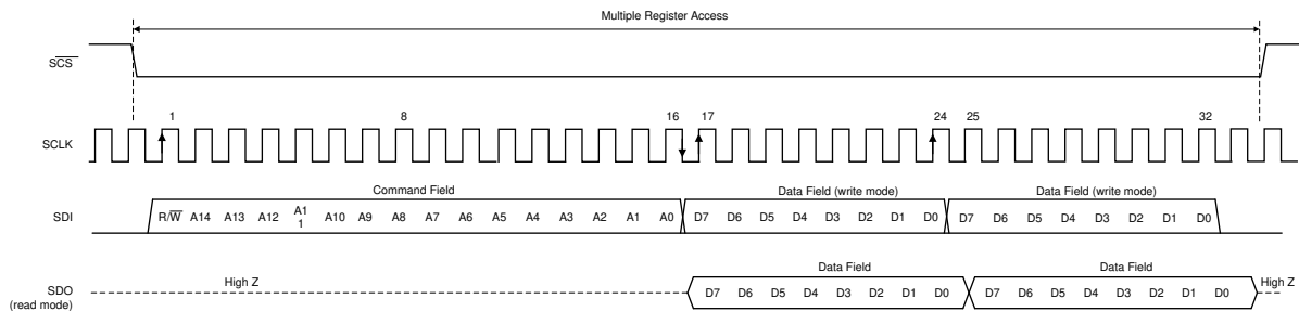
图 7-28. Serial Interface Protocol: Streaming Read/Write
