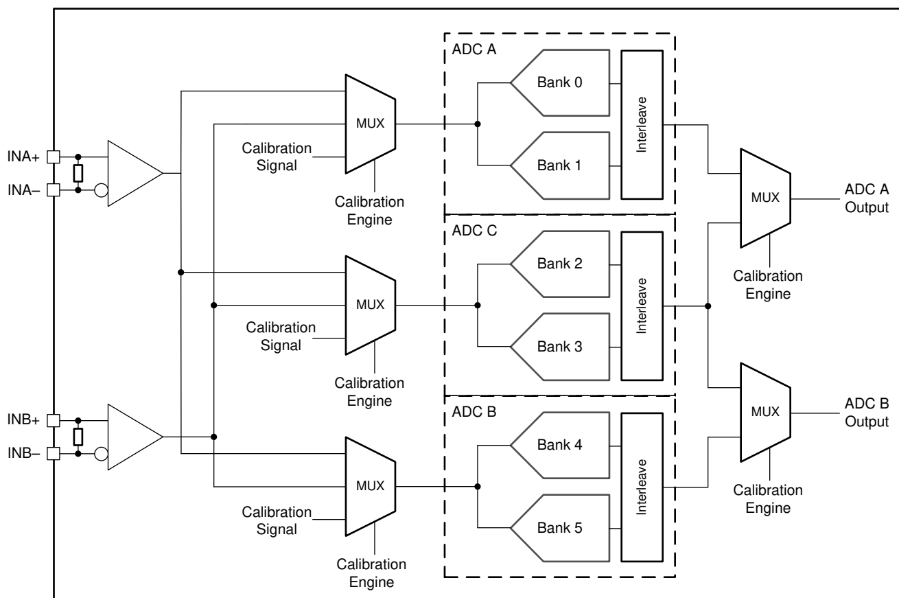
图 7-26. ADC12DJ4000RF Calibration System Block Diagram
