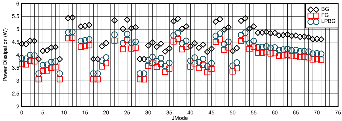
图 6-114. Power Dissipation vs JMODE at F_{\text{CLK}} = 4\text{ GHz}
