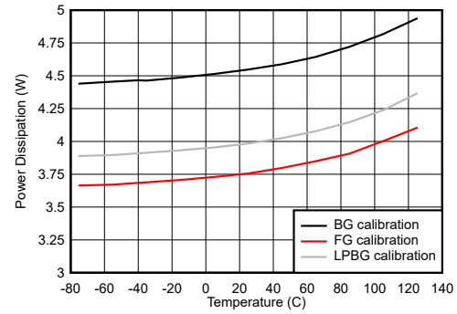
图 6-137. Dual Channel Mode: Power Dissipation vs Temperature
