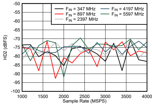
图 6-49. Dual Channel Mode: HD2 vs Sample Rate and Input Frequency
