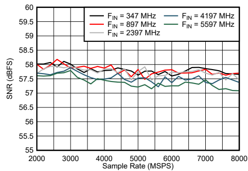
图 6-30. DES Mode: SNR vs Sample Rate and Input Frequency
