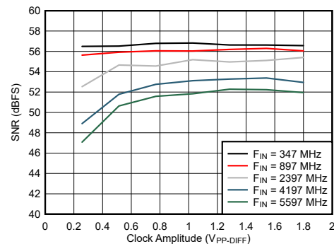
图 6-88. DES Mode: SNR vs Clock Amplitude
