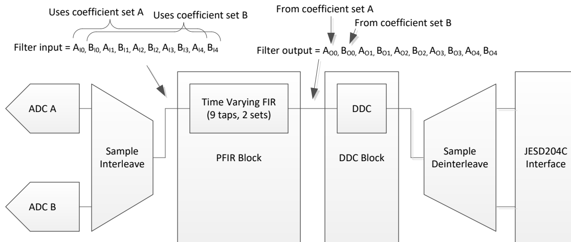
图 7-6. Time Varying Filter PFIR Block Diagram
