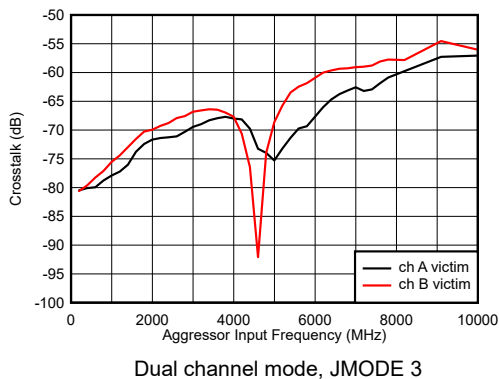
图 6-5. Crosstalk vs Input Frequency
