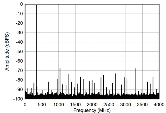
图 6-8. DES Mode: Single Tone FFT at 347 MHz
