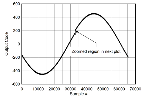
图 6-139. Background Calibration Core Transition (AC Signal)
