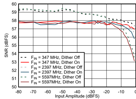
图 6-56. DES Mode: SNR vs Input Amplitude and Dither
