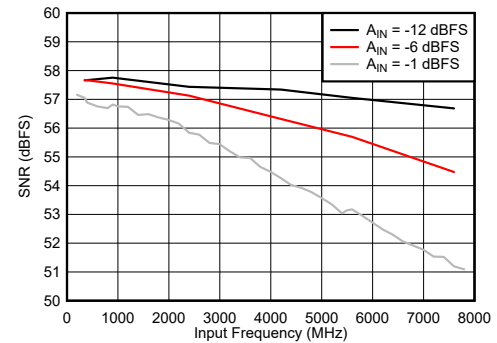
图 6-82. DES Mode: F_{\text{IN}} \pm F_S/4 vs Input Frequency
