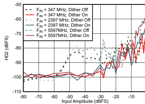
图 6-72. Dual Channel Mode: HD2 vs Input Amplitude and Dither
