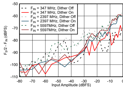
图 6-64. DES Mode: F_{\text{S}}/2 - F_{\text{IN}} vs Input Amplitude and Dither
