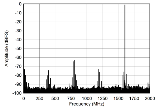
图 6-20. Dual Channel Mode: Single Tone FFT at 2397 MHz
