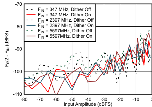
图 6-76. Dual Channel Mode: F_S/2 - F_{\text{IN}} vs Input Amplitude and Dither
