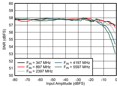
图 6-55. DES Mode: SNR vs Input Amplitude and Frequency
