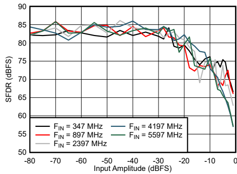
图 6-69. Dual Channel Mode: SFDR vs Input Amplitude and Frequency
