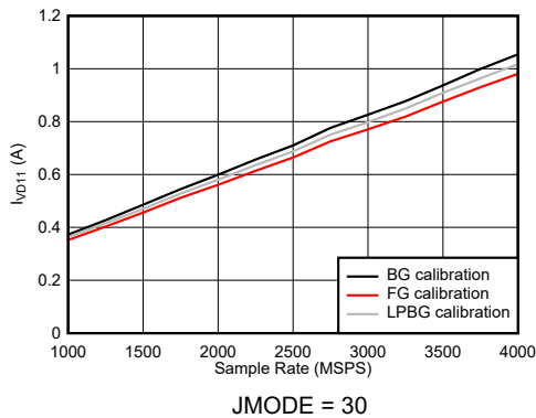
图 6-120. DES Mode: I_{VD11} vs Sample Rate
