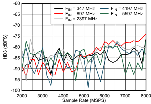
图 6-37. DES Mode: HD3 vs Sample Rate and Input Frequency
