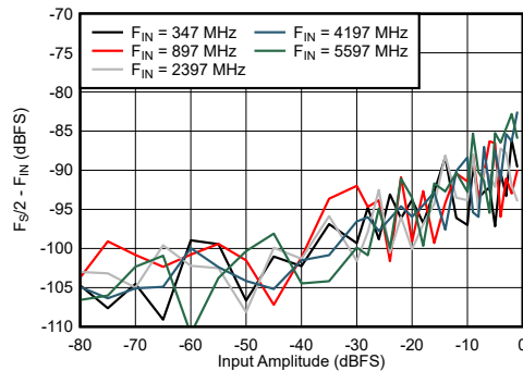
图 6-75. Dual Channel Mode: F_S/2 - F_{\text{IN}} vs Input Amplitude and Frequency
