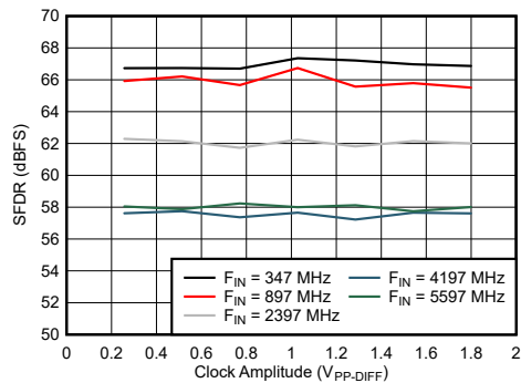
图 6-89. DES Mode: SFDR vs Clock Amplitude
