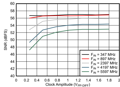
图 6-90. Dual Channel Mode: SNR vs Clock Amplitude
