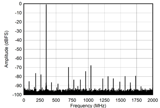
图 6-18. Dual Channel Mode: Single Tone FFT at 347 MHz
