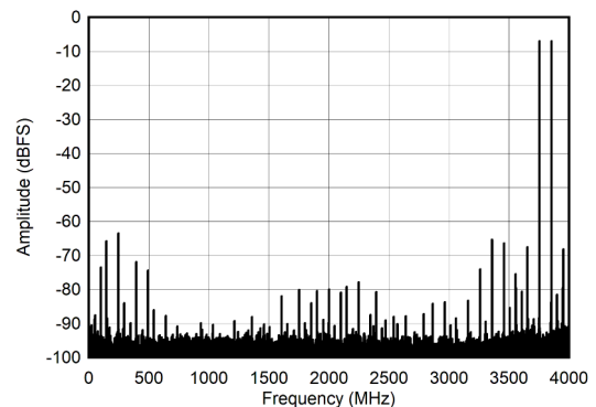
图 6-16. DES Mode: Two Tone FFT at 4197 MHz
