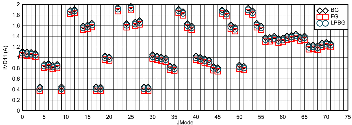
图 6-115. I_{V_{D11}} vs JMODE at F_{\text{CLK}} = 4\text{ GHz}
