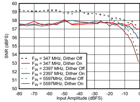
图 6-68. Dual Channel Mode: SNR vs Input Amplitude and Dither
