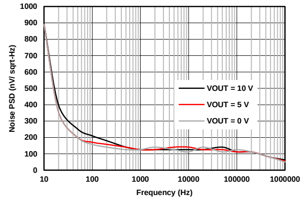
图 69. VOUT Noise Density vs Frequency
