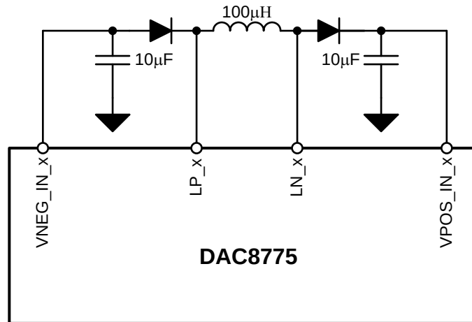
图 127. DAC8775 External Buck-Boost Components with Recommended Values
