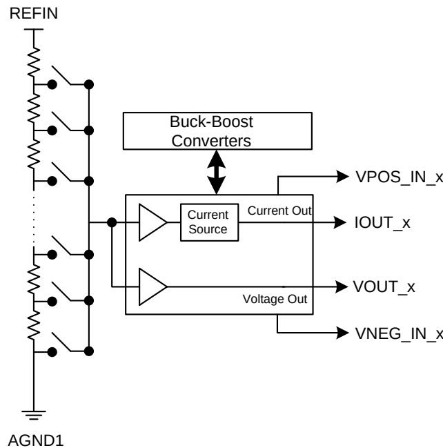
图 100. General Architecture
