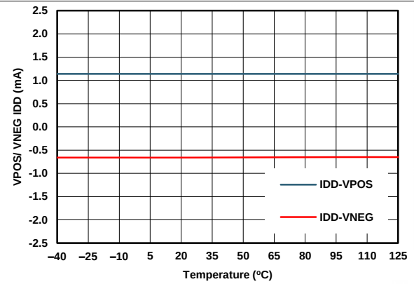
图 22. IOUT Power Supply Current vs Temperature
