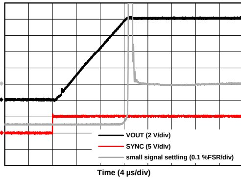
图 62. VOUT Full-Scale Settling Time, Rising Edge
