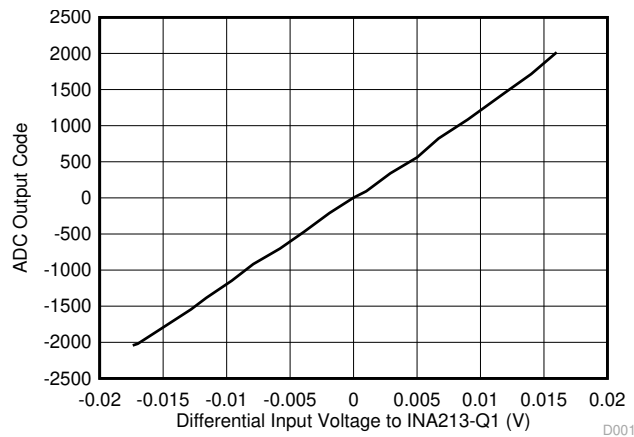
图 8-6. Input Voltage vs ADC Code in Bidirectional Current Sensing Application
