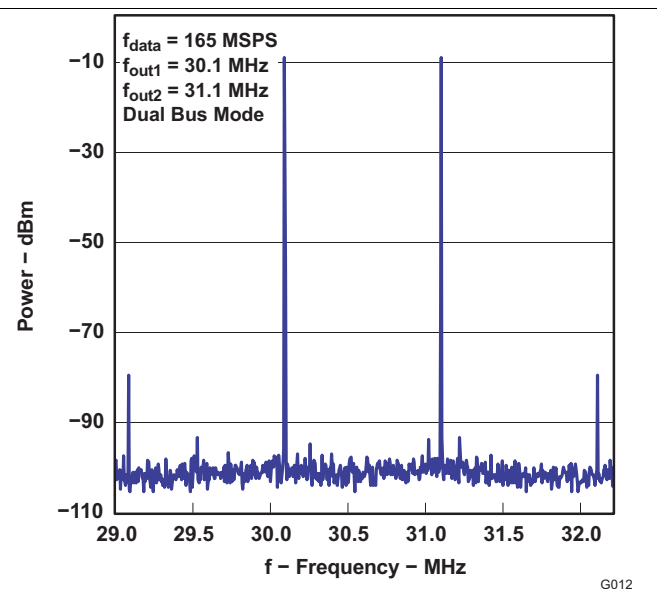
Figure 12. Two-Tone Spectrum
