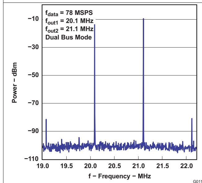
Figure 11. Two-Tone Spectrum
