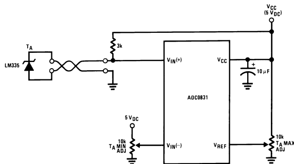
Figure 31. Low-Cost Remote Temperature Sensor
