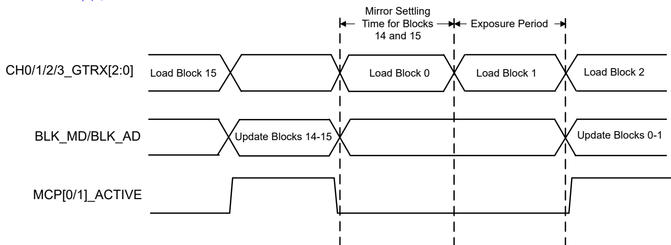
图 6-6. Dual Block Load Phased Sequence
