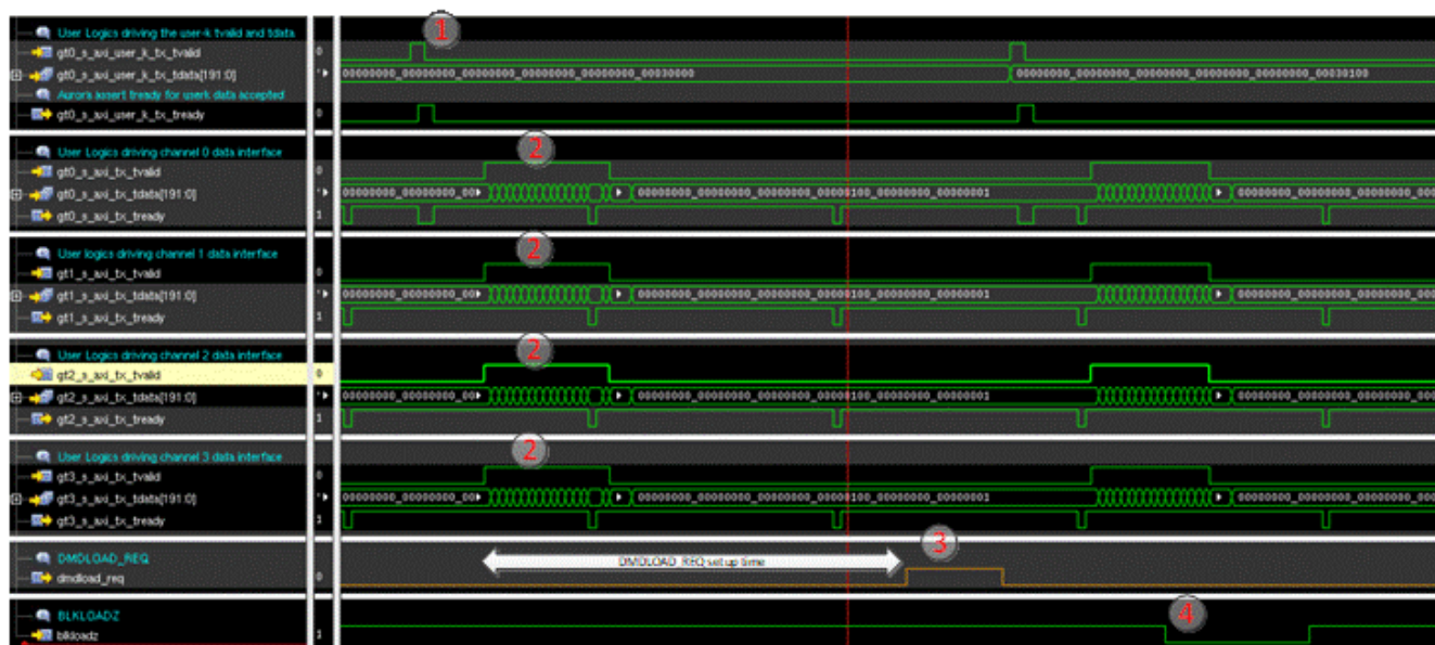
图 7-7. Example of DMDLOAD_REQ Setup Time for Three DMD Row Load Operation
