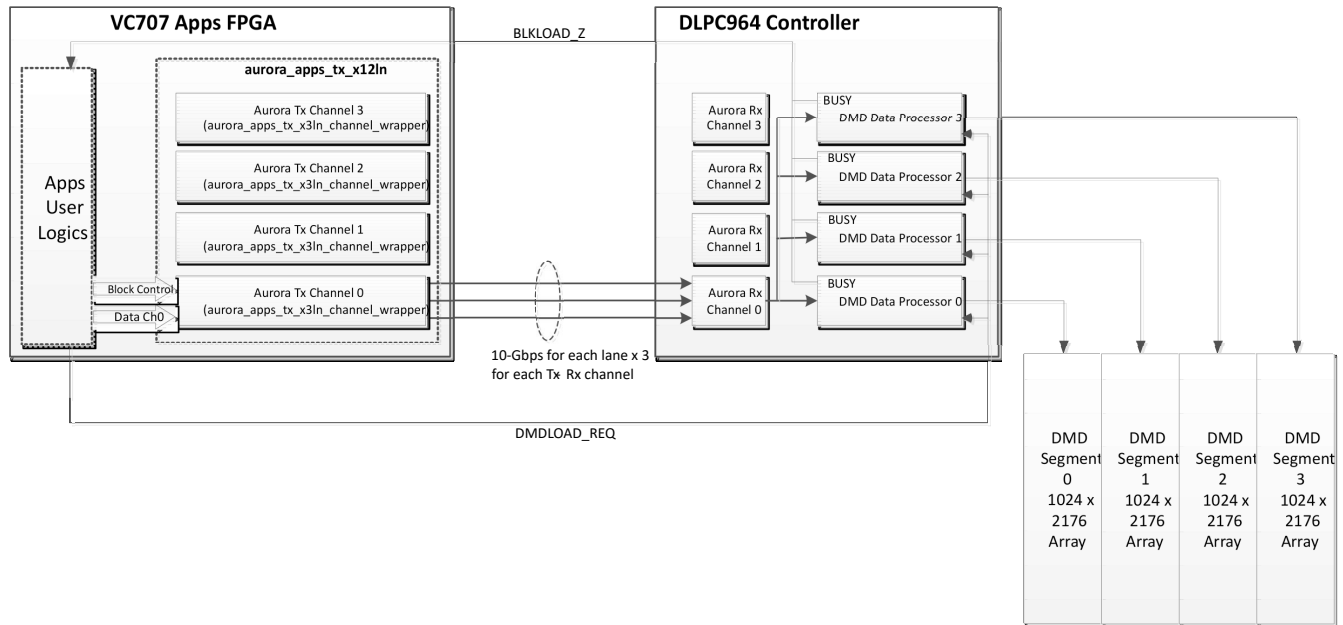
图 7-9. System Block Diagram for Single Channel Transfer Mode
