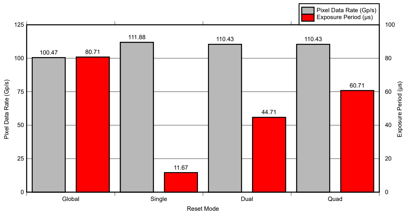
图 7-2. DLP991U DMD Performance Plot at 3.6Gbps Data Rate
