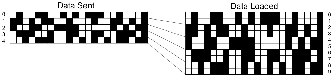
图 6-1. Example LOAD2 Address Mapping
