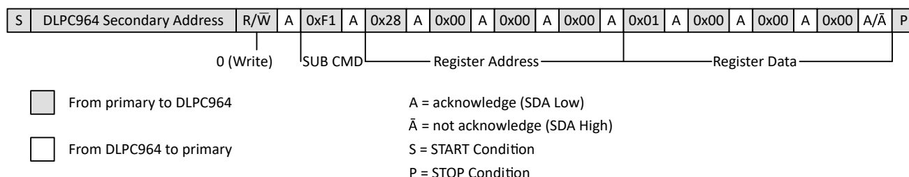
图 6-2. Example I²C Primary Writing DLPC964 Register Data
