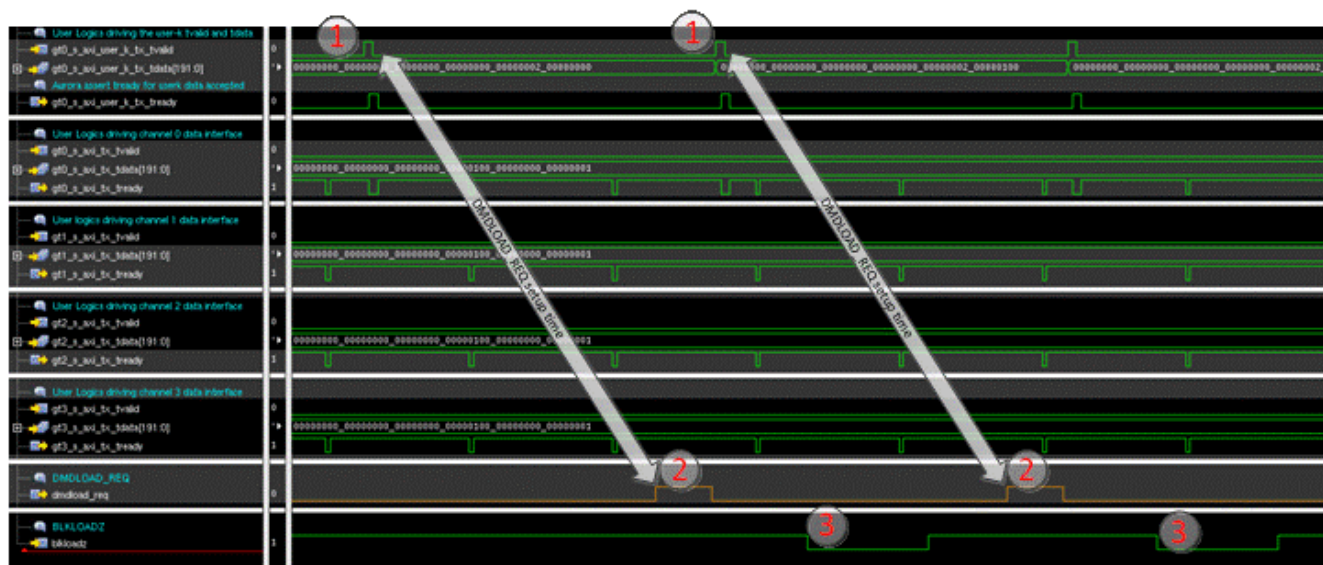
图 7-8. Example of DMDLOAD_REQ Setup Time for Block Set Operation
