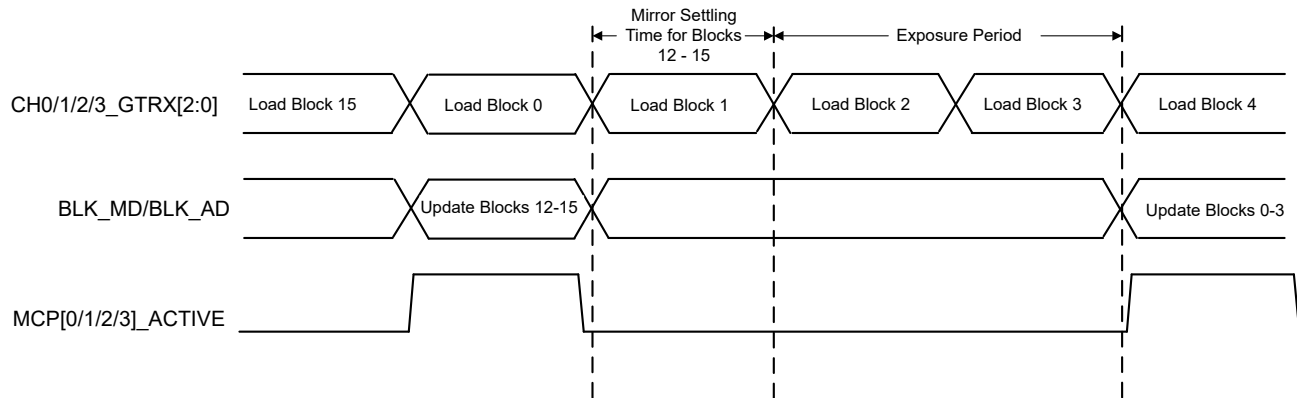
图 6-7. Quad Block Load Phased Sequence
