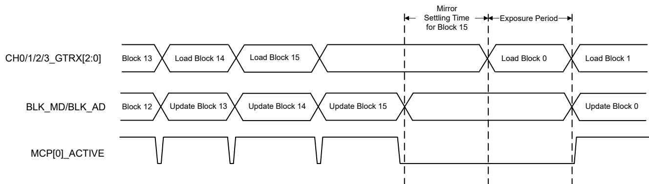
图 6-5. Single Block Load Phased Sequence
