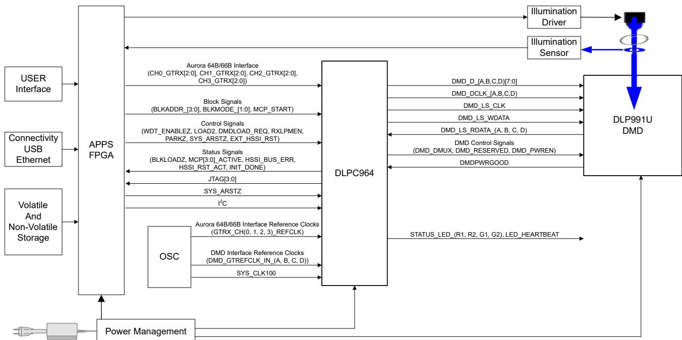
图 7-1. Typical DLP991U High Speed Application
