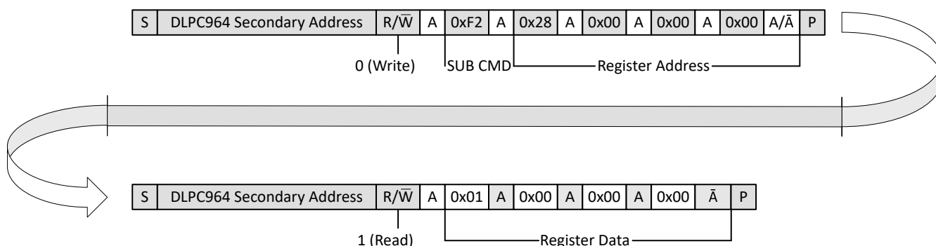
图 6-3. Example I²C Primary Reading DLPC964 Register Data
