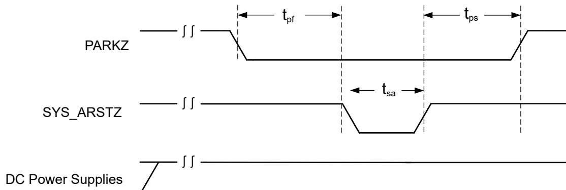
图 7-13. Restart Without Removing Power
