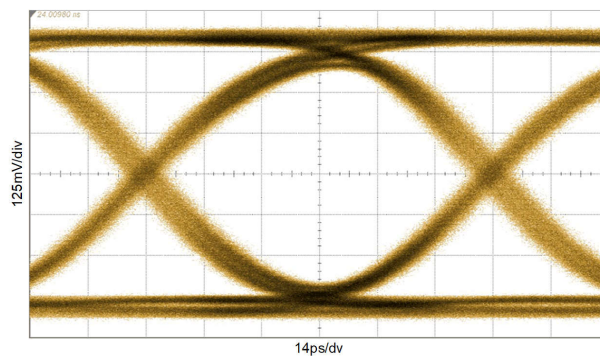
VOD_DE = F, SDI_OUT_SEL = H, OUT_CTRL = F 图 7-7. OUT1± 为 11.88Gbps (12G-SDI) , CC = 100m Belden 1694A , 经过时钟恢复
