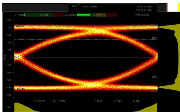
VOD_DE = F, SDI_OUT_SEL = L, OUT_CTRL = F 图 7-8. SDI_OUT+ 为 11.88Gbps (12G-SDI) , CC = 90m Belden 1694A , 经过时钟恢复
