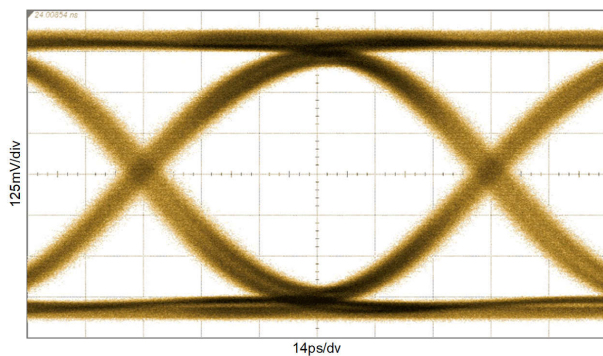
VOD_DE = F, SDI_OUT_SEL = H, OUT_CTRL = F 图 7-6. OUT0± 为 11.88Gbps (12G-SDI) , CC = 100m Belden 1694A , 经过时钟恢复
