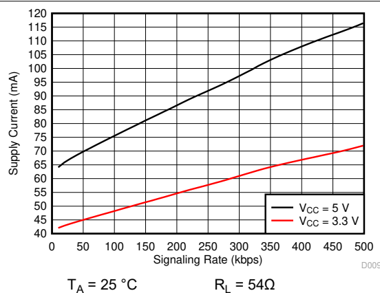
Figure 5-6. THVD2410V-EP Supply Current vs Signal Rate
