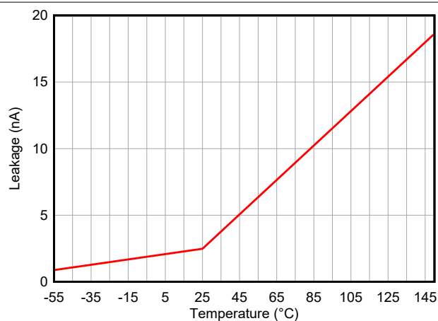
图 5-12. Leakage vs. Temperature
