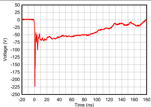
图 5-10. -8kV Clamped IEC Waveform
