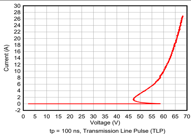
图 5-8. Negative TLP Curve
