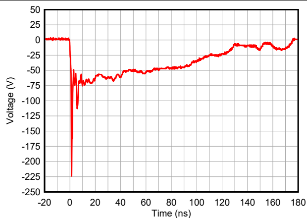
图 5-4. -8kV Clamped IEC Waveform
