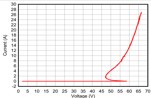
图 5-2. Negative TLP Curve
