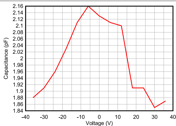
图 5-11. Capacitance vs. Bias Voltage
