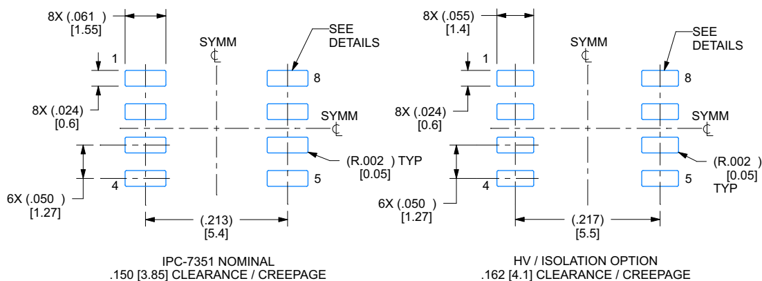
LAND PATTERN EXAMPLE EXPOSED METAL SHOWN SCALE:6X
