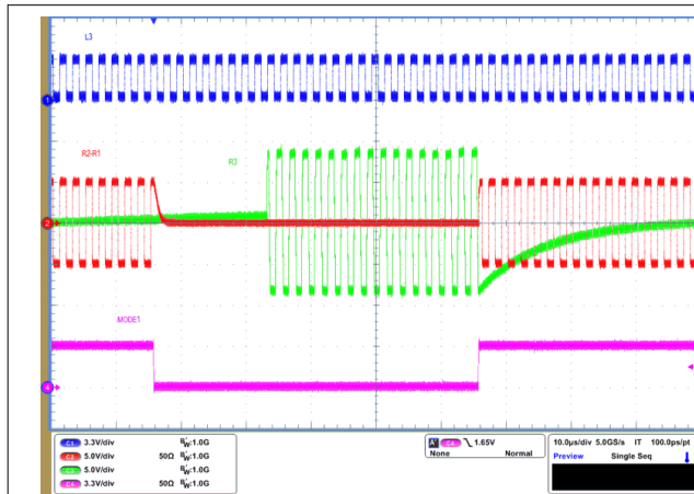
图 8-12. RS-232 to RS-485 Mode Switching Waveform
