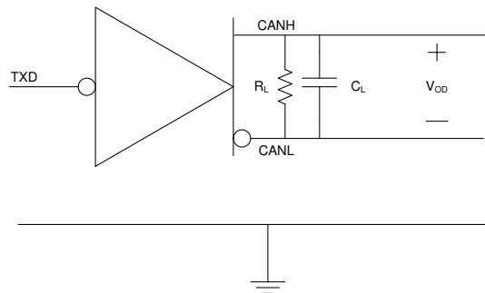
图 8-6. TXD Dominant Timeout Test Circuit and Measurement
