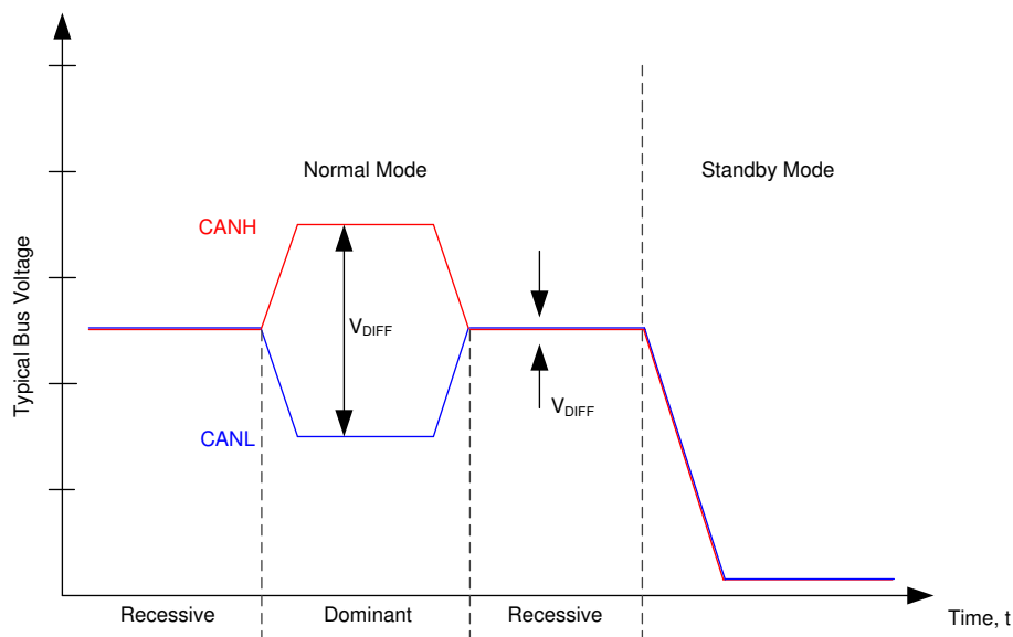
图 9-2. Bus States
