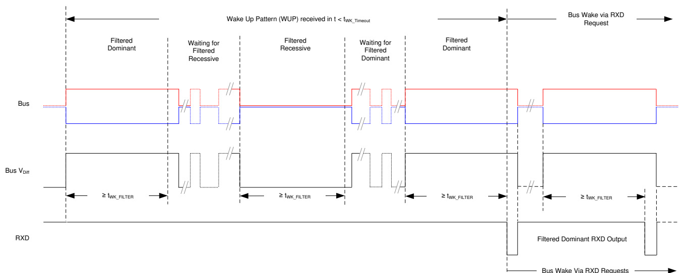
图 9-5. Wake-Up Pattern (WUP) with t_{WK\_TIMEOUT}
