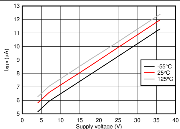
图 5-6. Standby Recessive I_{SUP} vs V_{SUP} and Temperature
