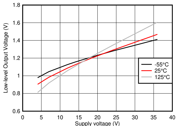
图 5-2. V_{OL} vs V_{SUP} and Temperature
