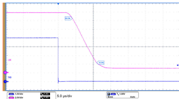
图 8-2. Recessive to Dominant Propagation
