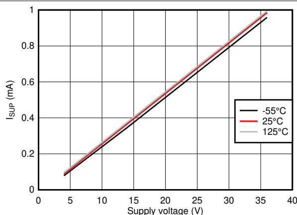
图 5-5. Standby Dominant I_{SUP} vs V_{SUP} and Temperature
