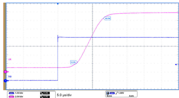
图 8-3. Dominant to Recessive Propagation
