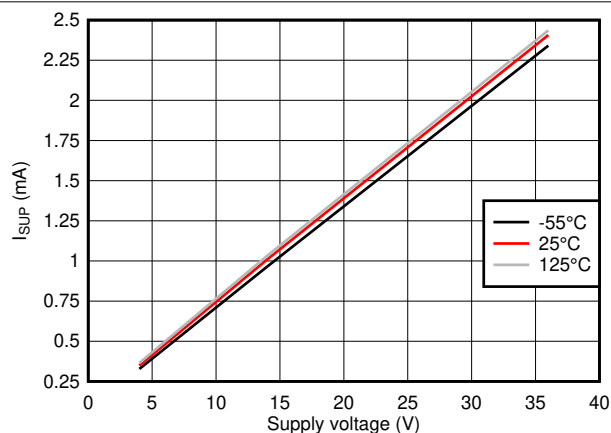
图 5-3. Dominant I_{SUP} vs V_{SUP} and Temperature
