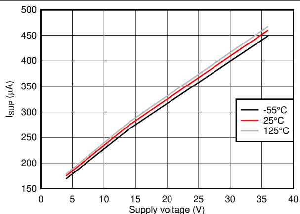
图 5-4. Recessive I_{SUP} vs V_{SUP} and Temperature
