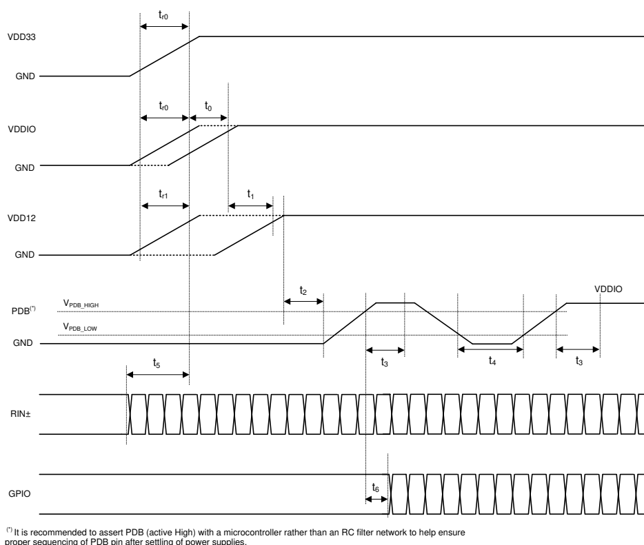
图 45. Power-Up Sequencing
