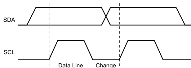
图 8-24. I 2 C Bit Transfer
