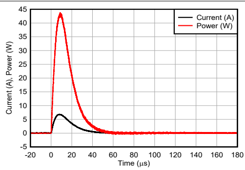
图 6-6. Surge Curve (IEC 61000-4-5, t_p=8/20 \mu s), I/O Pin to GND
