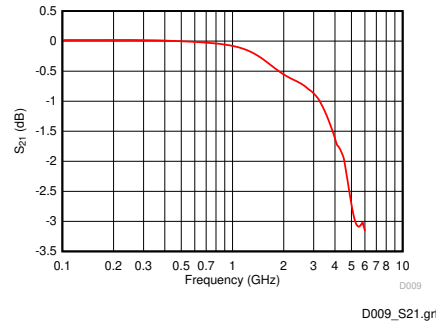
图 8-2. Insertion Loss Vs. Frequency
