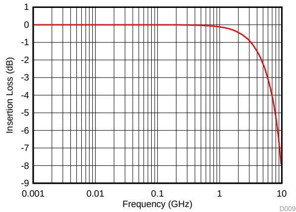
图 9. Insertion Loss
