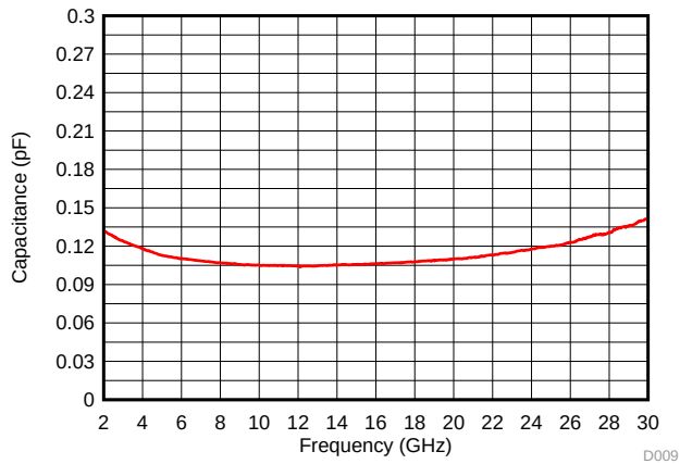
Figure 18. Capacitance vs. Frequency
