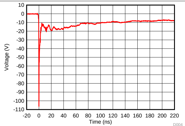
Figure 2. Negative TLP Curve
