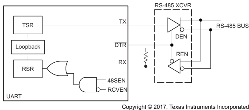
Figure 28. RS-485 Application Example 1
