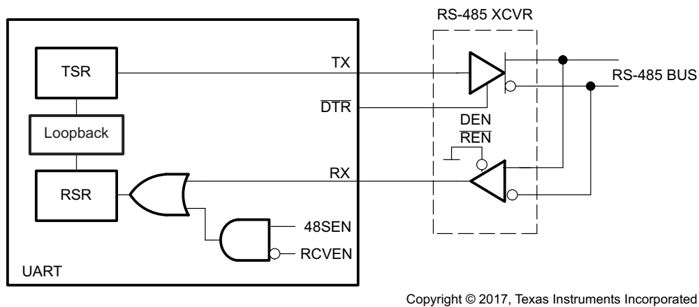
Figure 29. RS-485 Application Example 2
