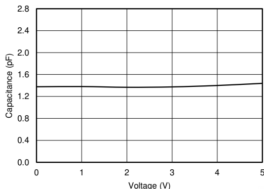
图 6-7. Capacitance Across V_{BIAS} f = 1\text{ MHz}
