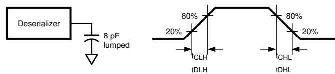
Figure 6. Deserializer LVCMOS Output Load and Transition Times
