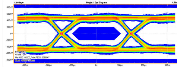
图 8-2. 3.4 Gbps HDMI 1.4 Eye Diagram in DCK Package
