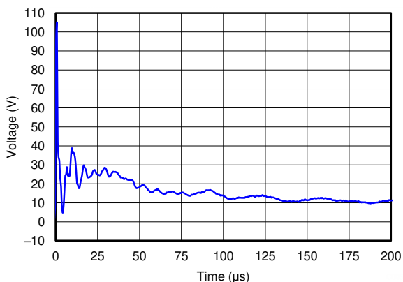
图 6-5. +8 kV IEC Waveform
