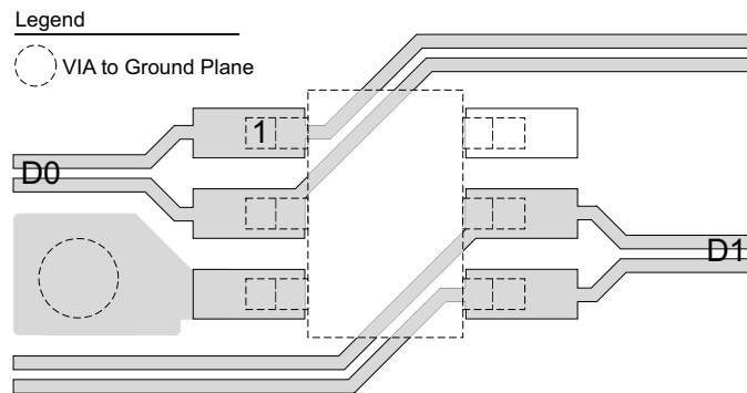
图 8-3. DCK Layout Example Showing Two Data Pairs, D0 and D1
