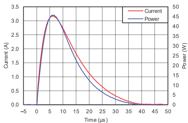
图 6-2. Surge Curve ( t_p = 8/20 \mu s ), Pin IO to GND
