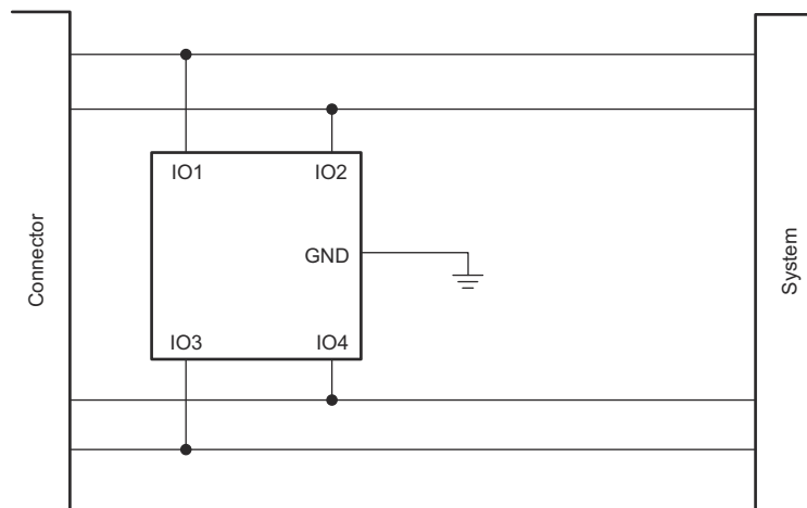
图 8-1. Protecting a Pair of Bi-Directional Differential Data Lines
