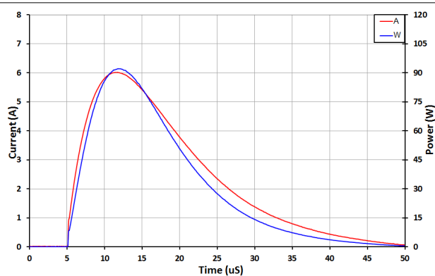
图 6-7. Negative Surge Waveform 8 to 20 \mu s
