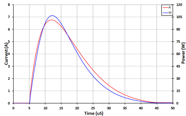
图 6-6. Positive Surge Waveform 8 to 20 μs
