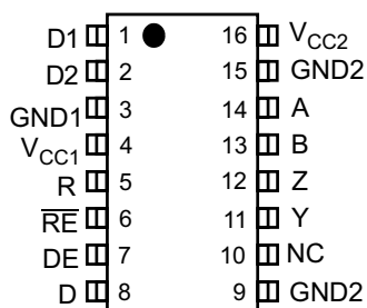
图 5-1. DW Package 16-Pin SOIC Top View
