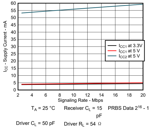
图 6-3. Supply Current vs Signaling Rate (With Load)
