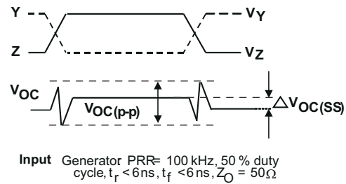
图 7-3. Test Circuit and Waveform Definitions For The Driver Common-Mode Output Voltage
