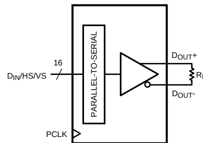
Figure 8. Serializer VOD DC Diagram
