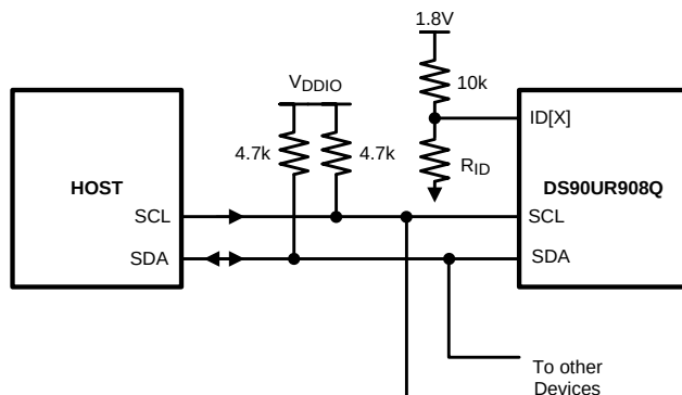
Figure 21. Serial Control Bus Connection
