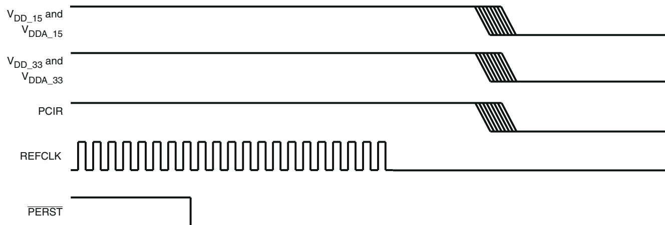
图 6-2. Power-Down Sequence
