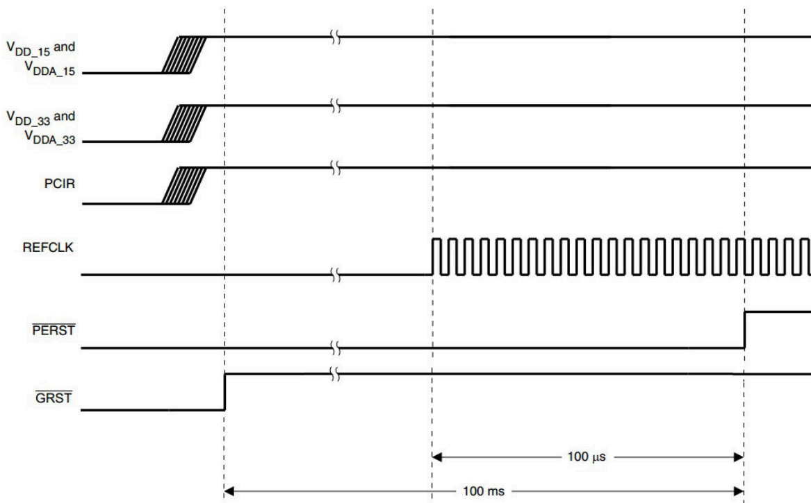
图 6-1. Power-Up Sequence
